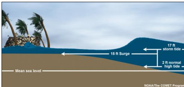
Figure 1. Storm Surge
