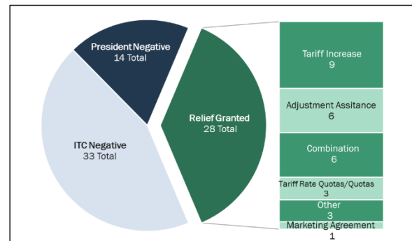
Figure 2. Section 201 Outcomes, 1975-2018
