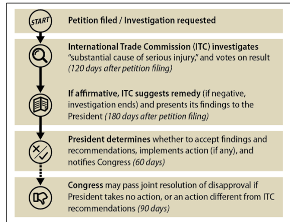
Figure 1. Section 201 Timeline
