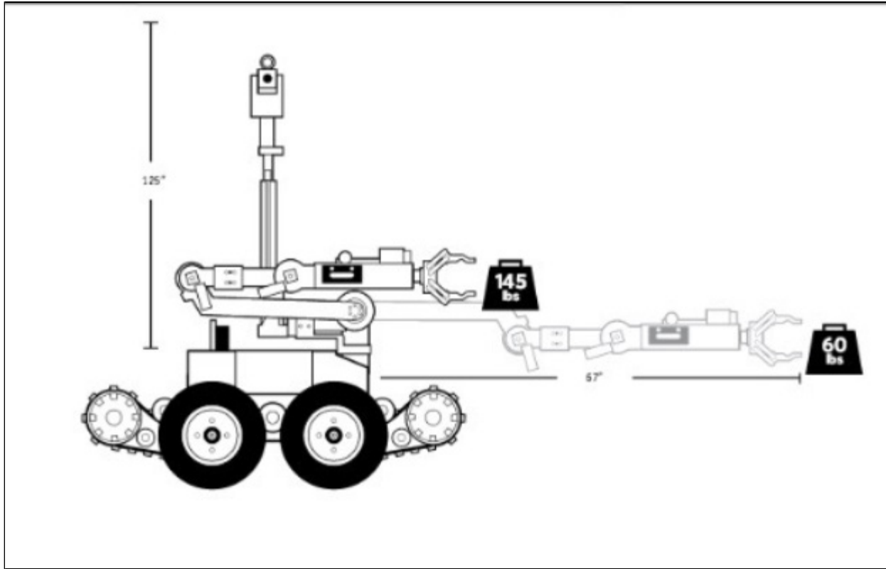
Figure 1. Remotec Andros Mark V-A1
