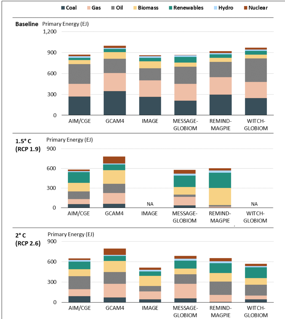
Figure 3. Global Primary Energy Mix in 2050, by IAM SSP2 (“middle-of-the-road” socioeconomic scenario)
