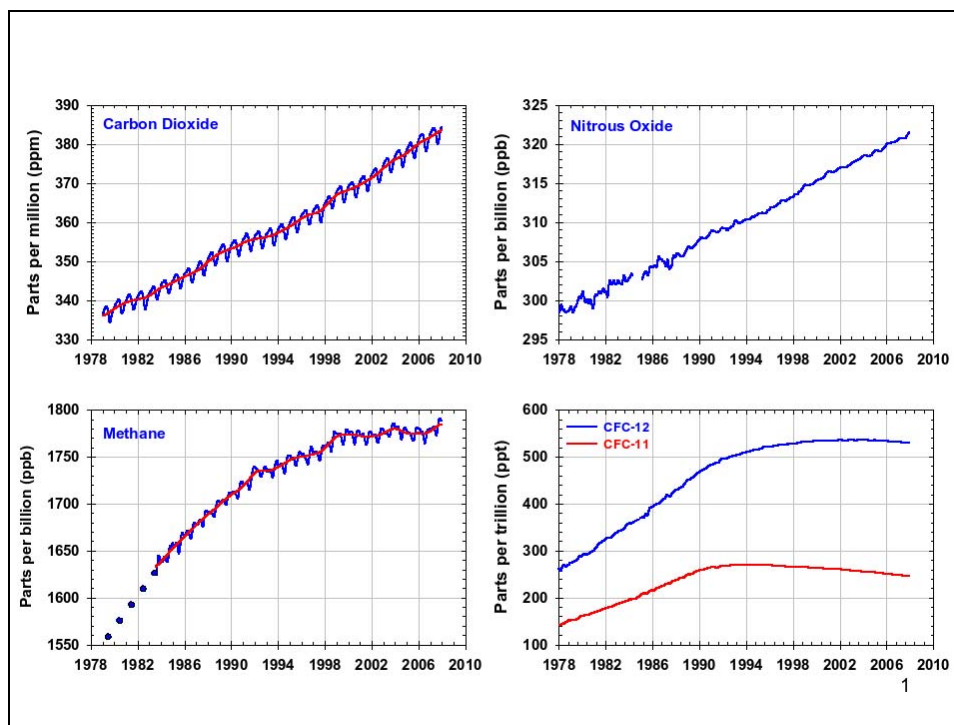
Figure 2. Global Average Atmospheric Concentrations of Five Major Greenhouse Gases
