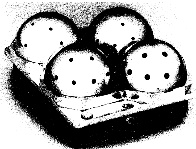
■ Figure 2. Four domes of the background instrument. Holes surrounded by thick material allow the flux to be sampled over a hemisphere at a counting rate that can be conveniently handled by the electronics. A hemispherical filter inside each dome defines an energy threshold for the particles entering the holes. Thus, four energy channels can be defined for the dose measured by the instrument.
