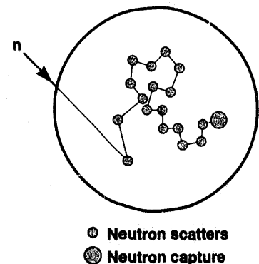
■ Figure 1. Schematic of the scatter-and-capture mechanism used in a boron-loaded scintillator to select only the neutrons that deposit all their energy in the detector. The proton-recoil pulses produced by the scattering of these neutrons provide the spectrum of their incident energies.
