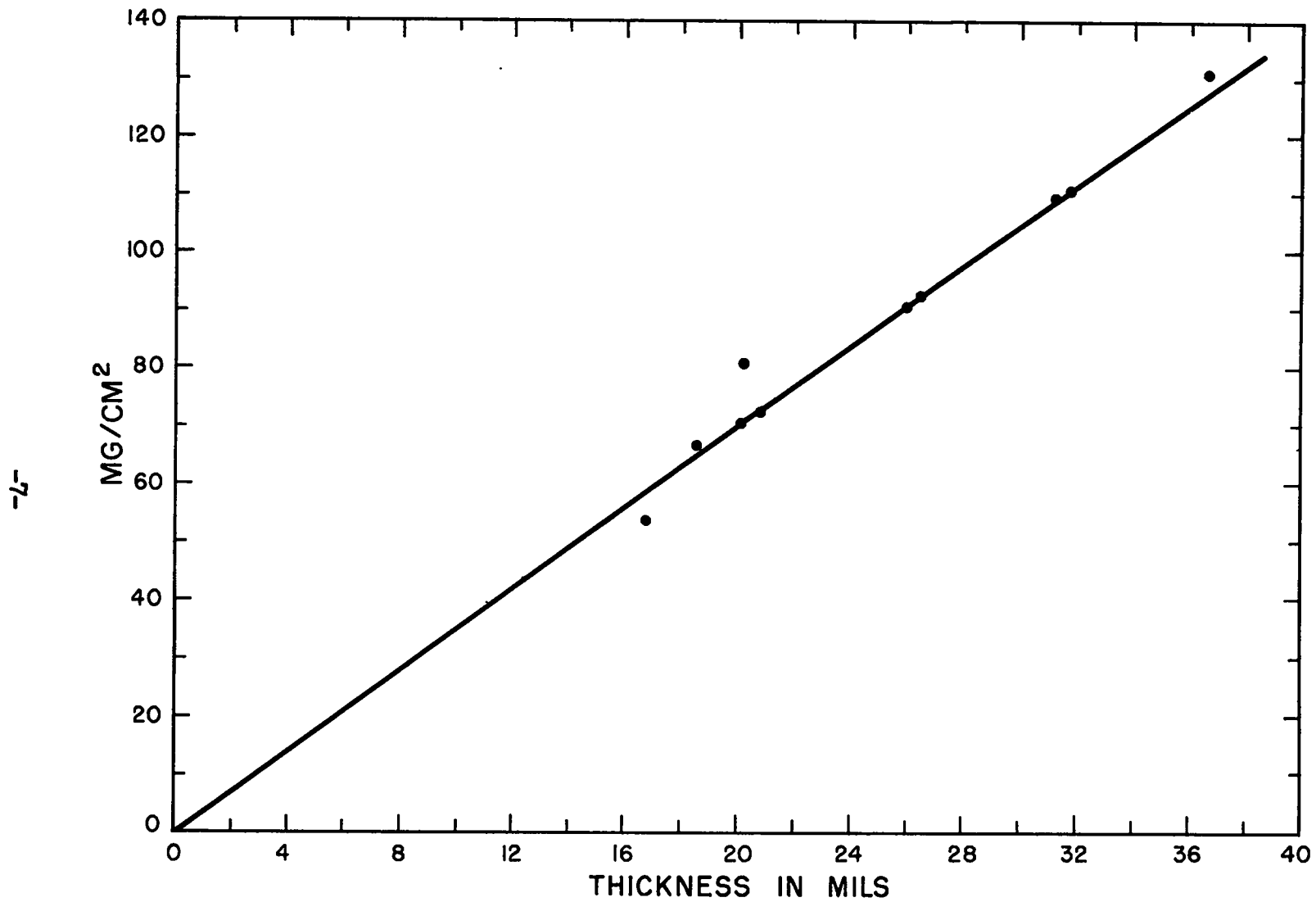
Fig. 2 - Correlation between weight per unit area and thickness in mils for dry-box glove neoprene.
