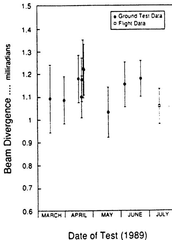
Fig. 5. Beam divergence history of the neutral beam.
