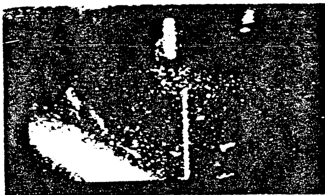
Fig. 6. Neutral beam (vertical line) propagating away from the spacecraft as viewed from an onboard wide-angle camera whose line of sight is almost parallel to the beam. The beam exits the accelerator at the bottom of the picture.
