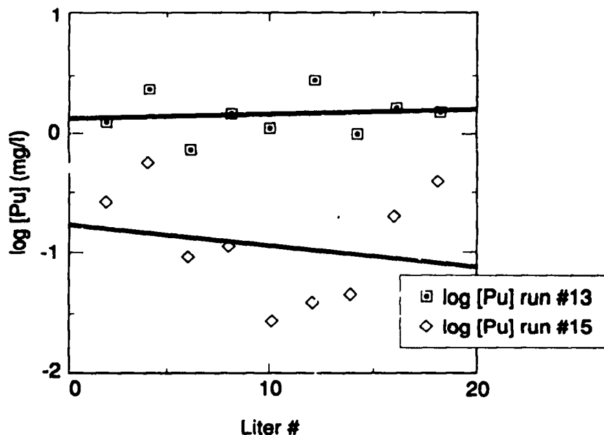
Fig. 4. Log [Pu] in Effluents vs Number of Liters of Wash
