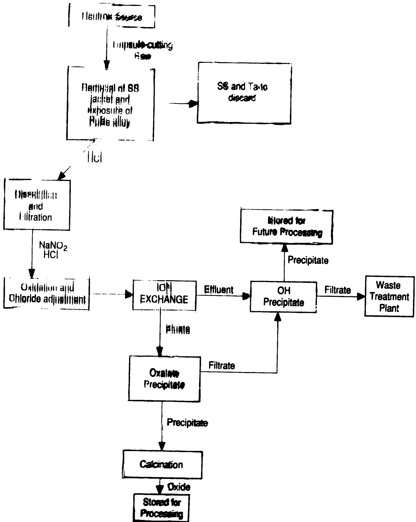
Fig. 1. Flow Diagram For Processing of PuBe Neutron Sources
