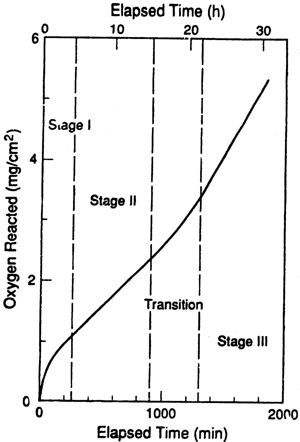
Figure 1. The stages of reaction observed for oxidation of plutonium metal. The curve is based on data for the Pu+O 2 reaction at 300°C and 1 torr O 2 pressure. 10
