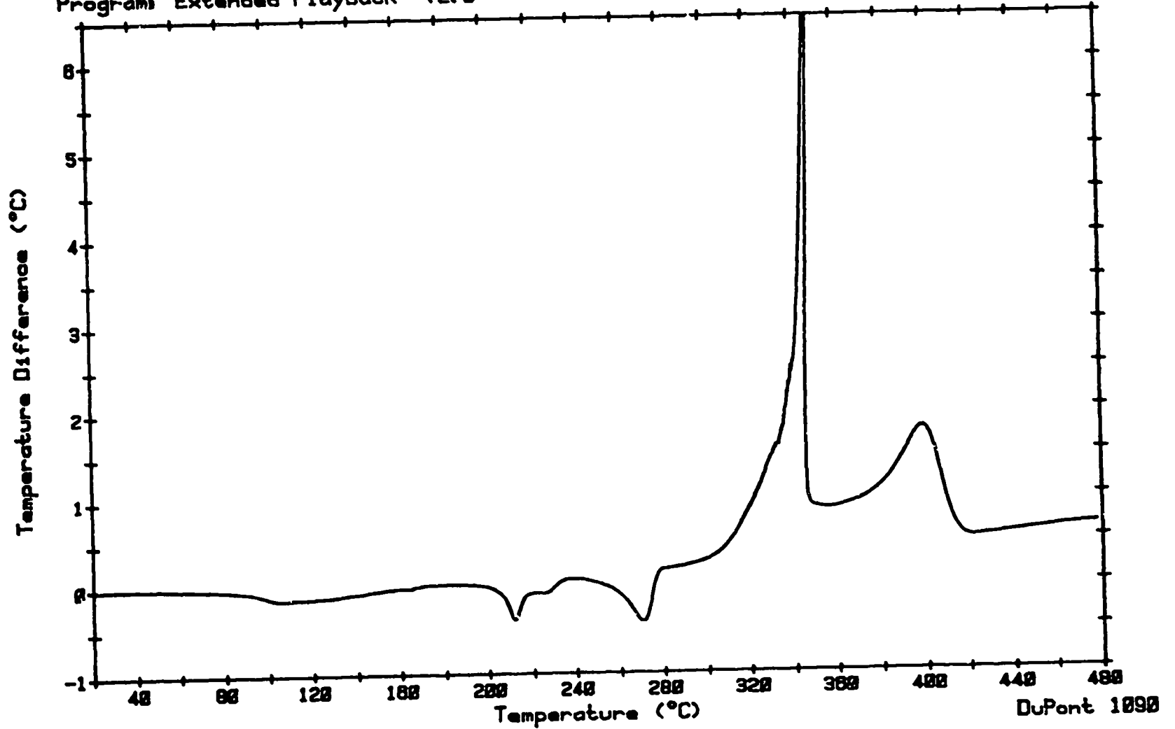
Figure A-10. VENDOR MIX#1, as received, macro, 5°C/min.
