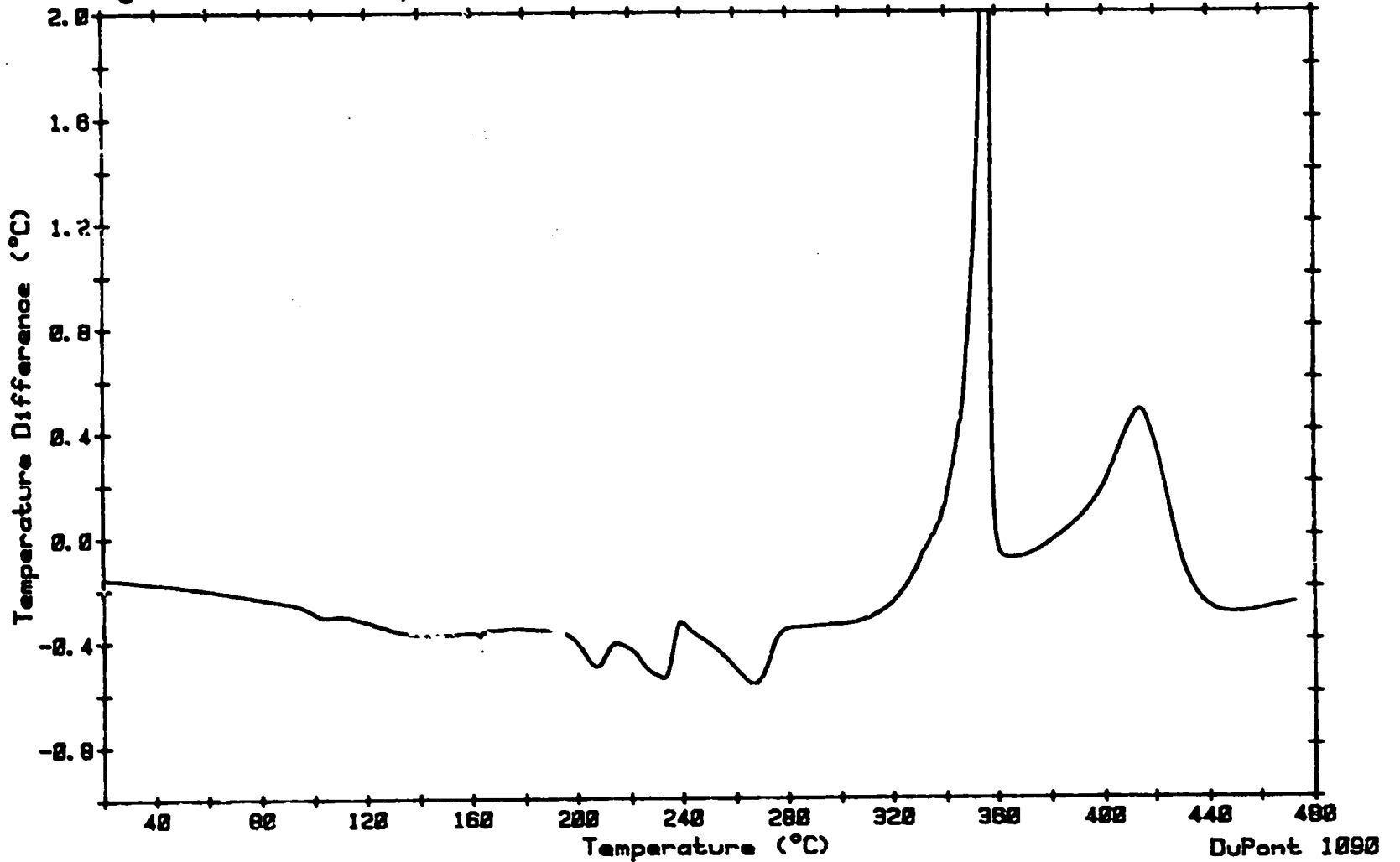
Figure A-19. VENDOR MIX#1, as received, micro, 10°C/min.
