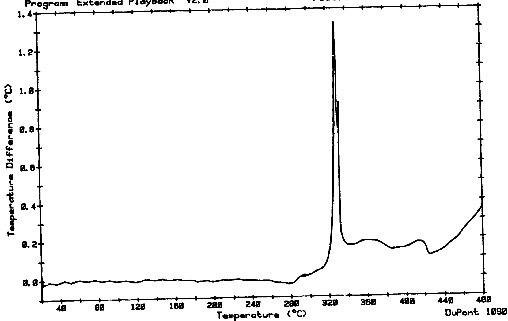
Figure A-14. INFARM1-REV-23, dry, micro, 2°C/min.
