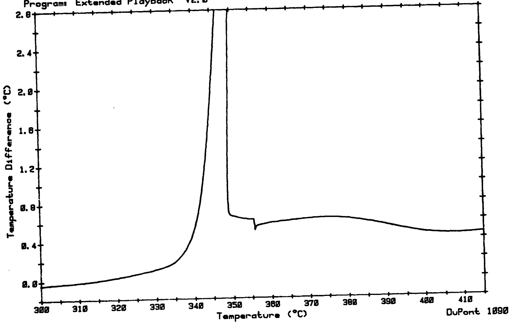
Figure A-23. INFARM1-REV-23, dry, micro, 5°C/min.
