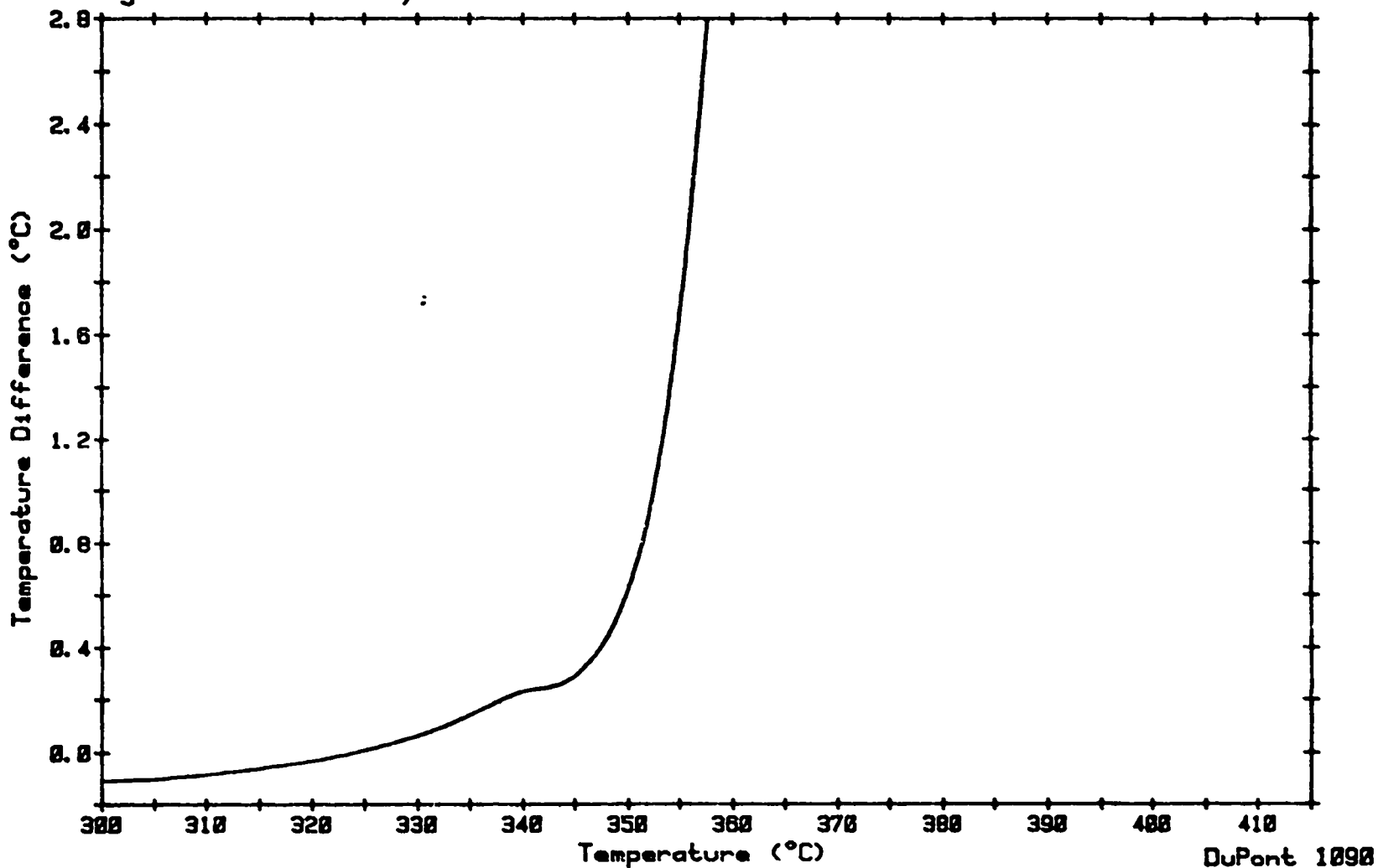
Figure A-22. INFARM1-REV-23, dry, micro, 10°C/min.
