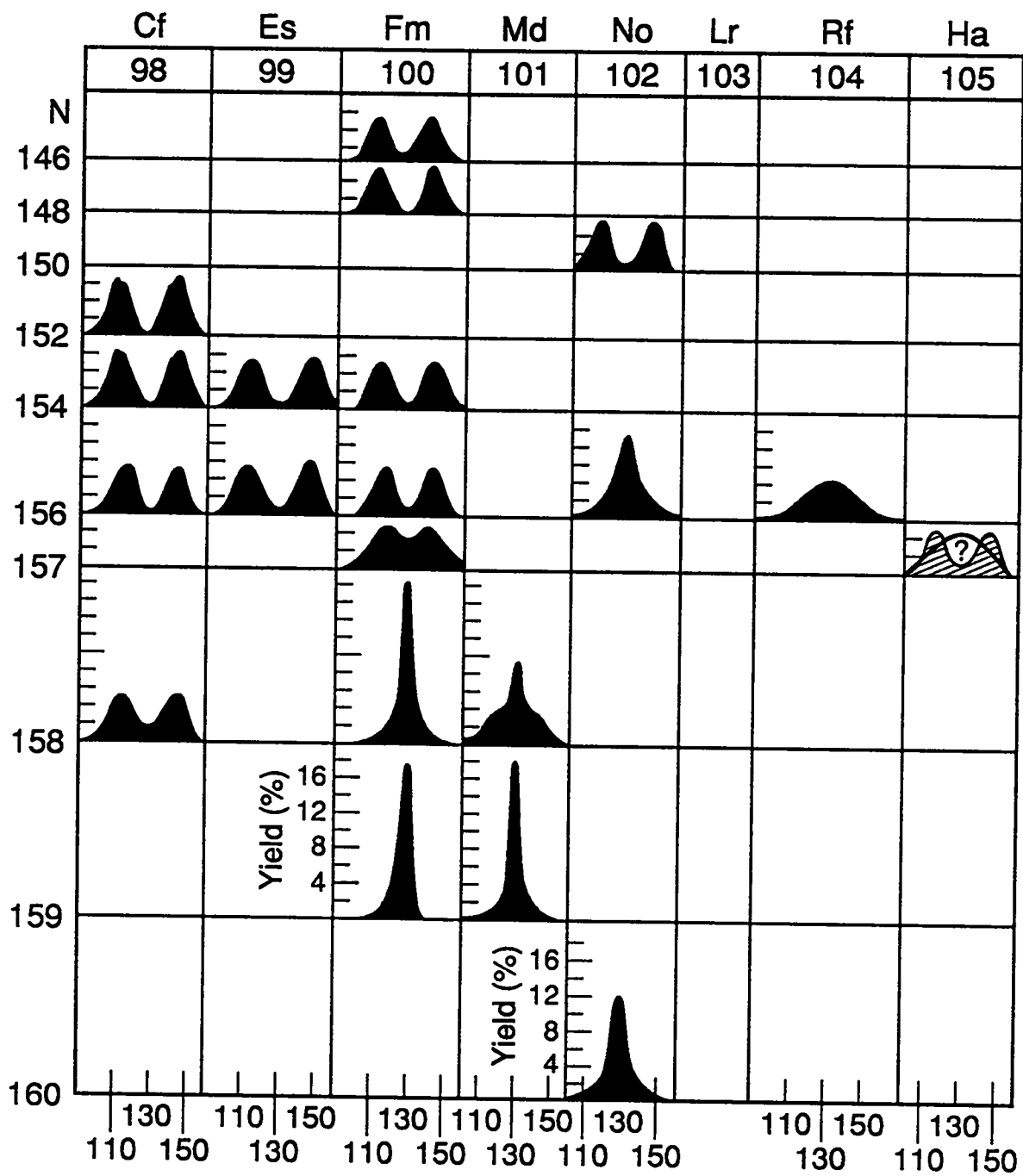
Mass Yield Curves for Spontaneous Fission
