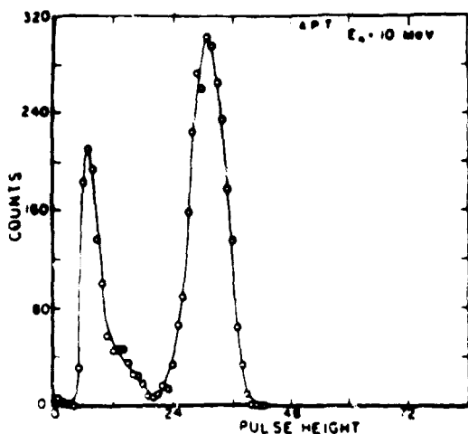
Fig. 3. Pulse height distribution observed with the APT for a neutron energy of 10 MeV.
