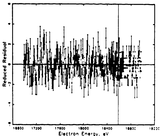
Fig. 3. Residual plot for Run 4-B with m_\nu=0 .
