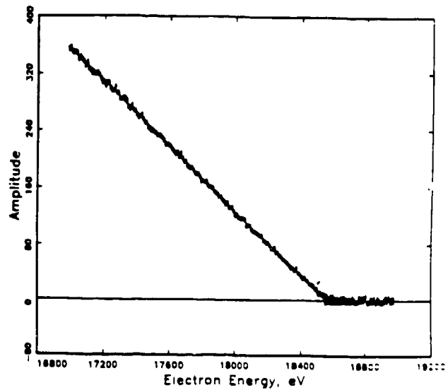
Fig. 2. Kurie Plot for Run 4-B.
