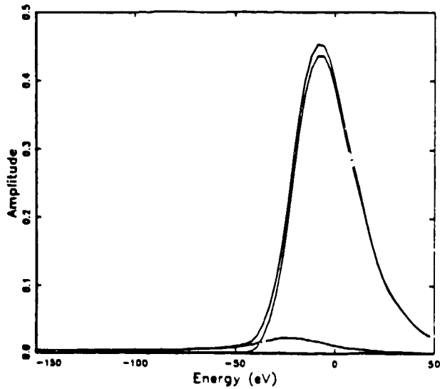
Fig. 1. Resolution function for Run 4-B showing optical resolution, energy loss component and sum of both.
