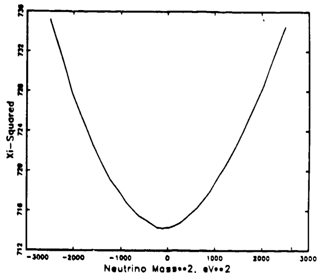
Fig. 4. \chi^2 plot for all three runs.
