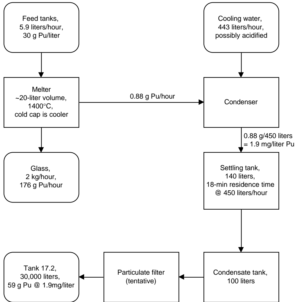
Fig. 1. Schematic of the planned vitrification system at the Savannah River Site.
