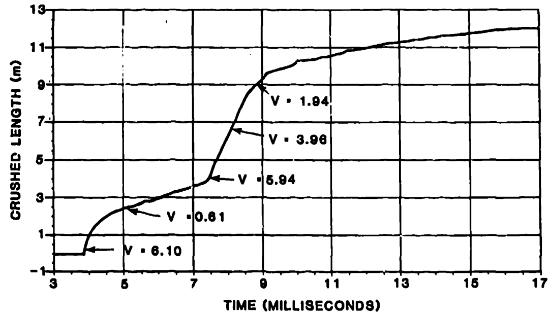
Figure 10. Explosive evaluation test using SLIFEX.
