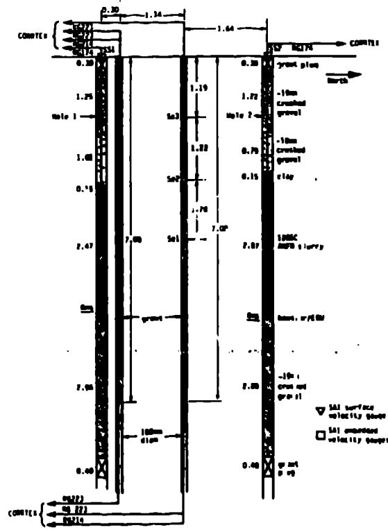
Figure 7. Installation of COBTEX sensor cables in a fragmentation test.
