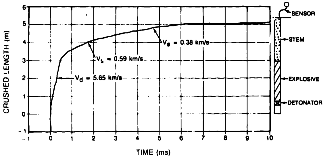
Figure 8. Idealized signal record from COBTEX or SLIFER showing explosive detonation and shock wave propagation the stem column.
