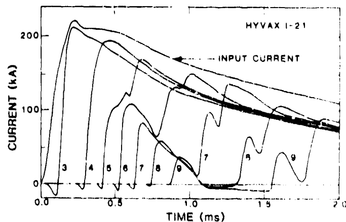
Fig. 2 Magnetic probe signals for HYVAX test I-21
