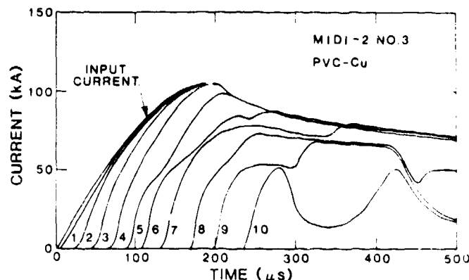
Fig. 7 Rail current probe data from MIDI-2 test #3
