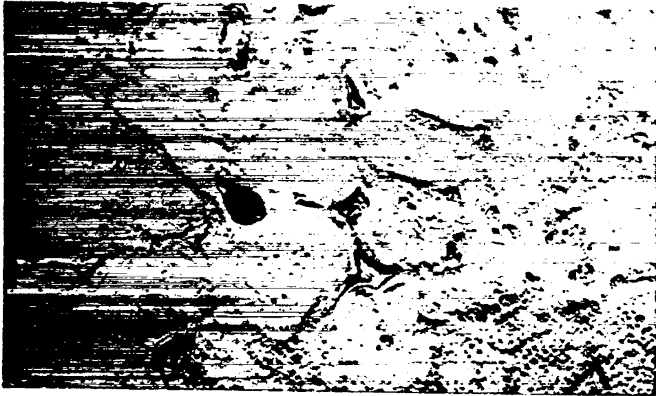
Figure 28. Microstructure of rolled relatively impure 1 w/o gallium-stabilized delta plutonium. 500 X
