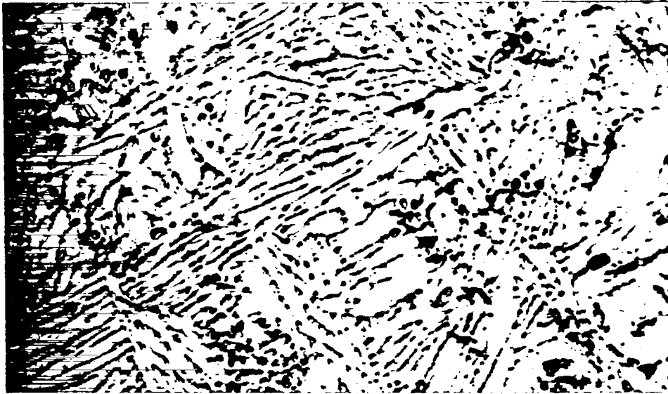
Figure 41. Microstructure of cast 1 w/o gallium-stabilized delta plutonium annealed for 250 hours at 625°C. 500 X
