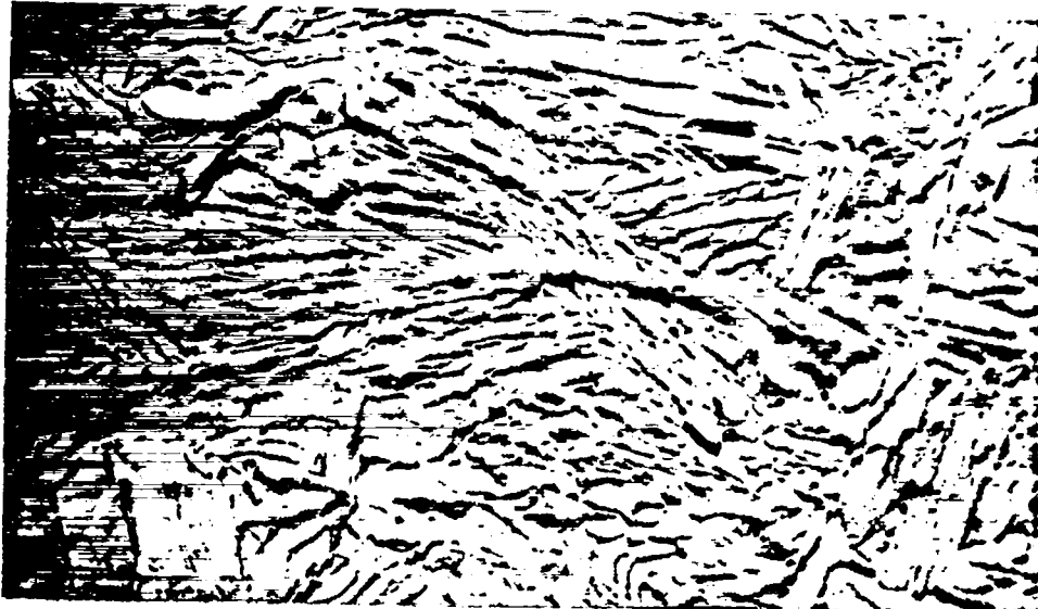
Figure 36. Microstructure of cast 1 w/o gallium-stabilized delta plutonium annealed for 4 hours at 625°C. 500 X
