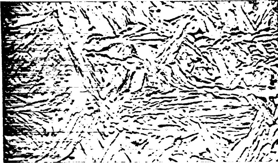
Figure 37. Microstructure of cast 1 w/o gallium-stabilized delta plutonium annealed for 16 hours at 625°C. 500 X
