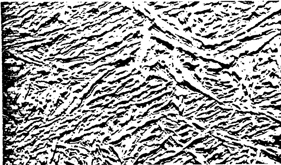
Figure 38. Microstructure of cast 1 w/o gallium-stabilized delta plutonium annealed for 24 hours at 625°C. 500 X
