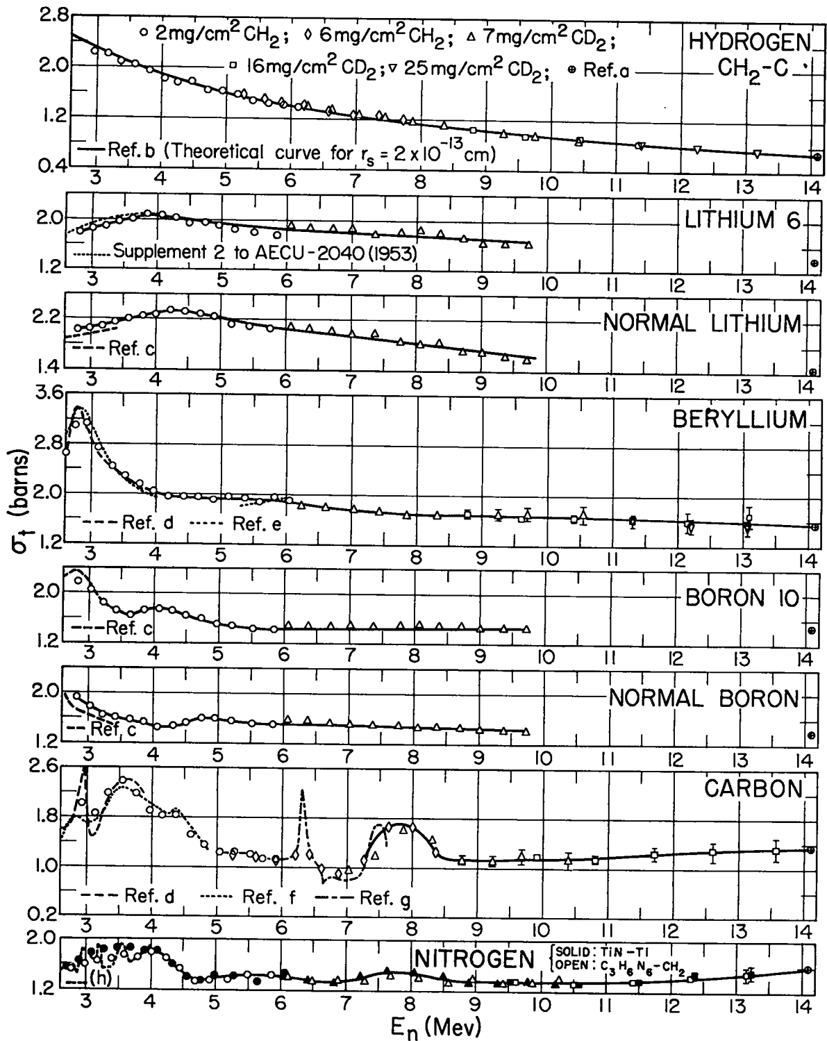
Fig. 4 Average total neutron cross sections of H, Li 6 , Li, Be, B 10 , B, C, and N
