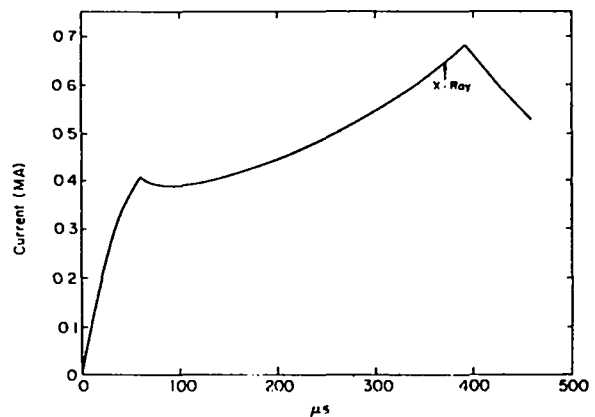
Fig. 4. Current vs time for a simulated rail gun load. A flash x-radiograph was taken at the generator-load junction shortly before generator burnout.
