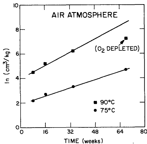
Fig. 3. Rate constant plot.
