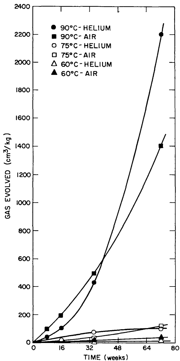
Fig. 1. Gas evolved from X-0298 small cylinders stored in sealed containers.
