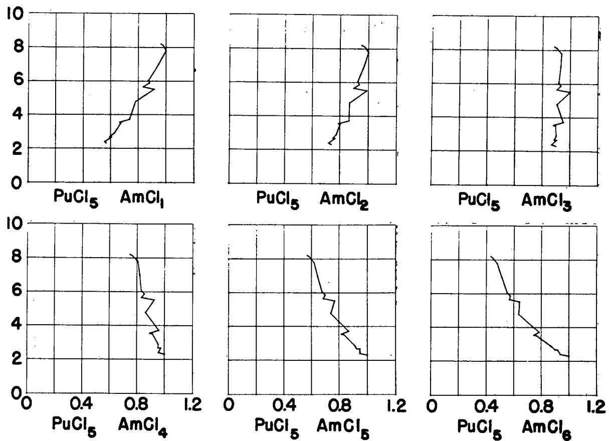
Fig. 6. K'/K'_{\text{max}} (x axis) vs. wt. % Pu in Salt (y axis), 730^{\circ}\text{C} ., for the Stoichiometry \text{PuCl}_5 and \text{AmCl}_1 through \text{AmCl}_6
