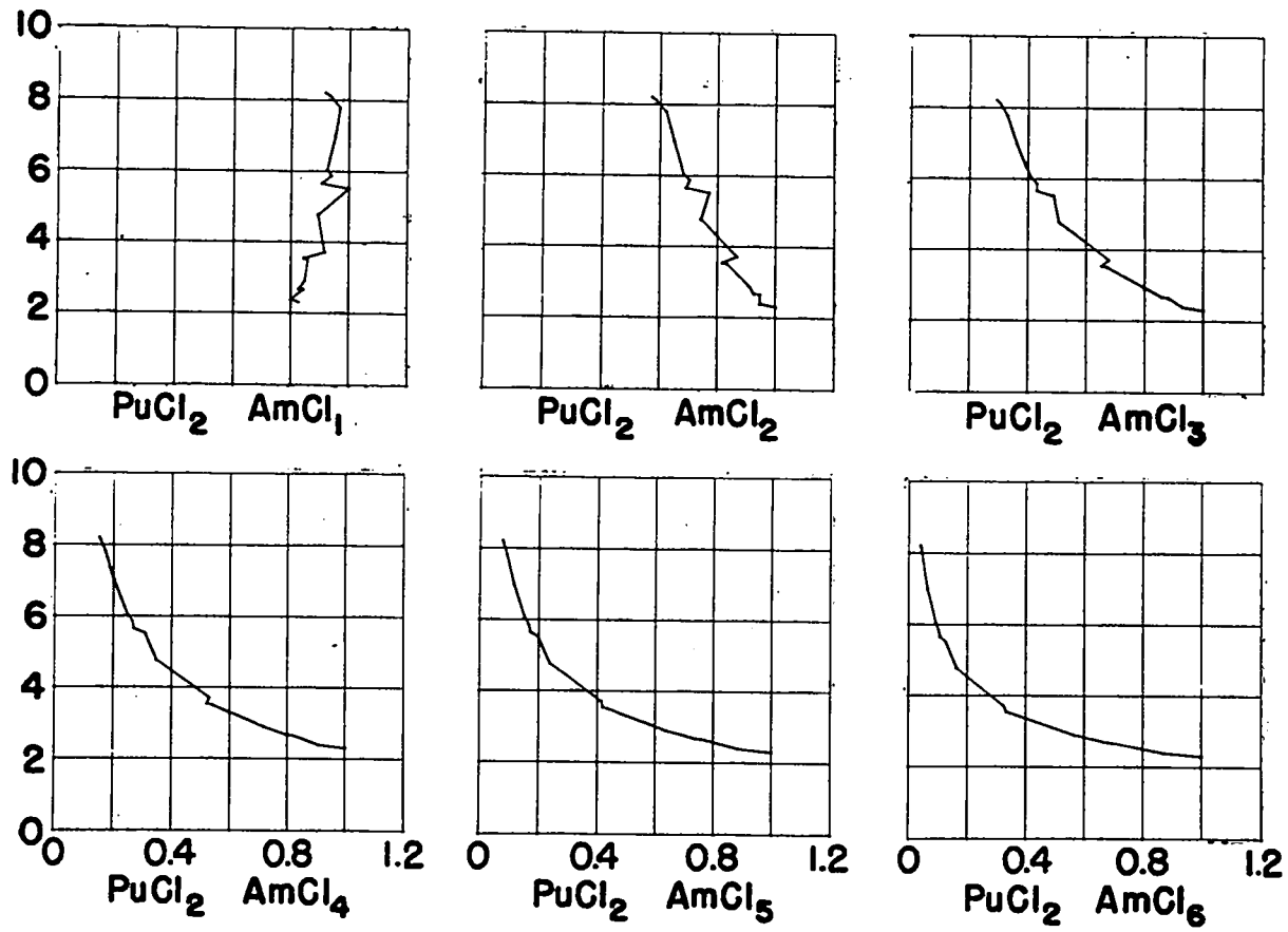
Fig. 3. K'/K'_{max} (x axis) vs. wt. % Pu in Salt (y axis), 730°C., for the Stoichiometry PuCl 2 and AmCl 1 through AmCl 6
