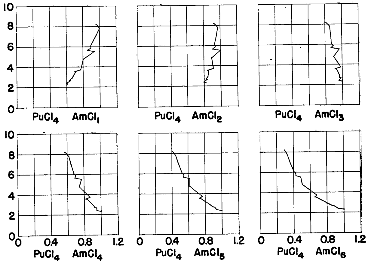
Fig. 5. K'/K'_{max} (x axis) vs. wt. % Pu in Salt (y axis), 730^{\circ}C. , for the Stoichiometry PuCl_4 and AmCl_1 through AmCl_6
