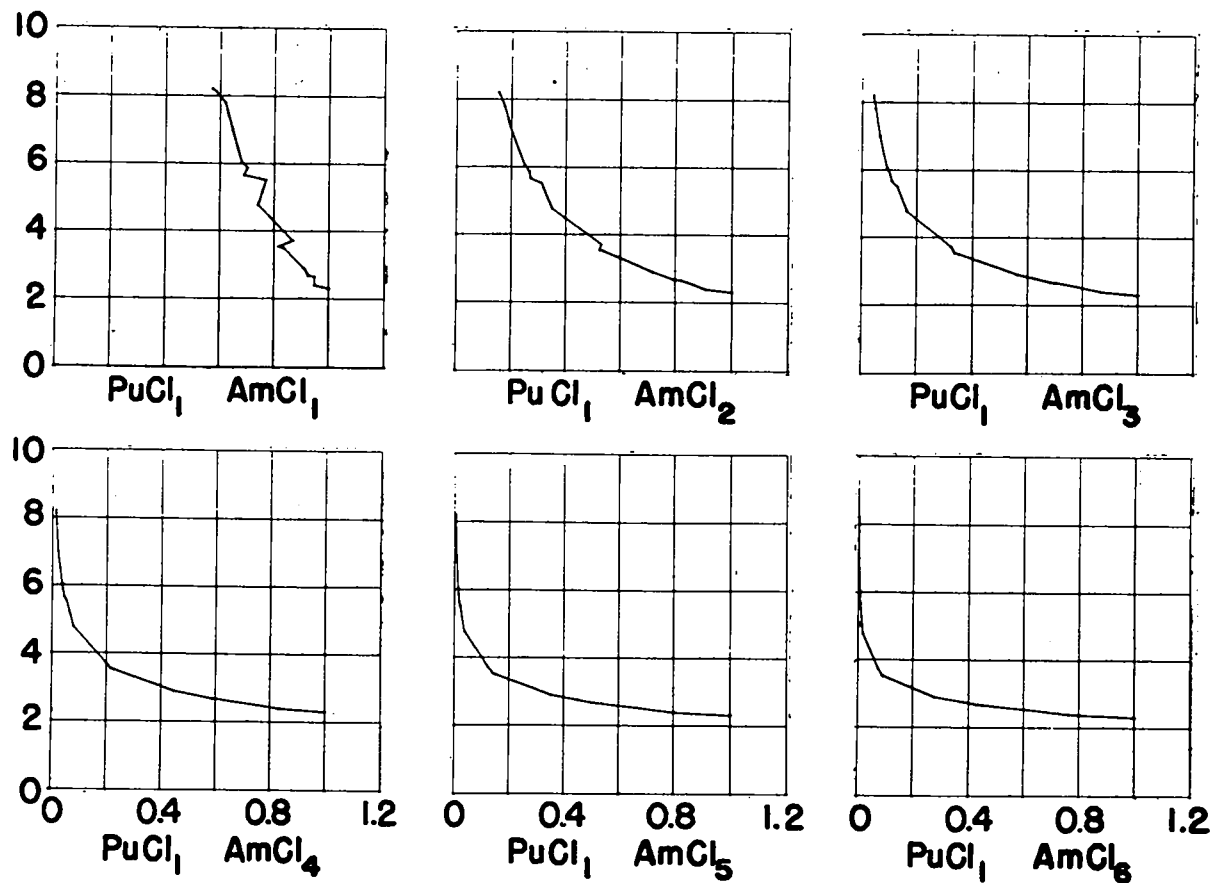
Fig. 2. K'/K'_{\max} (x axis) vs. wt. % Pu in Salt (y axis), 730^\circ\text{C} ., for the Stoichiometry \text{PuCl}_1 and \text{AmCl}_1 through \text{AmCl}_6
