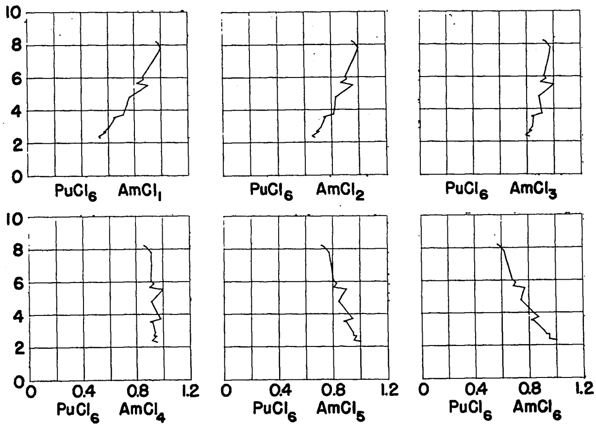
Fig. 7. K'/K'_{max} (x axis) vs. wt. % Pu in Salt (y axis), 730^{\circ}C. , for the Stoichiometry PuCl_6 and AmCl_1 through AmCl_6
