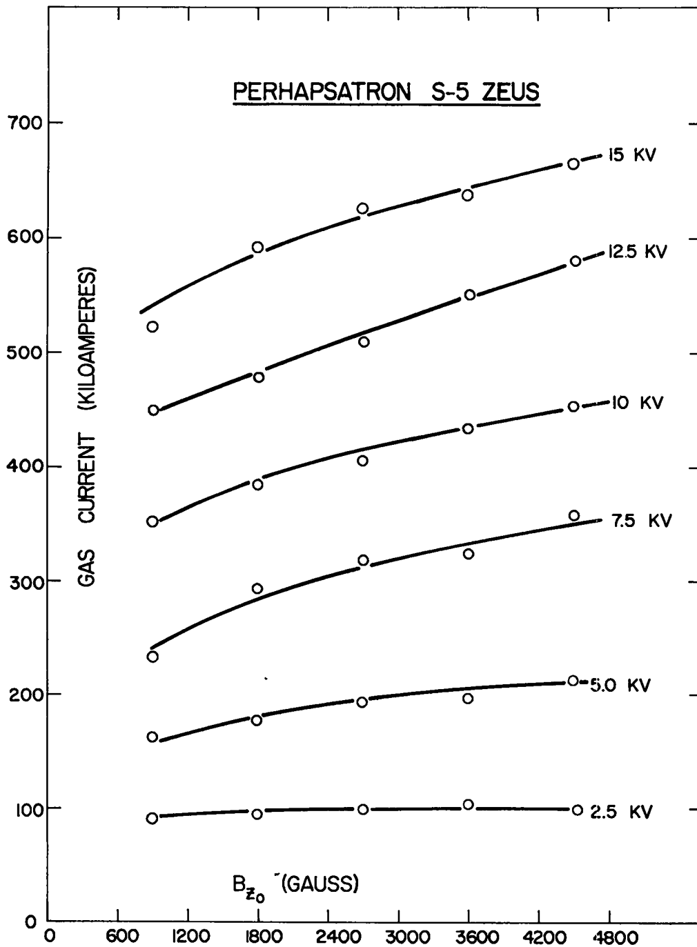
Fig. 12. Discharge current in Perhapsatron S-5-Zeus as function of B_0 for various bank voltages.
