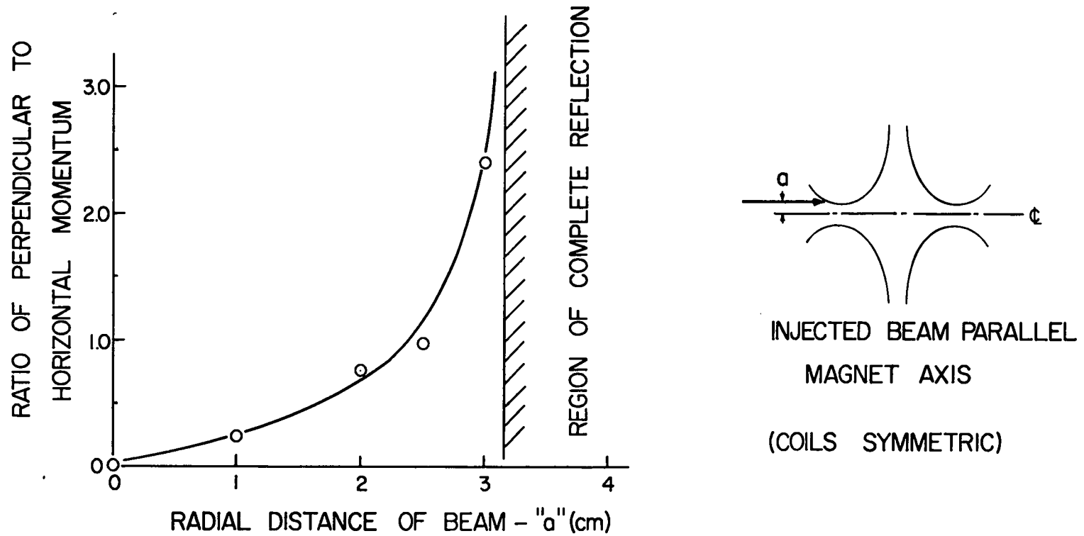
Fig. 3. Movement of momentum (perpendicular to horizontal) ratio in symmetric magnetic field.
