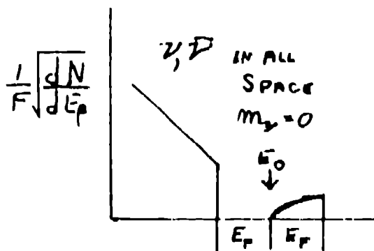
Fig. 3a Kurie Plot, No Clustering
