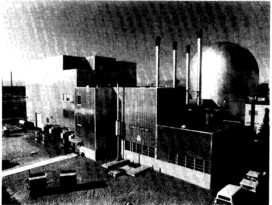
Fig. 13. The EBR-II reactor is located at Idaho National Engineering Laboratory near Idaho Falls, Idaho. This liquid-metal-cooled fast breeder reactor has operated successfully for over 15 years. The reactor produces up to 20 megawatts of electrical energy and has had an excellent history of reliable operation. A predecessor of EBR-II, a small reactor called EBR-I, produced the first nuclear-generated electricity in 1951. (Photo courtesy of Argonne National Laboratory.)
