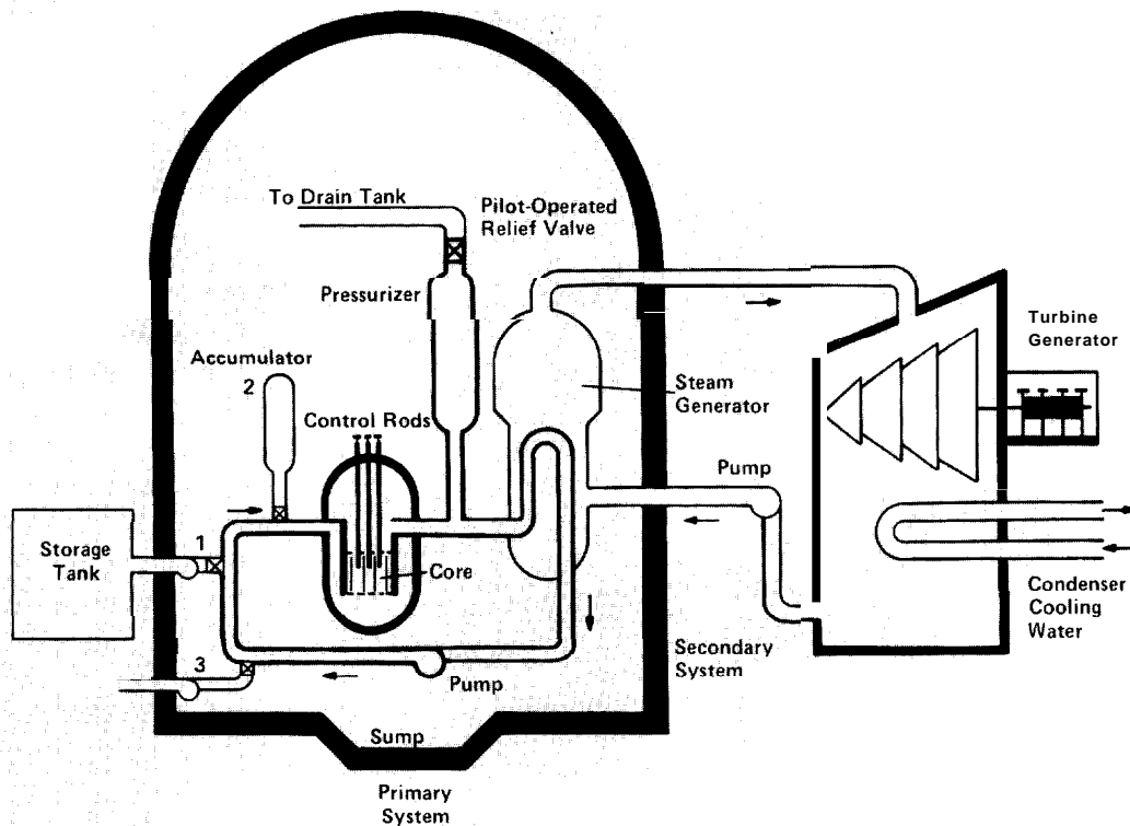
Fig. 5. A pressurized-water reactor showing a primary loop, a secondary loop, and the three subsystems (labeled 1, 2, and 3) of the emergency core-cooling system. In the primary system, water under high pressure (about 150 bars) is pumped by
