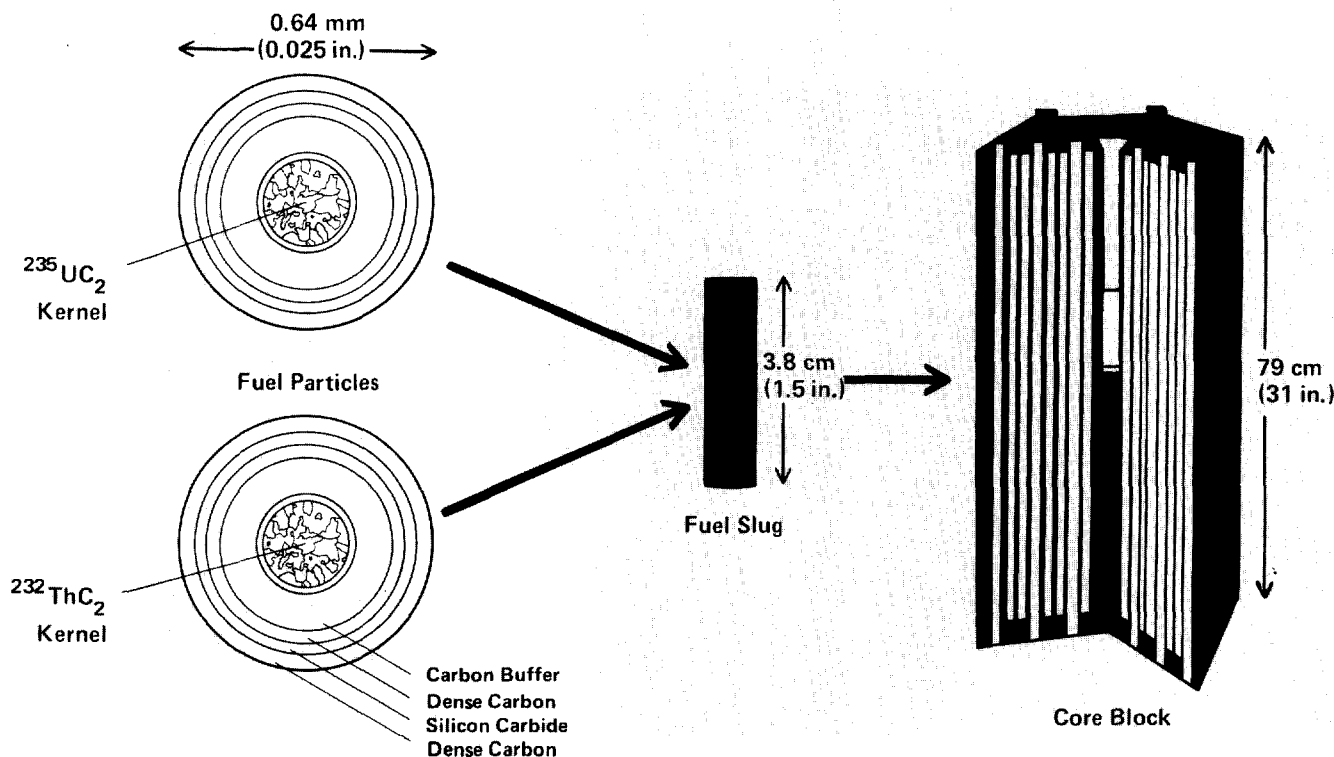
Fig. 15. Fuel for the high-temperature gas-cooled reactor is in the form of small particles containing a kernel of either fissile uranium-235 or fertile thorium-232, both as dicarbides. Typically, three barrier coatings plus an inner buffer zone encase the kernel and serve to contain the fission products. The
