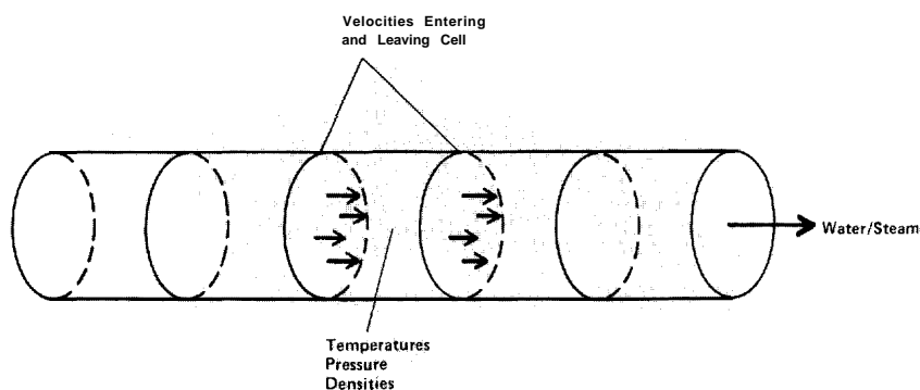
Fig. 10. Division of a coolant pipe into computational cells. Densities, pressures, and temperatures at the center of each cell are computed, as well as the velocities of the steam-water mixtures entering and leaving each cell.
