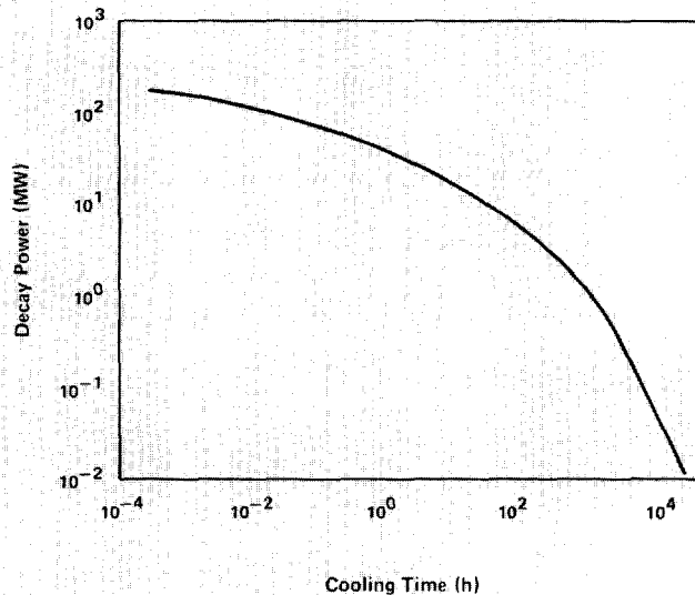
Fig. 7. A log-log plot of decay power as a function of time after reactor scram for the Three Mile Island Unit 2 reactor. This curve was calculated by the Laboratory Nuclear Data Group. It depends on the reactor's power history and fuel and fission-product inventories and on details of the decay chains that fission products and transuranics follow as they spontaneously decay to more stable nuclear states.
