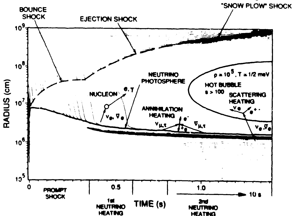
Figure 2. The sequence of processes occurring in a Type II supernova according to Wilson and Mayle. (1989). First a star collapses, owing to exhaustion of the fuel and emits electron neutrinos as the compressing matter turns into neutron-rich matter. The forming neutron star bounces producing a strong shock that weakens owing both to the thermal decomposition of the infalling nuclear matter and the reversal of the neutron star bounce trajectory. Subsequently, a large burst of neutrinos of all flavors heats the infalling matter, starting an explosive shock. Yet later, mu and tau neutrino-antineutrino annihilations in nearly opposed collisions just above the neutrino photosphere generate heat without nucleonic matter, making a hot, high-entropy ( 10^4 Boltzmann-units) bubble, which pushes out the ejected matter in a thin "snow plow" shock. The pressure is maintained because the high-entropy ensures a large scale height adjacent to the neutron star.
