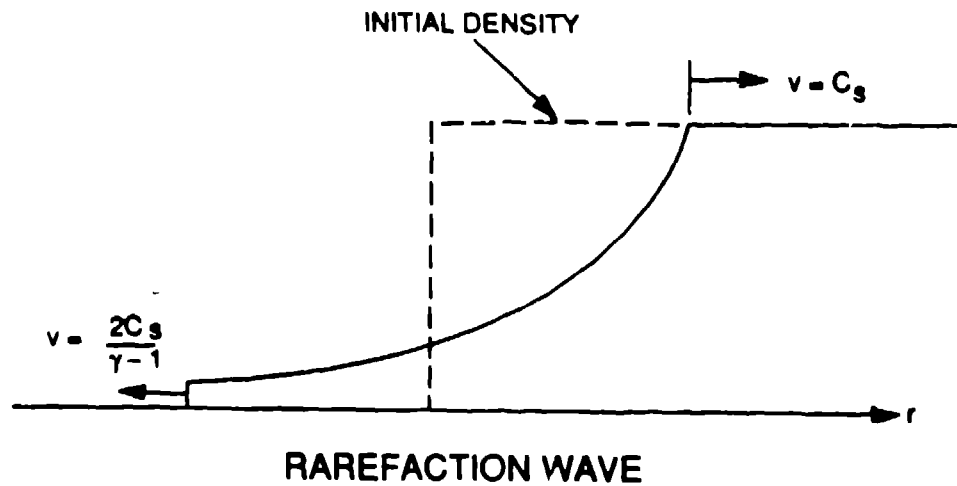
Figure 1 shows the classical rarefaction wave that progresses within the fluid at sound speed and reverses the flow. The maximum velocity of blow off from a rarefaction wave is 2C_s/(\gamma-1) .
