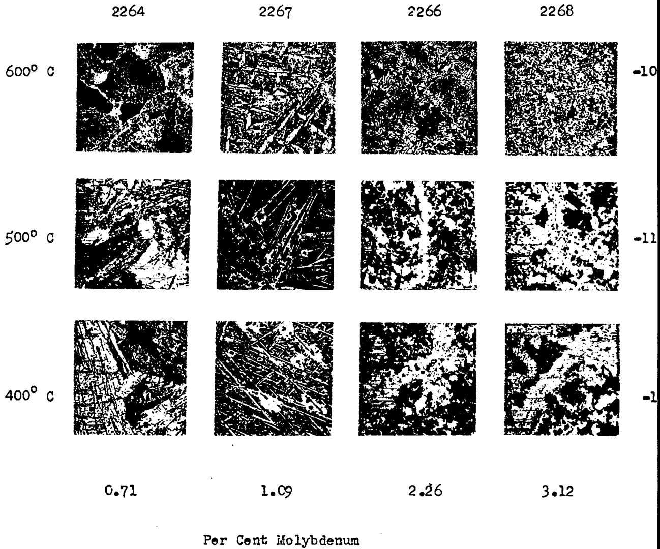
Fig. 2 Microstructure of the Long Time Heat Treated Alloys x 250
