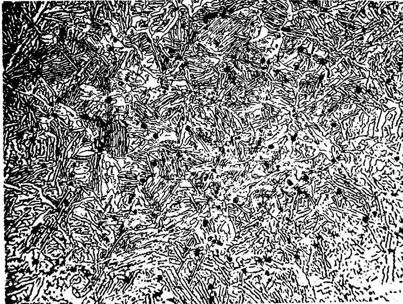
Figure 3 : Structure of a 2.0 percent Mo-U alloy. Quenched after 24 hrs. at 675° C. Etched in 2 percent oxalic acid
