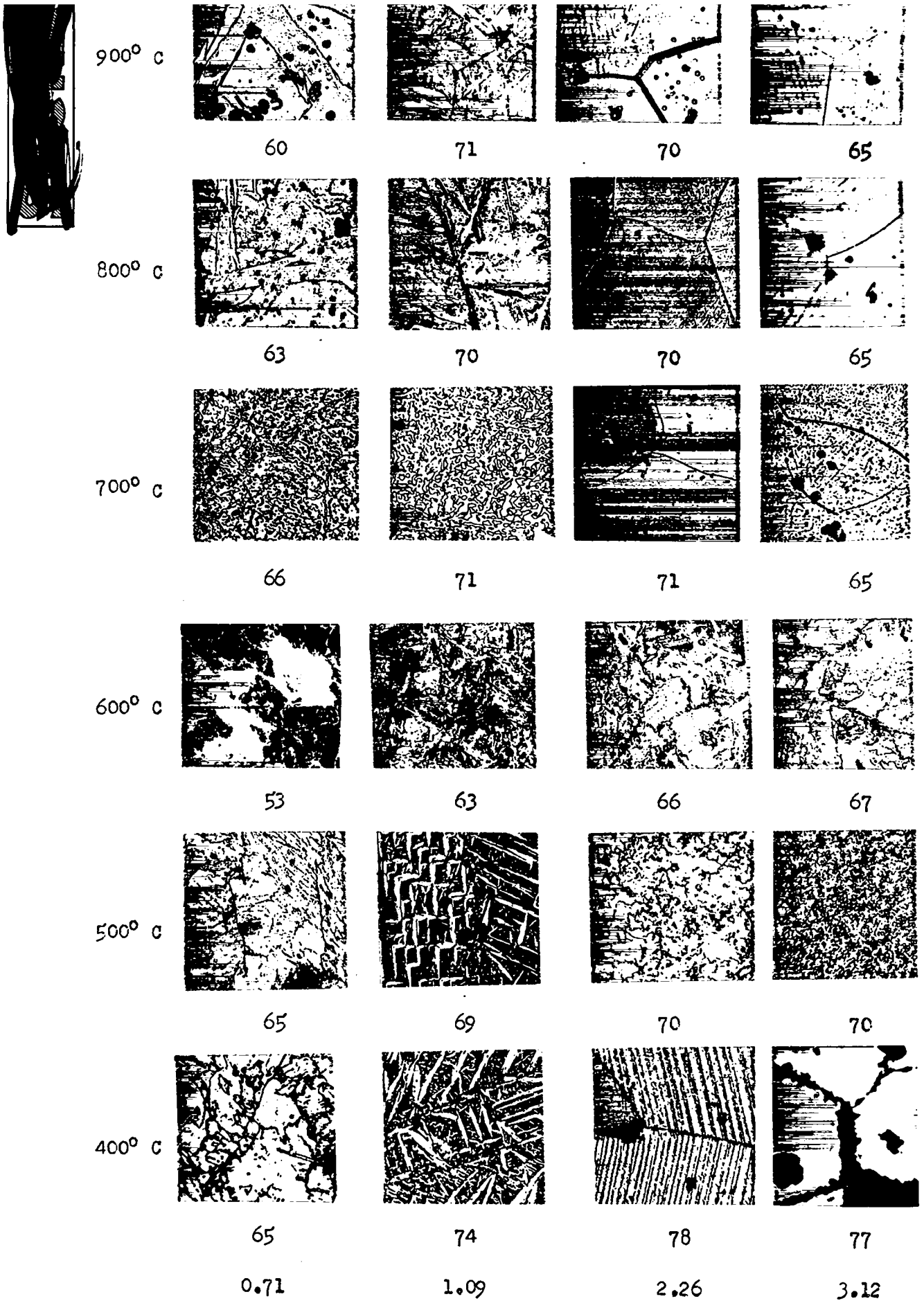
Fig. 1. Microstructures of Heat Treated Alloys x 250
