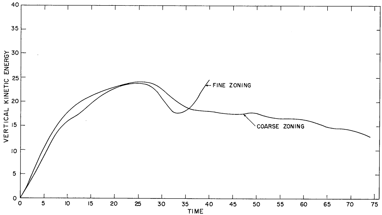
Fig. 13 Vertical kinetic energy of one basic section of the slab, shown as a function of time, for the calculations shown in Figs. 9 and 10.
