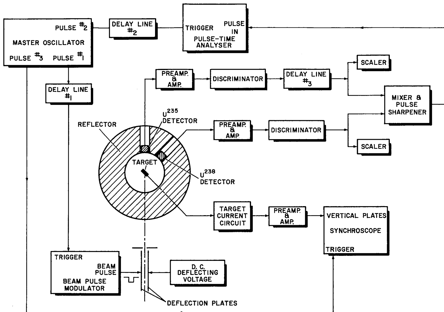
Figure 2. Detection system
