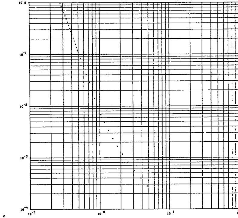
ANATOL WITH AN 19 O/O REACTED PRESSURE-VOLUME ISENTROPE THRU THE C-J VALUE
