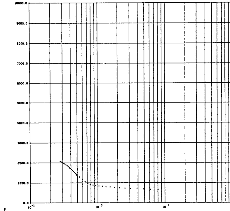
ANATOL WITH AN 19 O/O REACTED TEMPERATURE-VOLUME ISENTROPE THRU THE C-J VALUE
