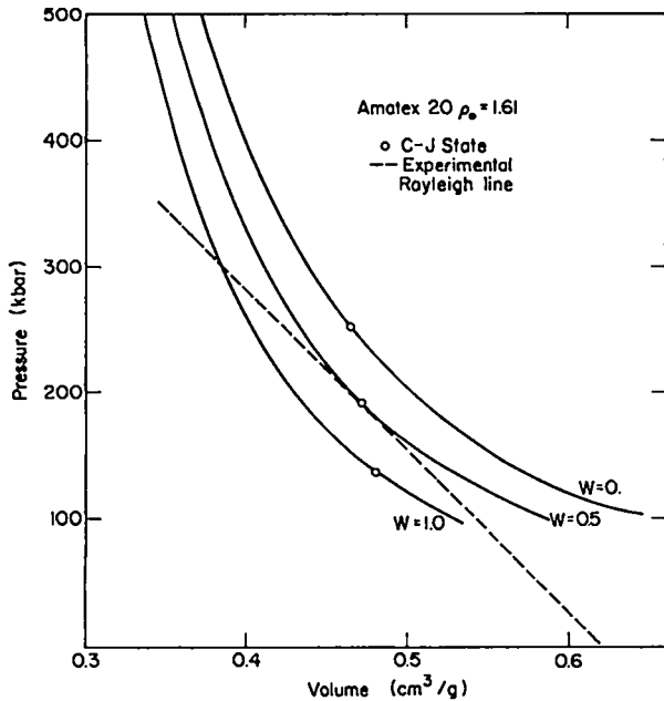
Fig. 4. The BKW calculated Hugoniot for Amatex 20 for W_{AN} = 0, 0.5, \text{ and } 1.0 .
