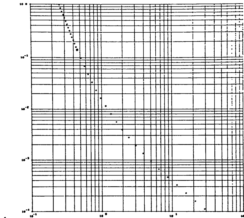
FIGURE WITH MARK = 0.37 PRESSURE-VOLUME ISENTROPE FROM THE C-J VALUE
