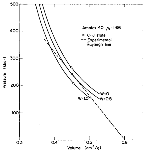
Fig. 3. The BKW calculated Hugoniot for Amatex 40 for W_{\text{AN}} = 0, 0.5, \text{ and } 1.0 .
