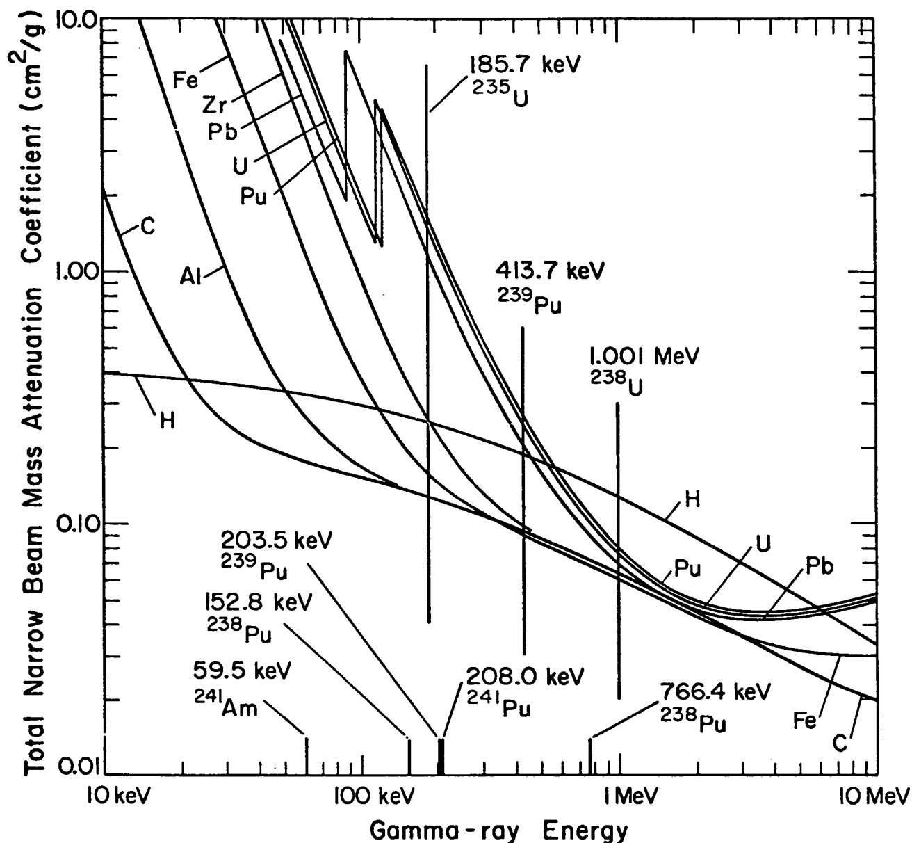
Fig. 1.10. Mass absorption coefficients for selected elements.
