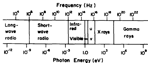
Fig. 1.1. The electromagnetic spectrum.
