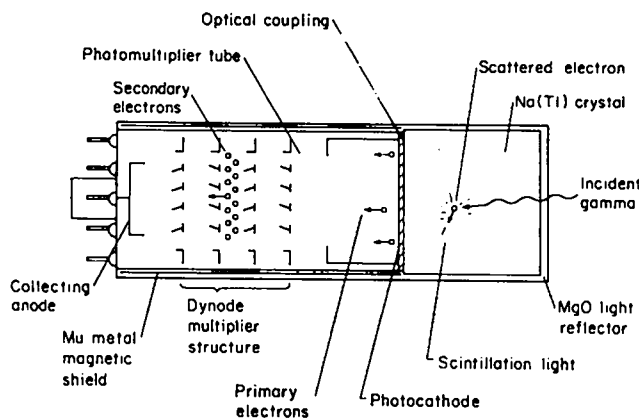
Fig. 2.7. The scintillation detector.
