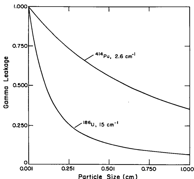
Fig. 5.4. Self-attenuation vs particle size.
