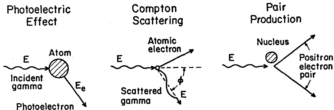
Fig. 1.5. Representation of major gamma-ray interaction processes.
