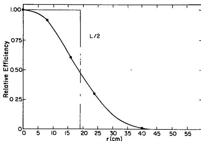
Fig. 5.9. Relative detection efficiency vs lateral distance from detector centerline.
