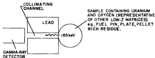
Fig. 6.1. Schematic illustration of uranium enrichment measurement.
