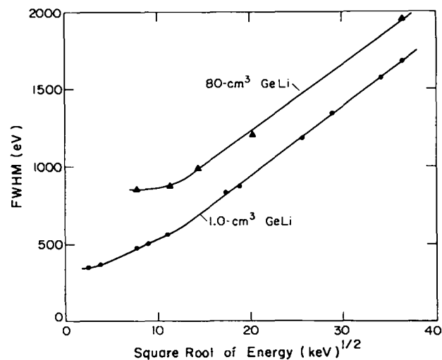
Fig. 3.2. Resolution vs energy for two Ge(Li) detectors.
