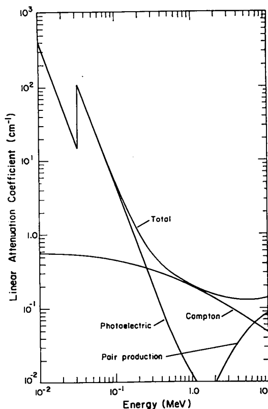
Fig. 1.9. Linear absorption coefficient for NaI showing contributions from photoelectric effect, Compton scattering, and pair production. Note the use of log-log scales. (Data from NBS Circular 583 after "Harshaw Scintillation Phosphors," Harshaw Chemical Company.)
