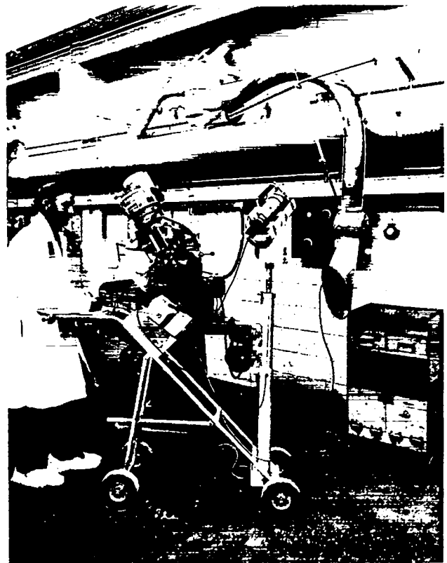
Fig. 5.7. Measurement of uranium holdup in a duct using cart-mounted NaI and SAM-1.
