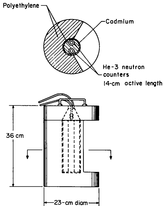
Fig. 8.5. Assembly drawing of the portable shielded neutron assay probe (SNAP).
