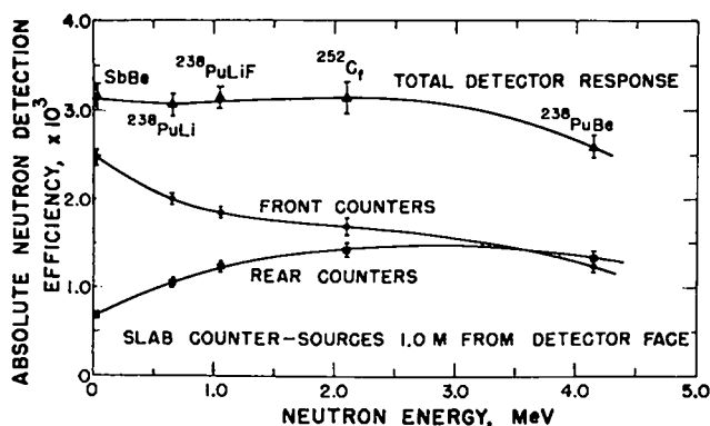
Fig. 8.4. High efficiency slab neutron detector.
