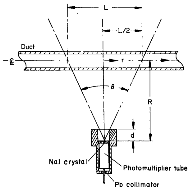
Fig. 5.8. Diagram of duct measurement geometry.
