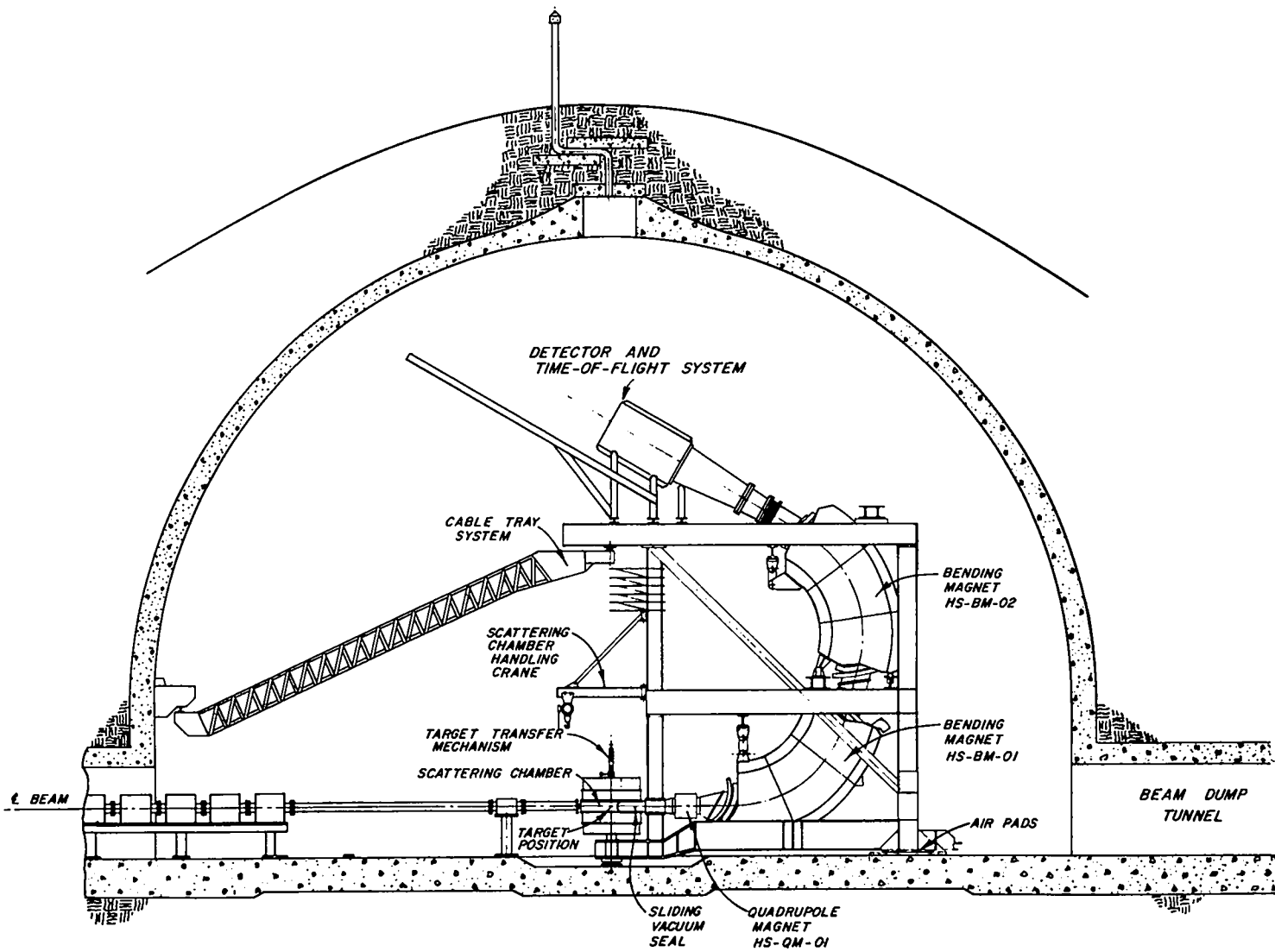
Fig. 21. High-Resolution Spectrometer, elevation (HRS).
