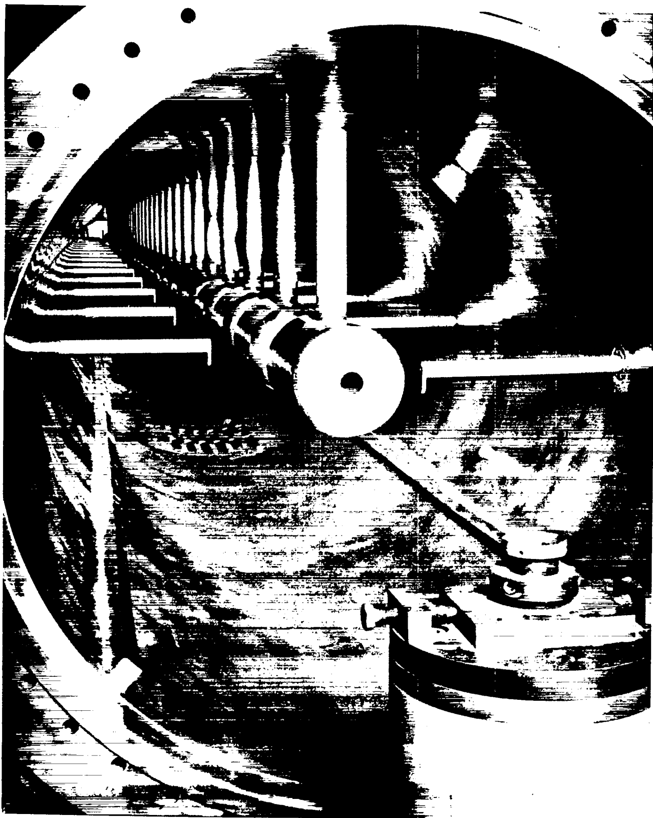
Fig. 7. Drift-tube linac, interior view of electrodes.
