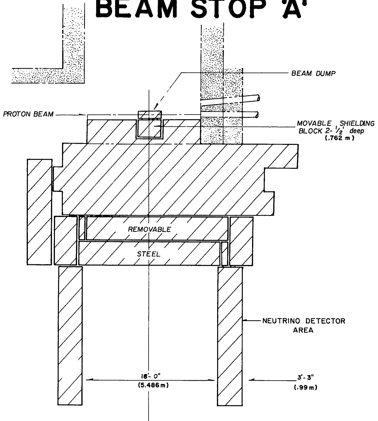
Fig. 26. Neutrino Facility, top view.
