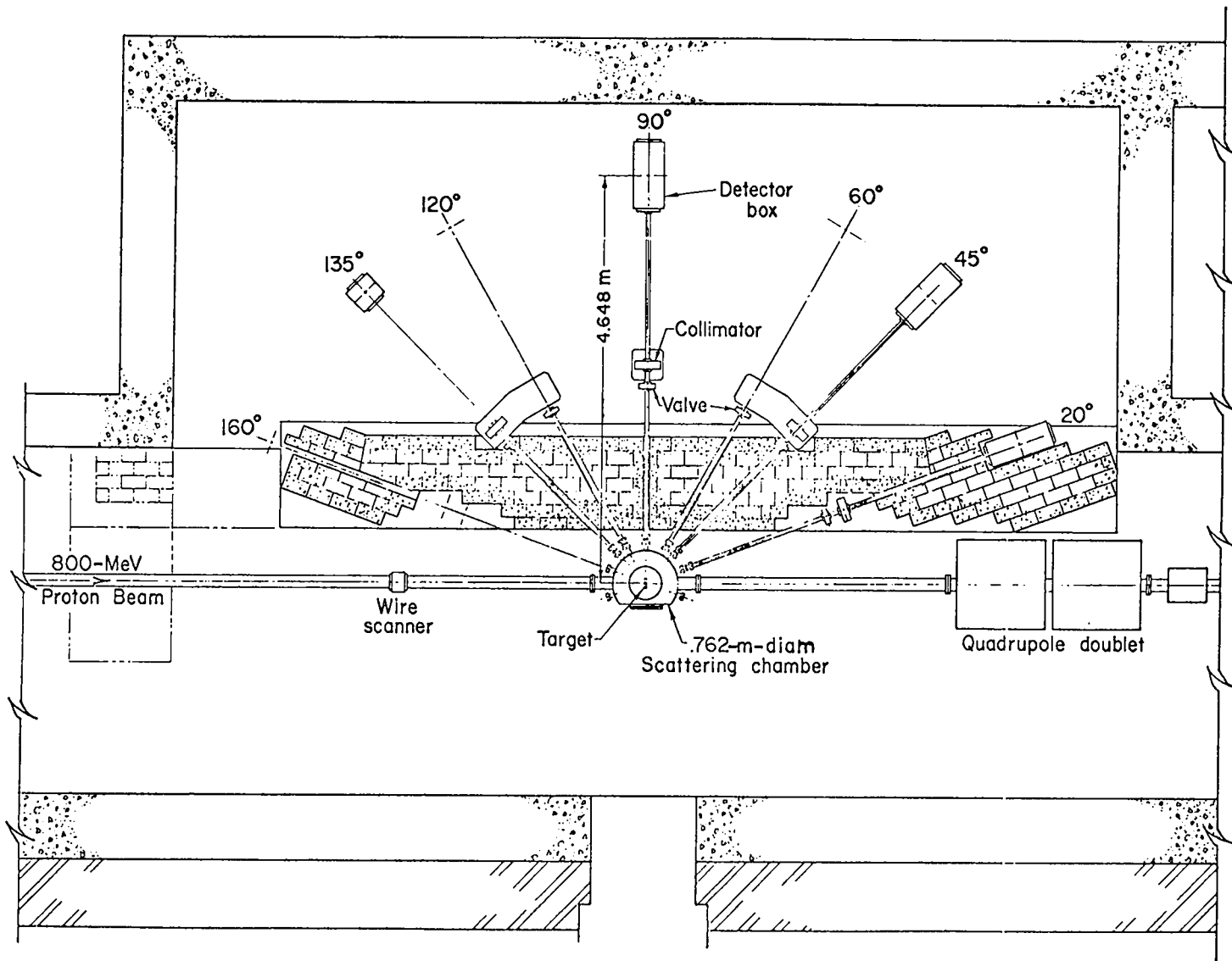
Fig. 22. Thin target area, plan view.
