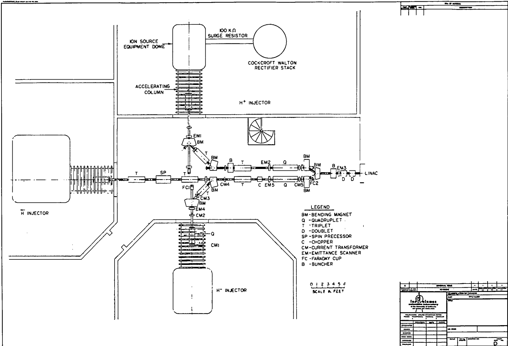
Fig. 3. Injector Building.
