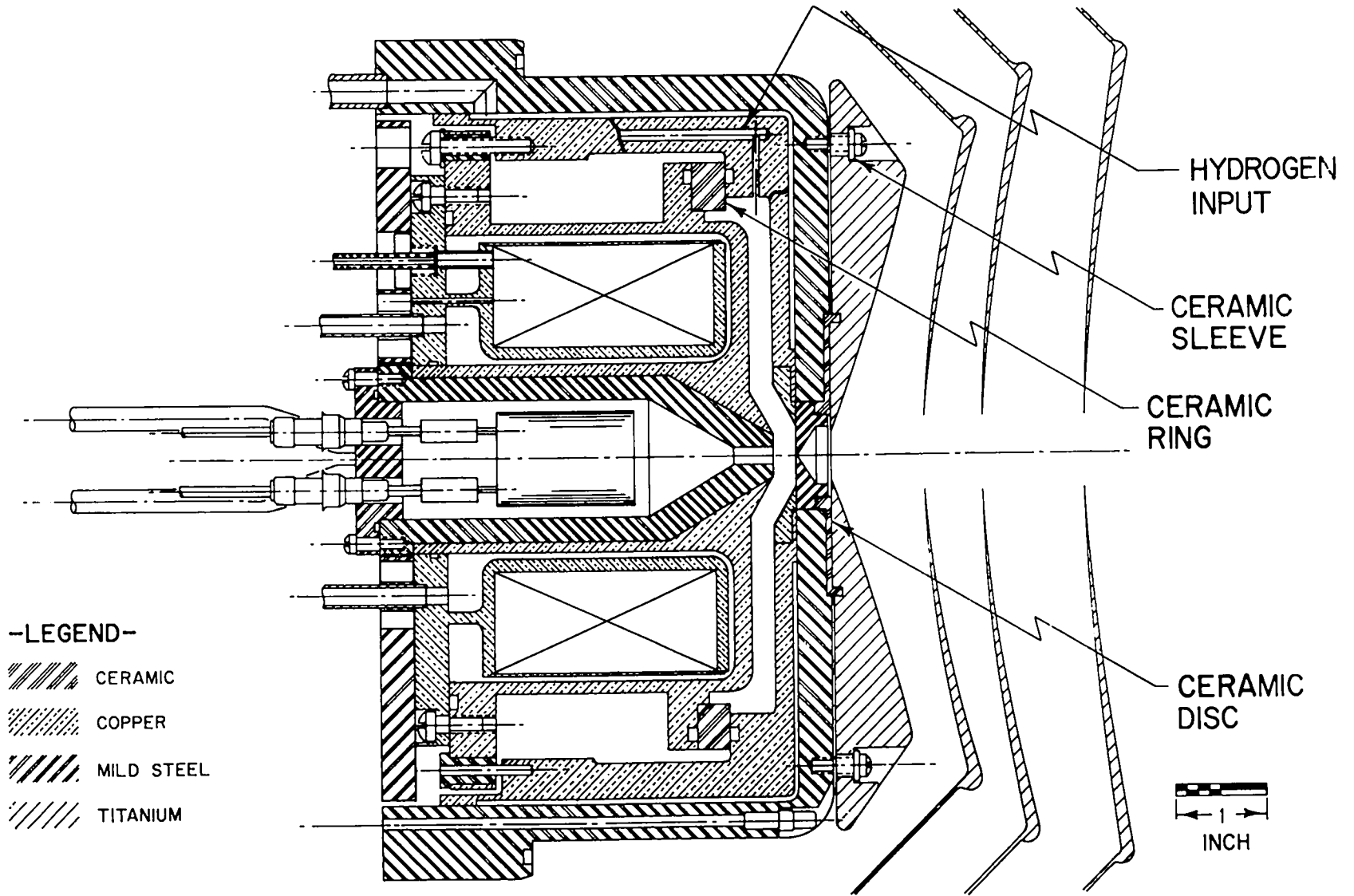
Fig. 5. Proton ion source.
