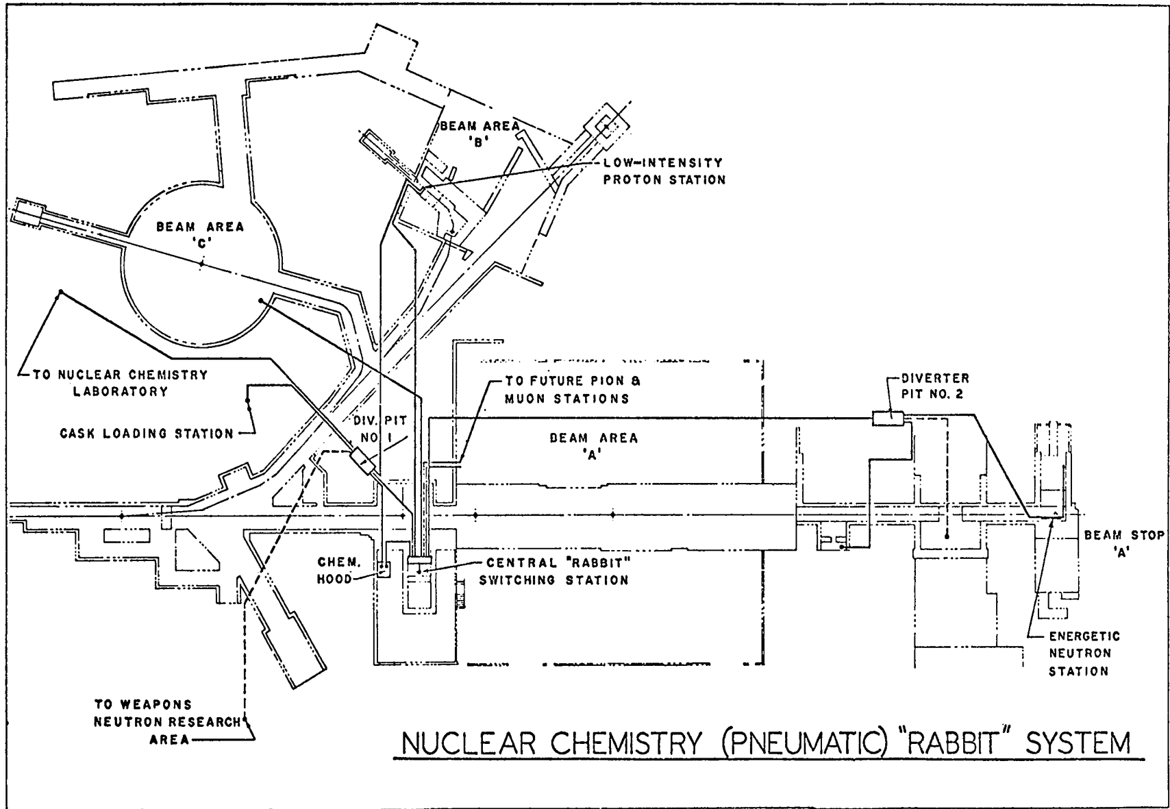
Fig. 24. Radiochemistry pneumatic tube stations.
