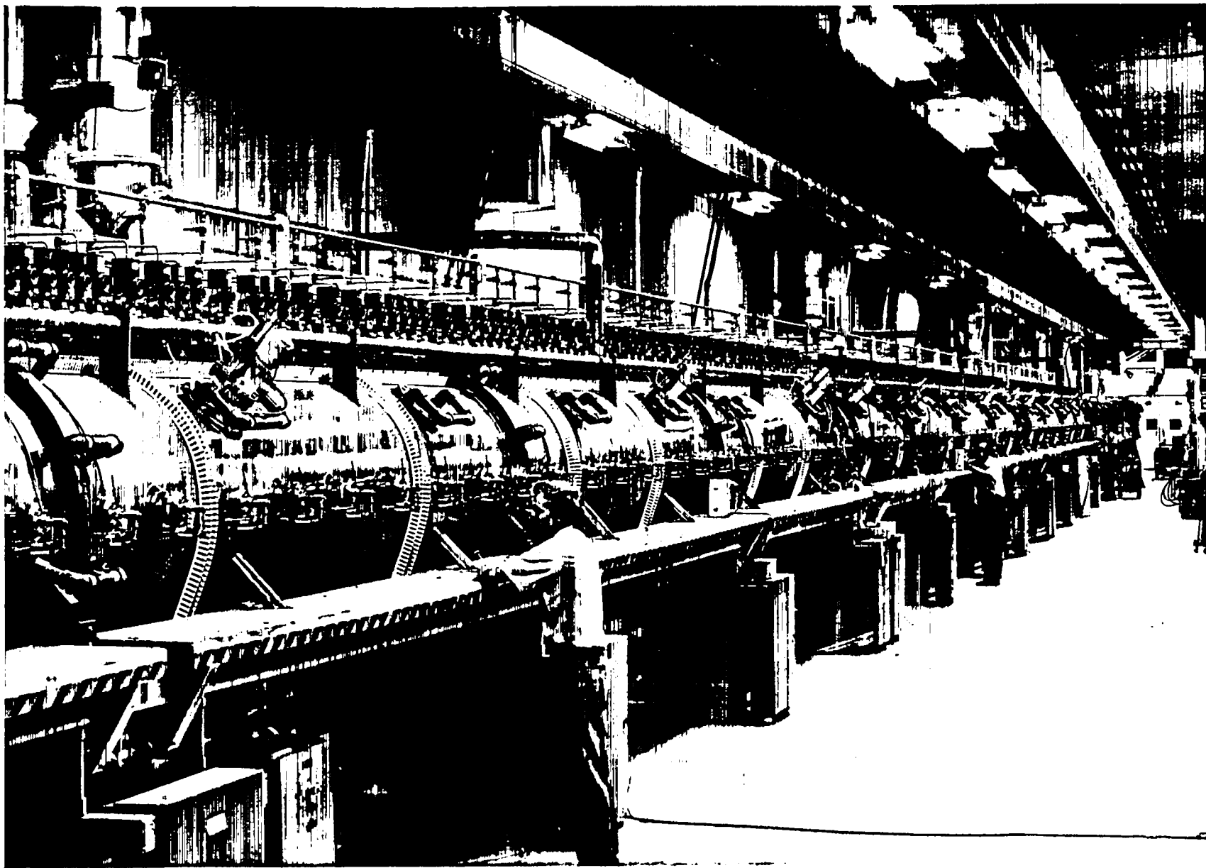
Fig. 8. Drift-tube linac in tunnel.
