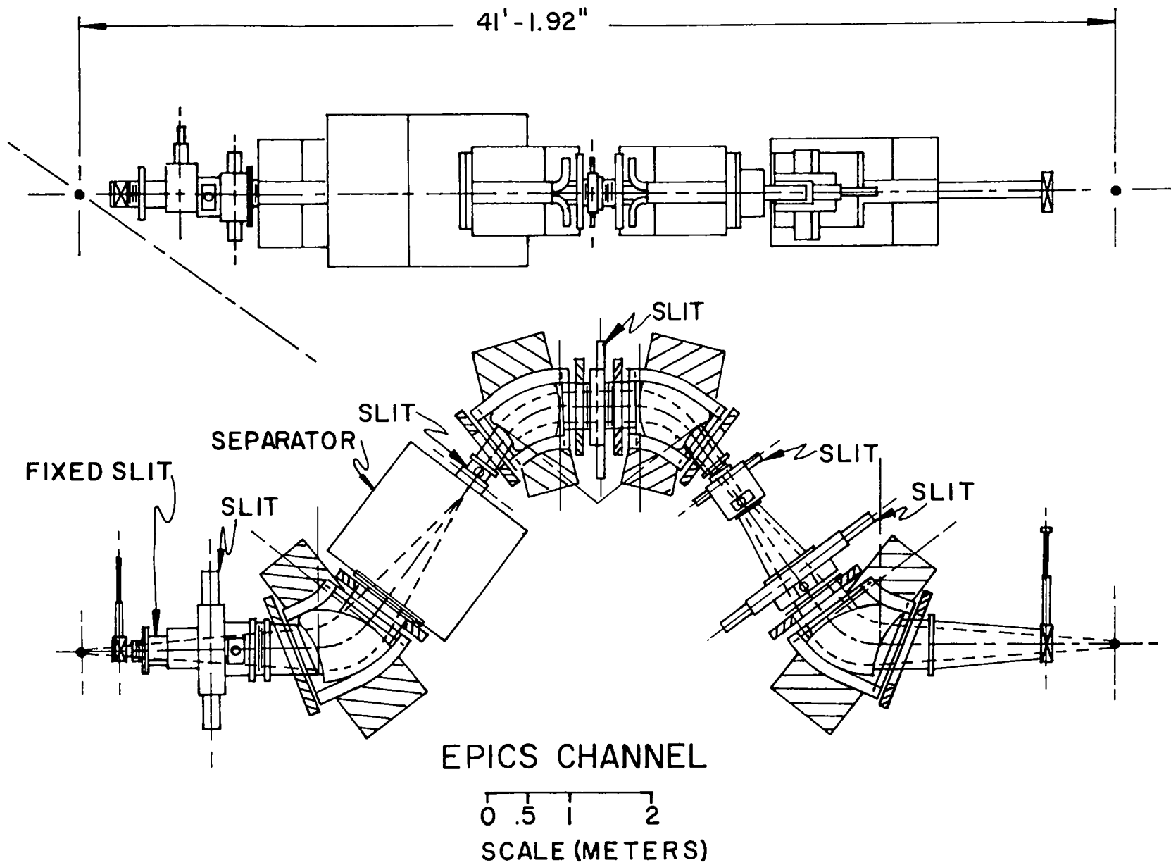
Fig. 16. Energetic Pion Channel (EPICS).
