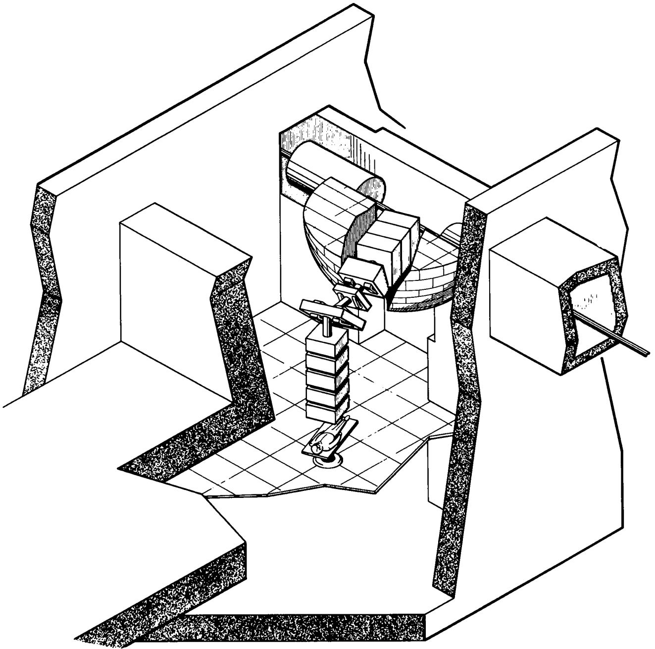
Fig. 28. Biomedical Target Area and general arrangement.
