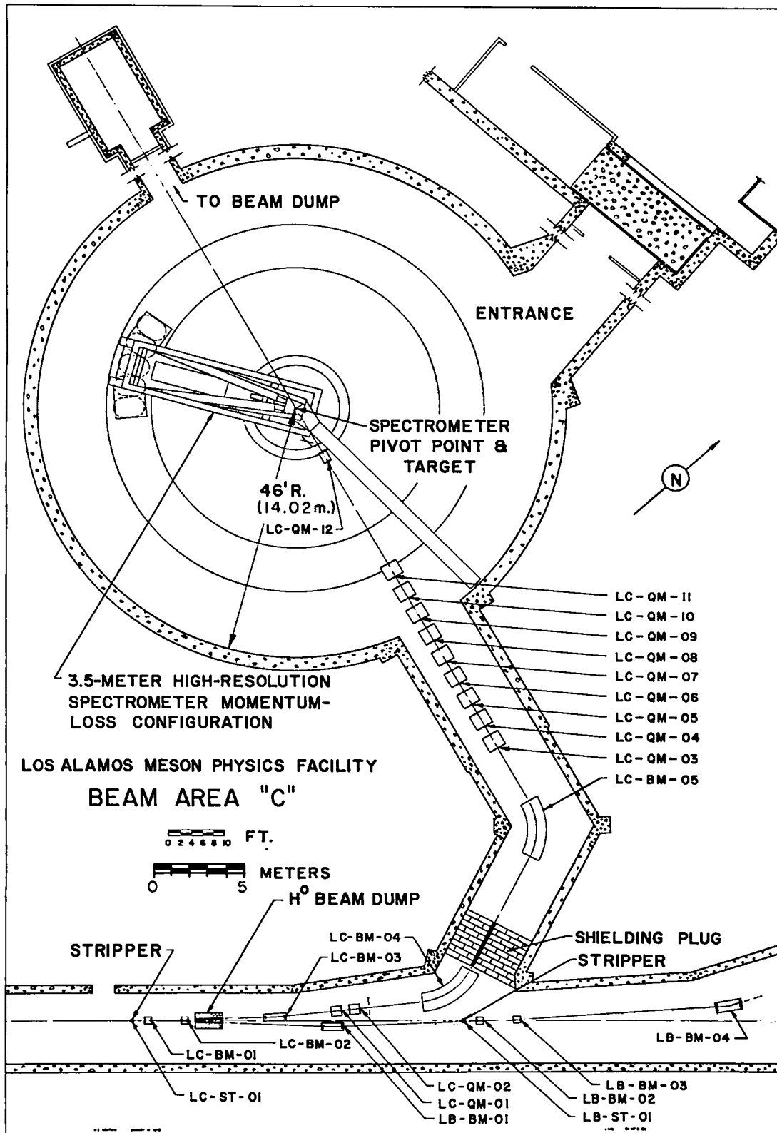
Fig. 20. Experimental Area C.
