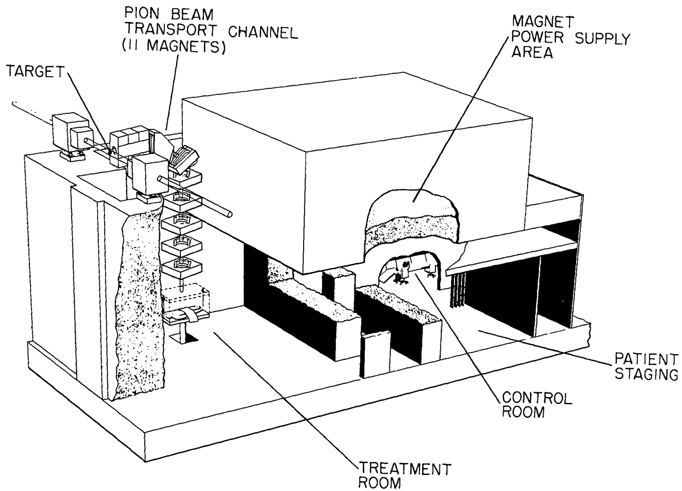
Fig. 30. Pion Radiation Therapy Facility.
