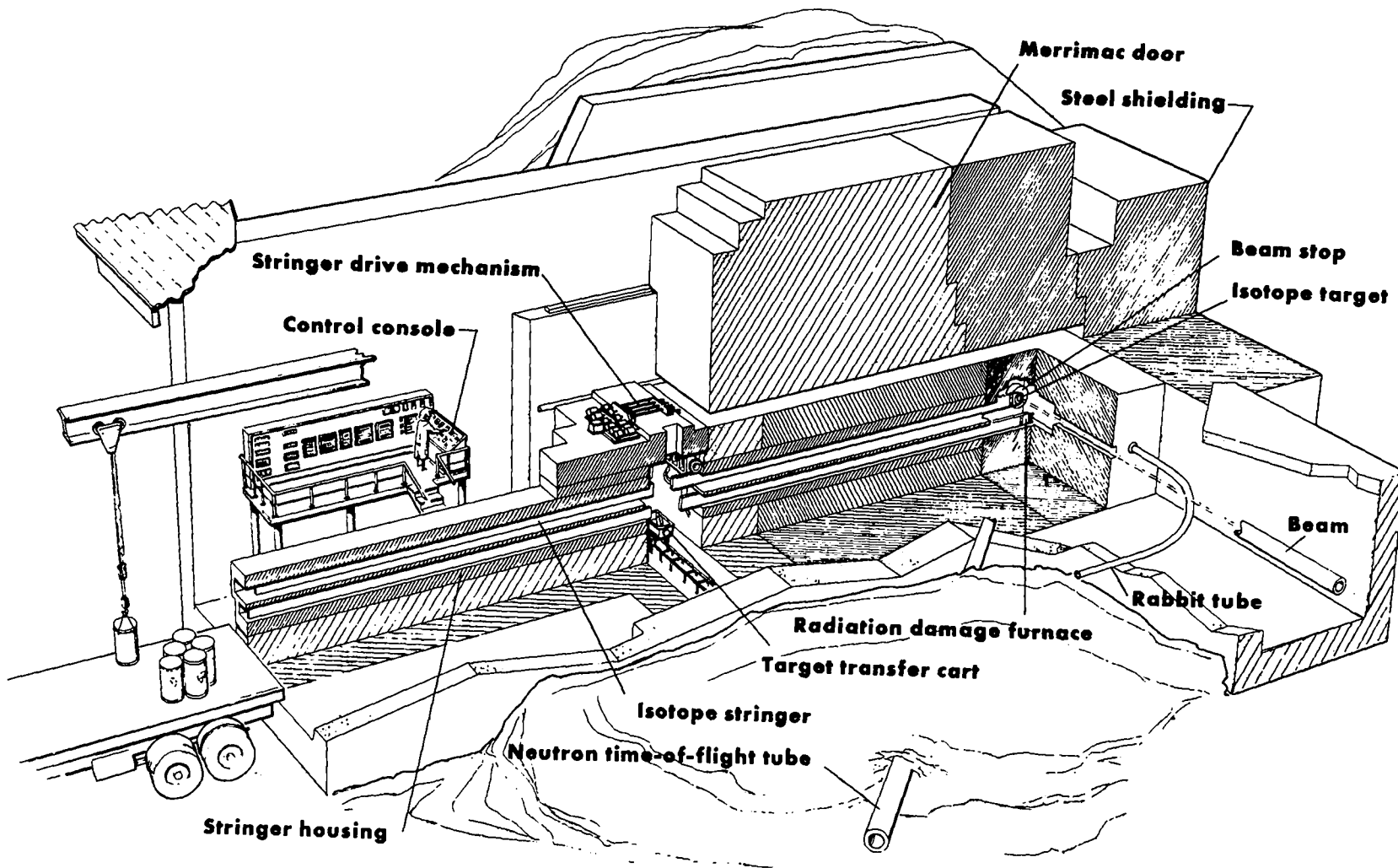
Fig. 25. Isotope Production Facility.
