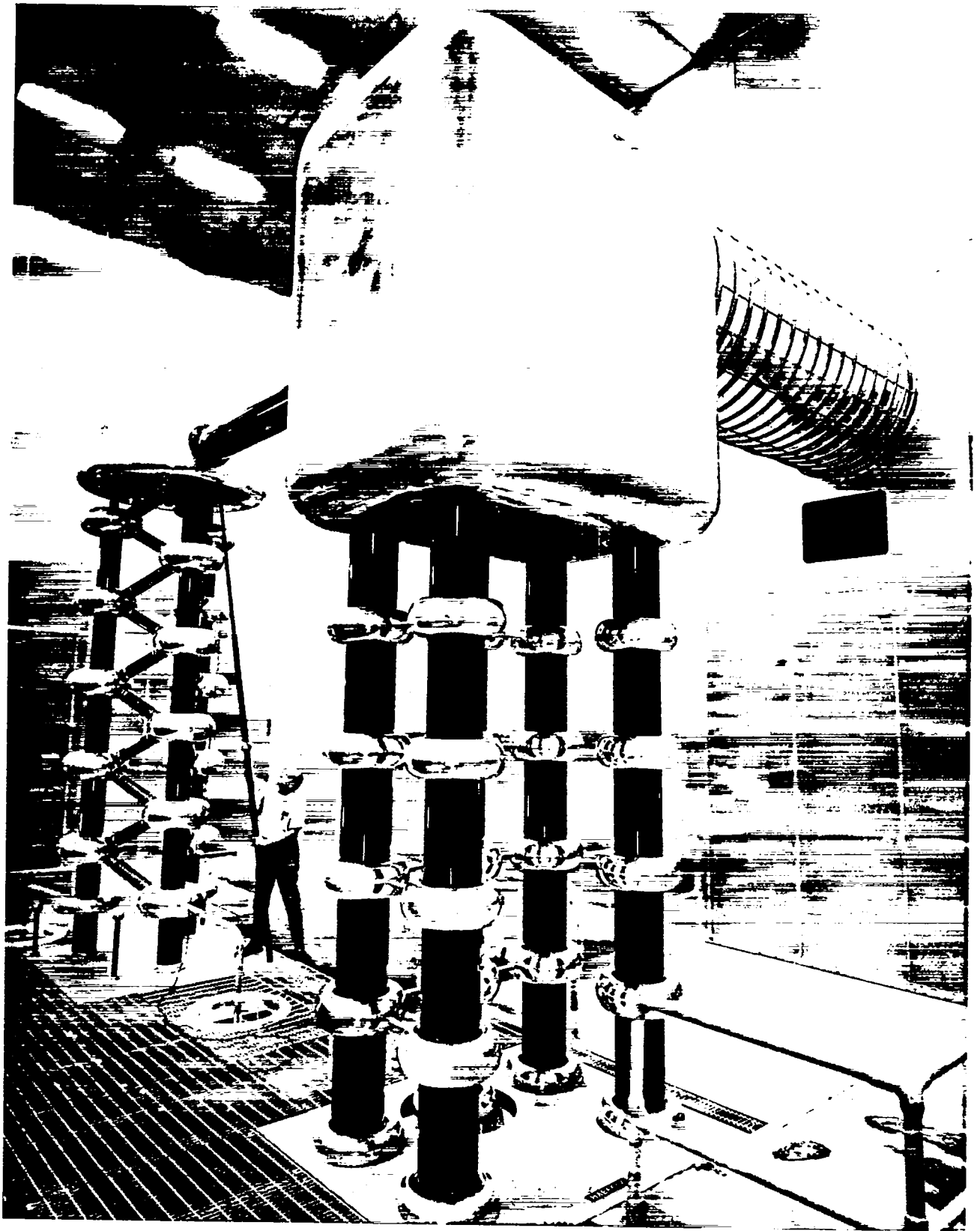
Fig. 4. Cockcroft-Walton 750-keV Preaccelerator.
