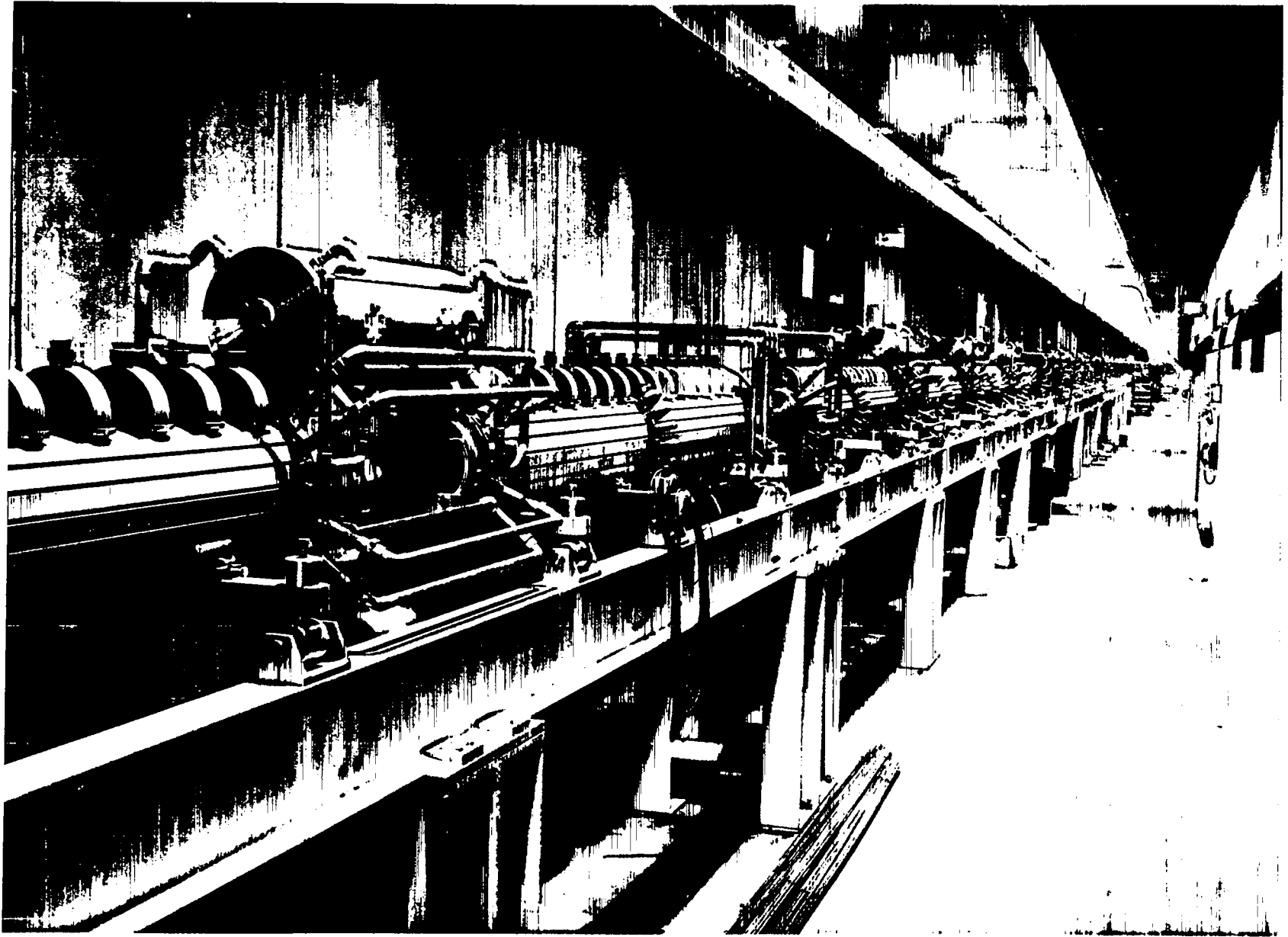
Fig. 10. Side-coupled-cavity linac in tunnel.
