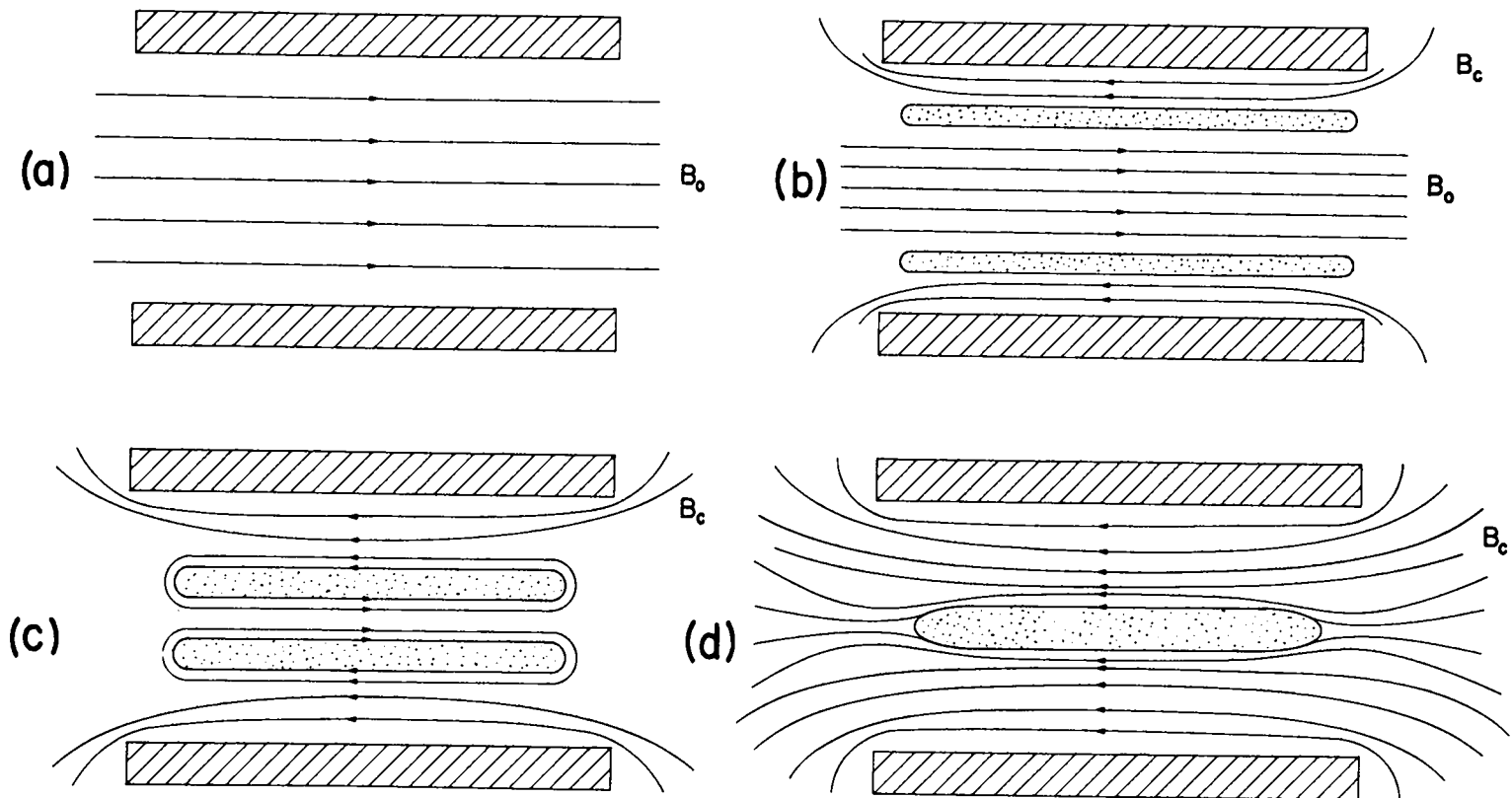
Fig. 3. Reversed trapped field diagrams, illustrating the trapping and annihilation of magnetic field inside the plasma.
