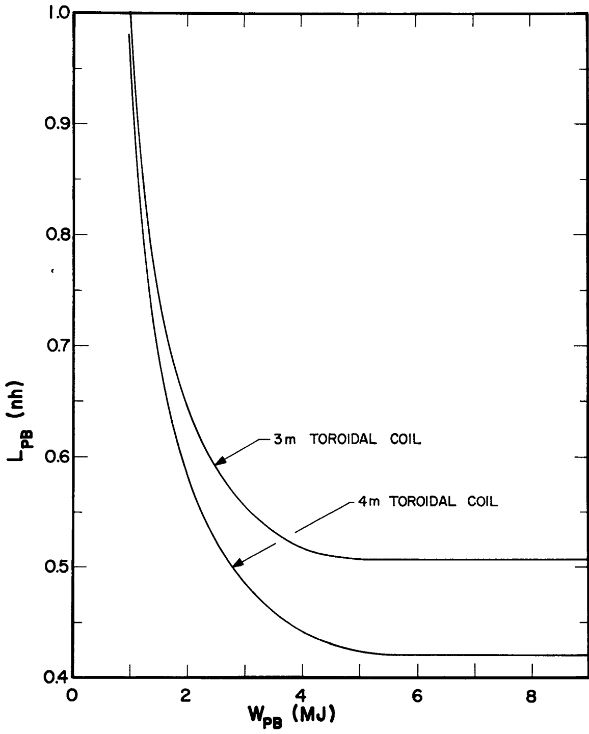
Fig. 30. Inductance of the primary capacitor bank as a function of capacitor energy storage.
