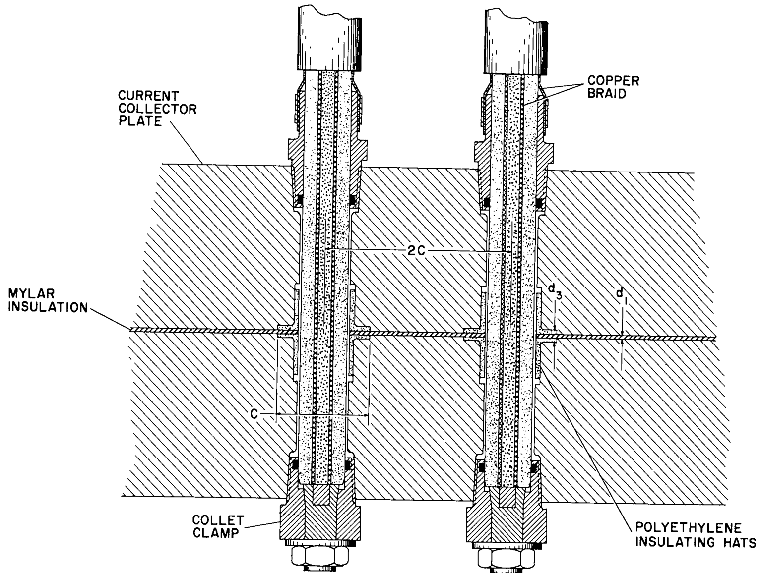
Fig. 29. Detail of the cable feed into the Scyllac collector plate.
