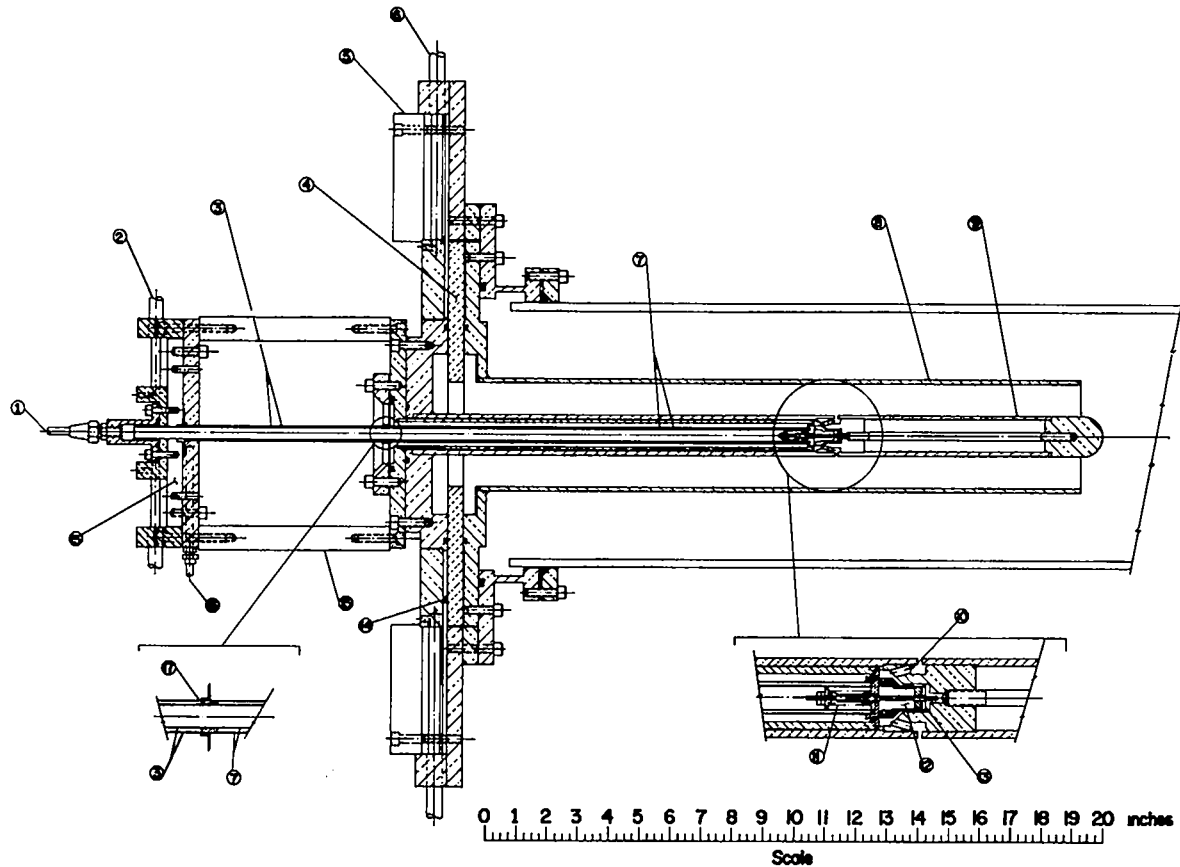
Fig. 1. Plasma gun design with fast thermal expansion valve. (1) Gas inlet. (2) Sixteen REX-4 cables to valve driver capacitor bank. (3) Driver section. (4) One-half-in.-thick glass insulator. (5) Lucite clamping ring. (6) Twenty-four B.I.C.C. Type-20 cables to gun capacitor bank. (7) Sonic line. (8) Outer electrode. (9) Inner electrode. (10) Gas outlet holes (15 holes, 1/8-in. diam). (11) Valve spring. (12) Valve plenum. (13) Teflon bumper washer. (14) Polyethylene insulation. (15) Phenolic insulator. (16) Cooling air inlet. (17) Small holes for air outlet.
