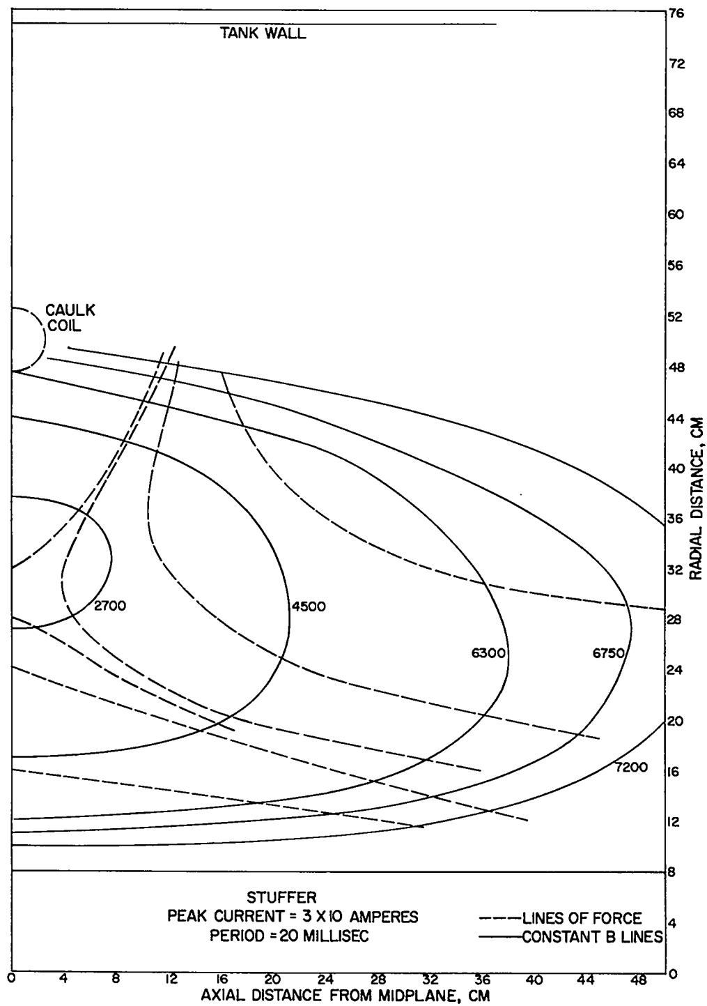
Fig. 2. Mark III caulked stuffed picket fence.
