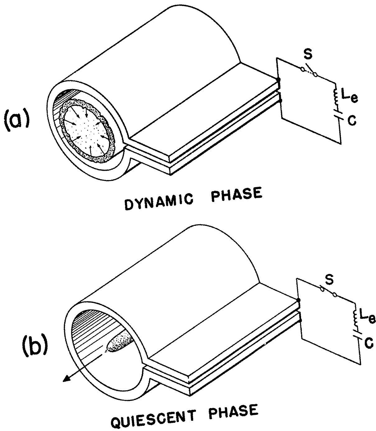
Fig. 1. Simplified schematic view of a theta pinch.
