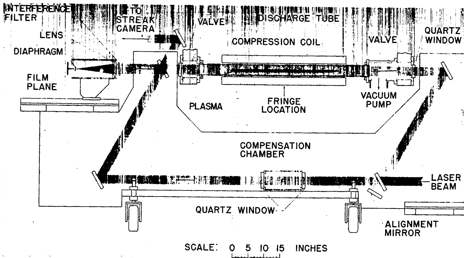
Fig. 14. Diagram of the Scylla IV discharge tube and Mach-Zehnder interferometer used for making plasma density measurements.
