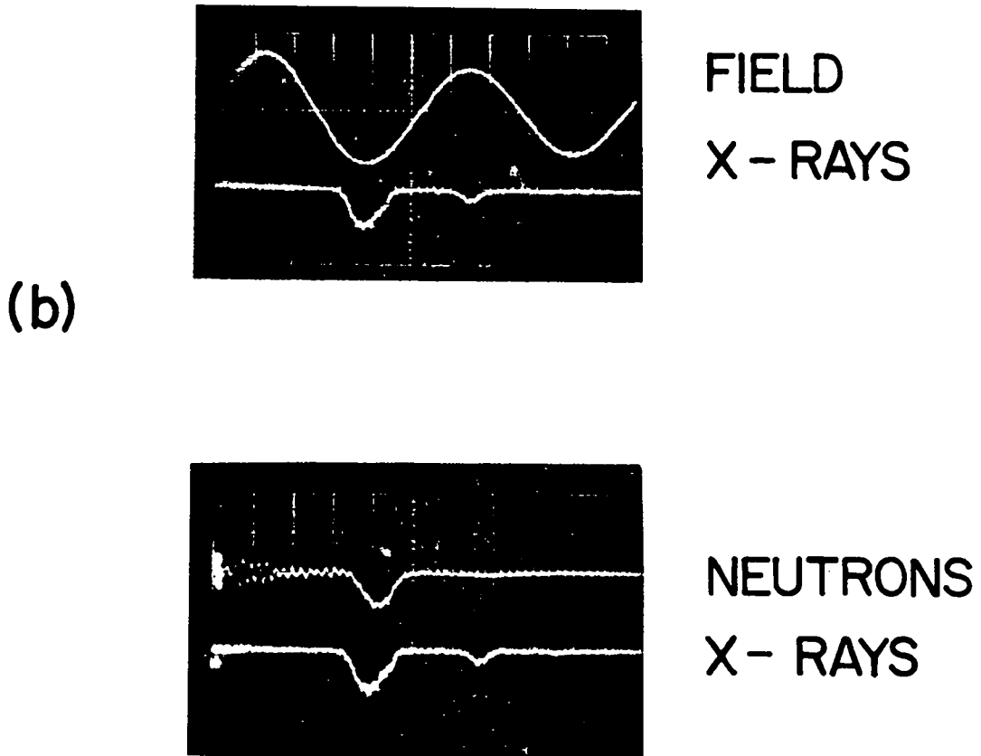
Fig. 2. (a) Cross-sectional drawing of Scylla I compression coil and discharge tube. (b) Oscillograms of compression-coil current (proportional to magnetic field) and the neutron and soft x-ray signals. The horizontal time scale is 1 \mu\text{sec} per division.
