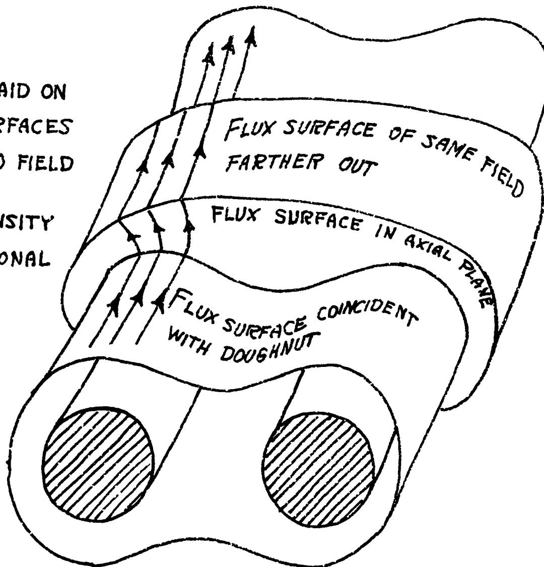
Fig. 7. Field extension in injection region.
