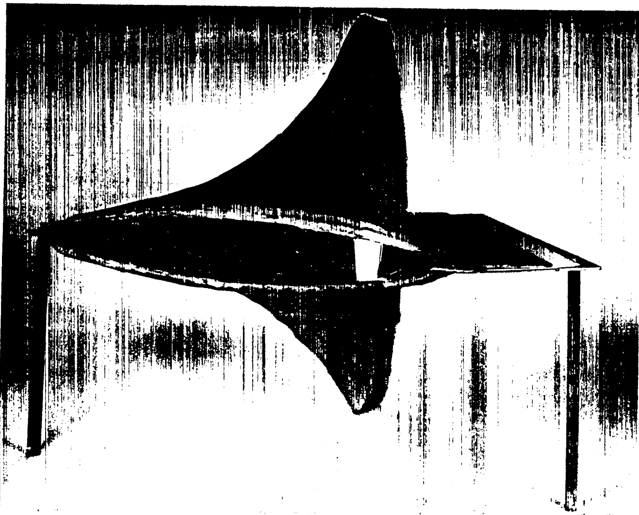
Fig. 23. A model section of a periodic \theta -pinch compression coil in which stabilization fields are obtained by shaping the inner surface of the conductor.
