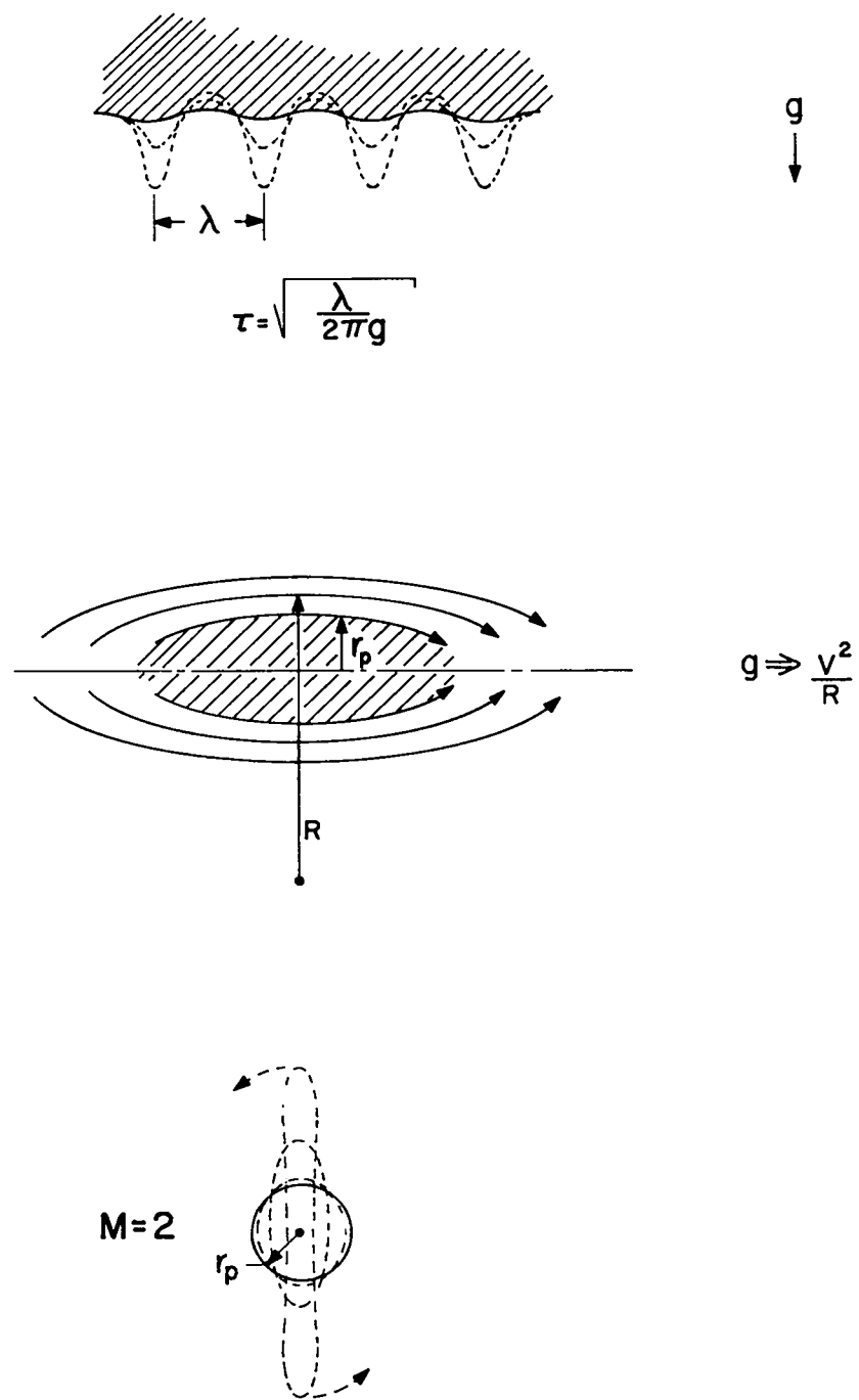
Fig. 7. Model of Rayleigh-Taylor instability (upper diagram) for a plane fluid interface and plasma flute instability (lower diagram) in the presence of curved magnetic lines (center diagram).
