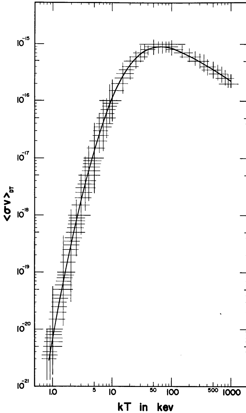
Fig. 31. The nuclear cross-section for fusion reactions between deuterons and tritons averaged over a Maxwell distribution of velocities as a function of temperature.
