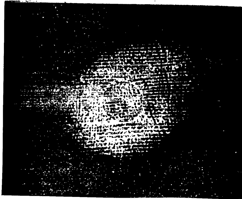
Fig. 13. (a) Shadowgram of Scylla IV plasma at peak compression taken in parallel red (ruby laser) light. Density gradient serves to focus rays on photographic plate, thus showing boundary of plasma. (b) Compressed plasma is seen in deflection mapping by grid lines ruled on a window between the plasma and a camera. One can see the circular plasma outline in the kinks of the grid lines.
