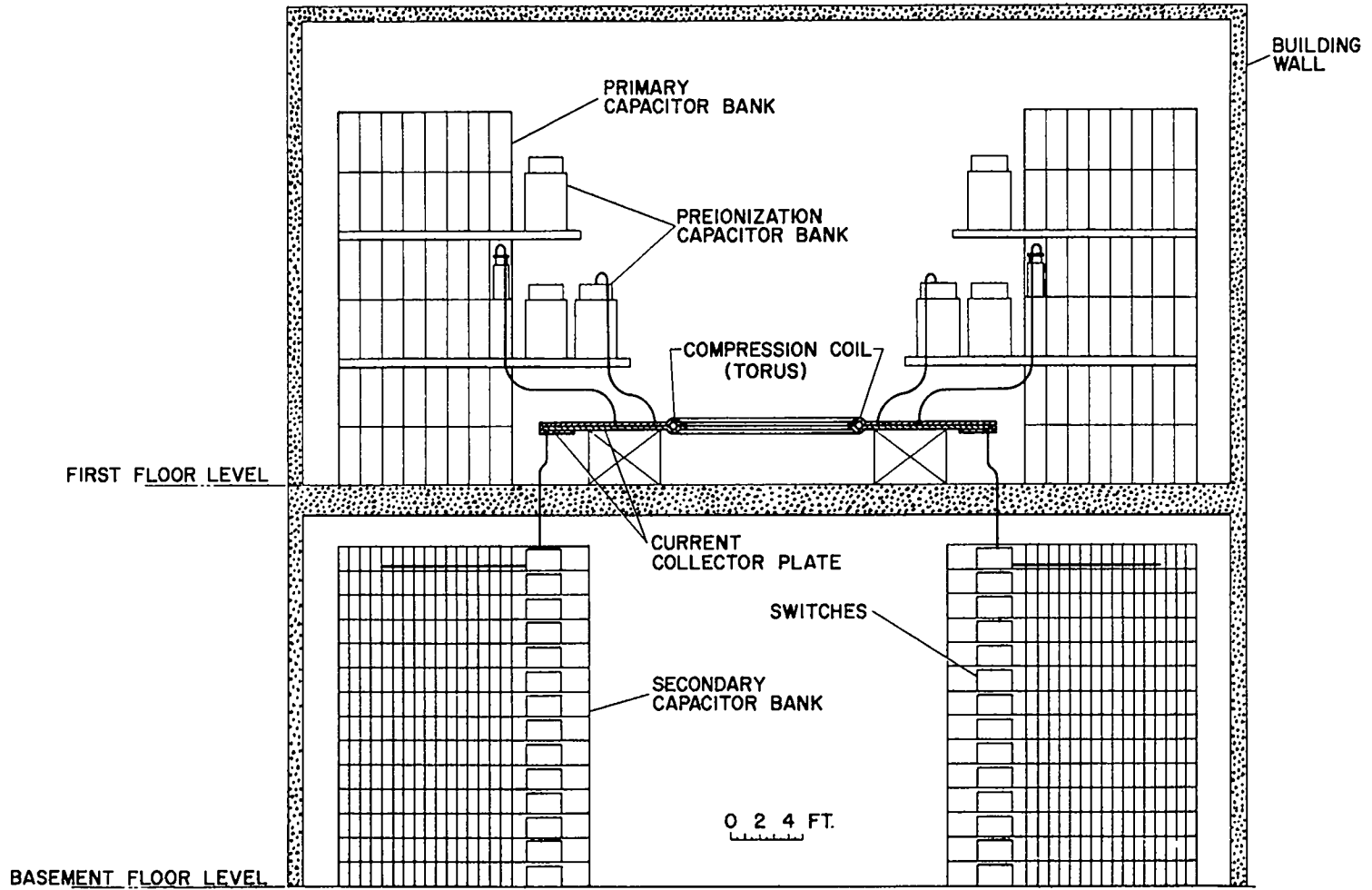
Fig. 26. Elevation of the proposed Scyllac experiment.
