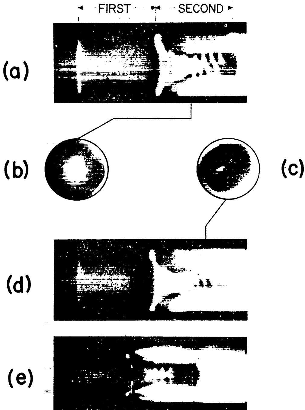
Fig. 8. Photographs of the Scylla III plasma. (a) and (d) are streak-camera, end-on photographs of the rotating flute instability in Scylla III. (b) and (c) are Kerr-cell photographs of the plasma cross sections at the times indicated. The half-cycle duration is 5 \mu sec.
