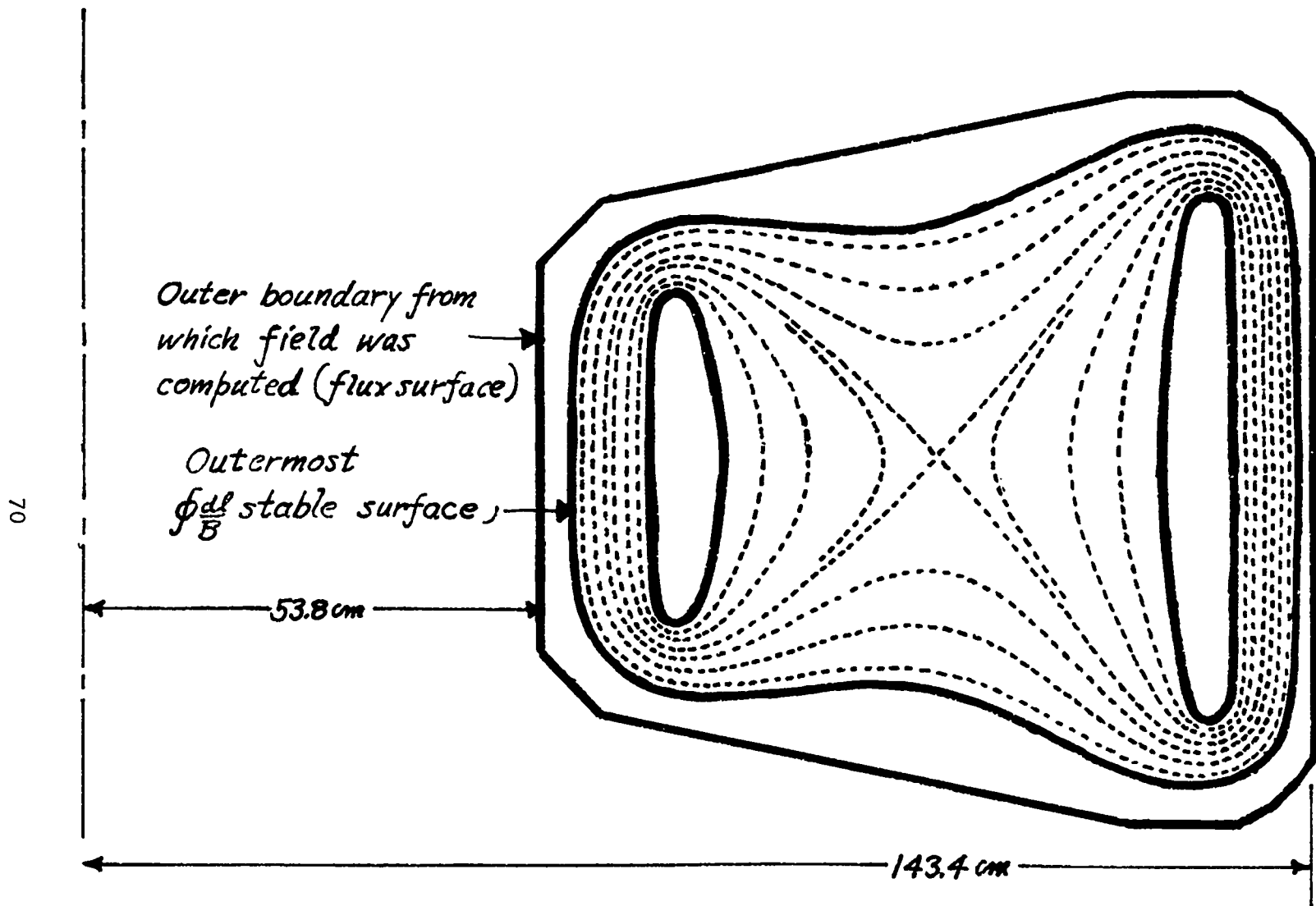
Fig. 5. Present least-energy quadrupole field.
