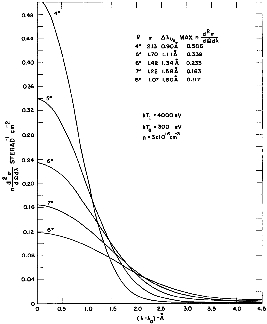
Fig. 24. Absolute differential scattering cross section vs wavelength difference from that of the incident laser beam for assumed Maxwellian distributions of ion and electron velocities at the temperatures and density indicated. The parameter of the curves is the scattering angle \theta_s .
