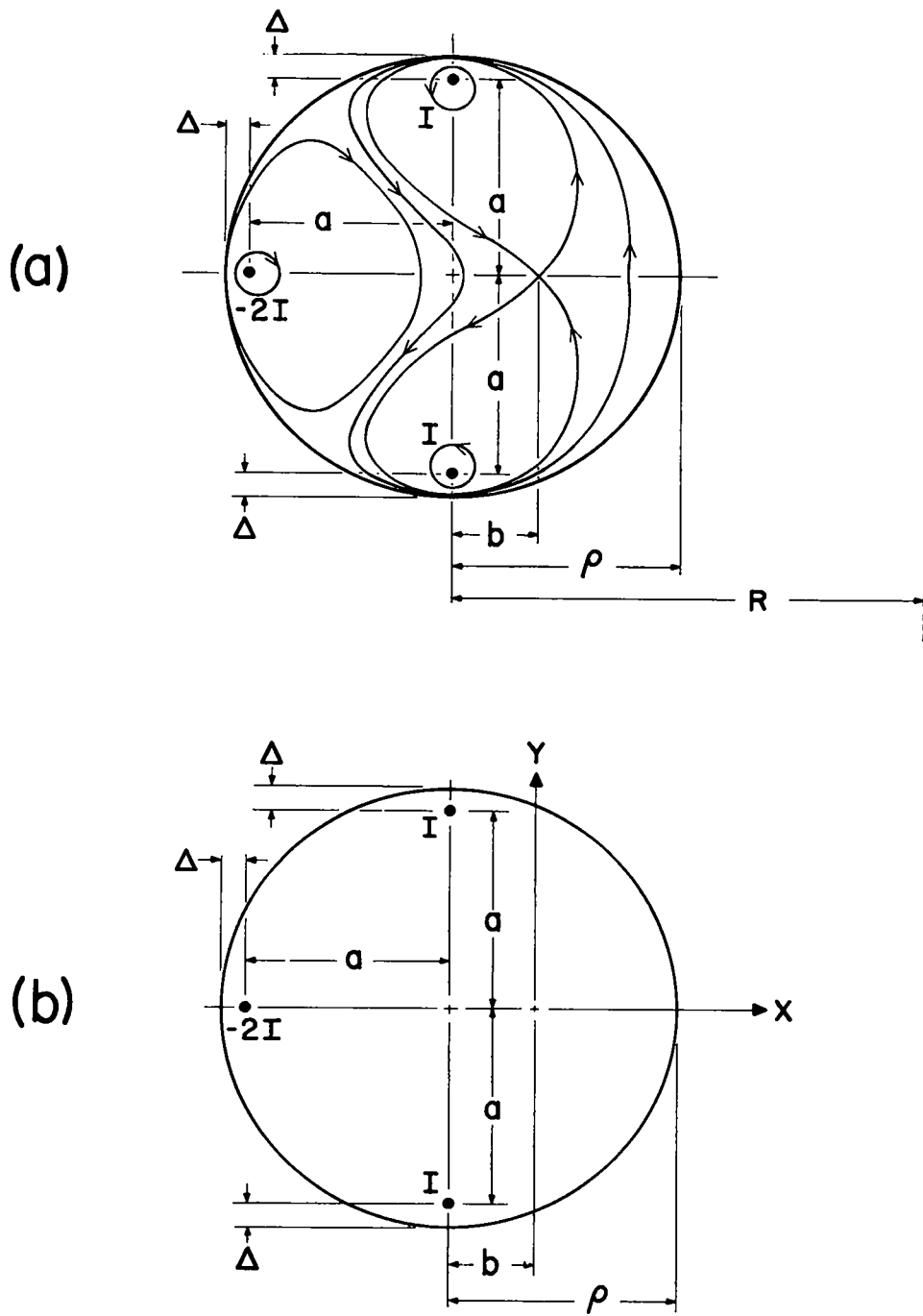
Fig. 33. Configuration of multipole conductors for stabilization of a toroidal \theta pinch. (a) shows the position of the bars and the magnetic field-line configuration, (b) shows the change of coordinates for calculating the scalar potential.
