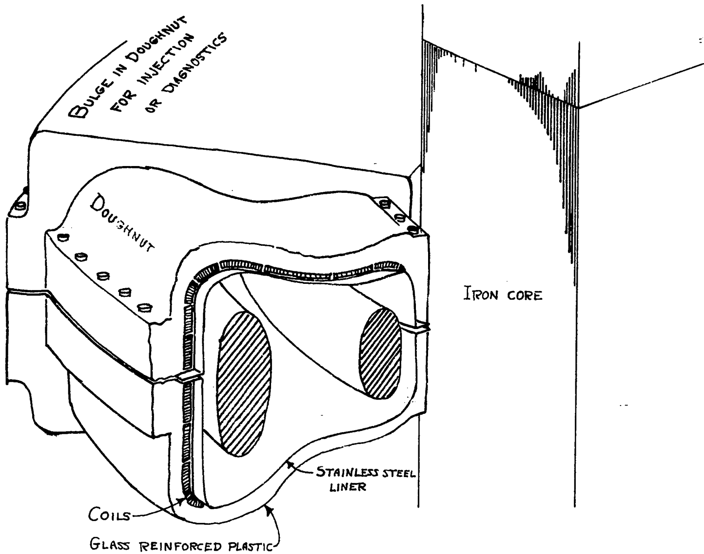
Fig. 6. Conceptual toroidal quadrupole machine (Cut away).
