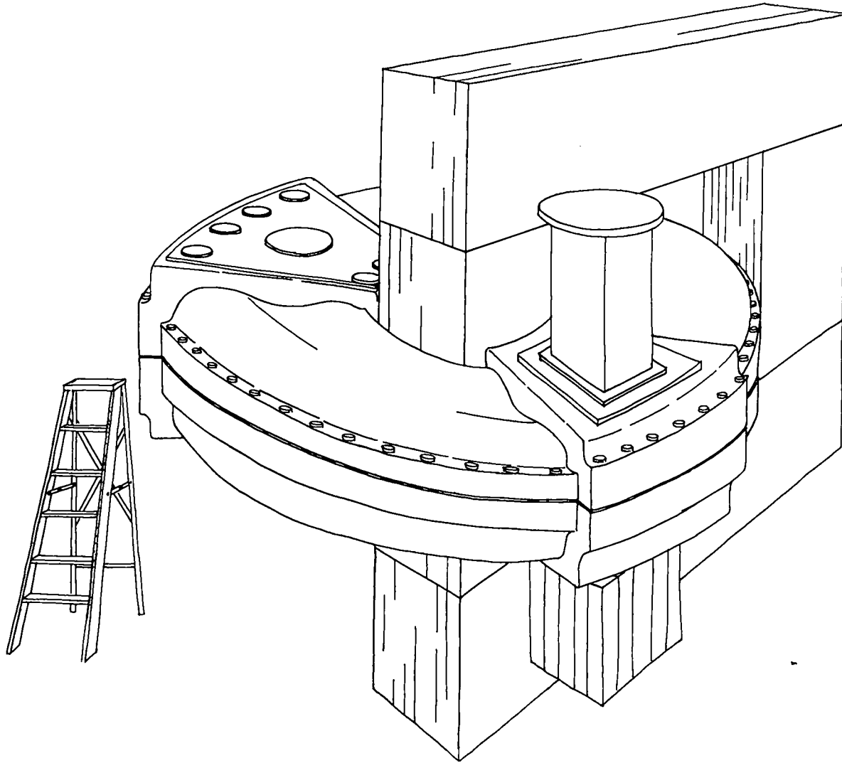
Fig. 8. Conceptual toroidal quadrupole machine. Cables, levitation details, and experimental ports are left out for simplicity.
