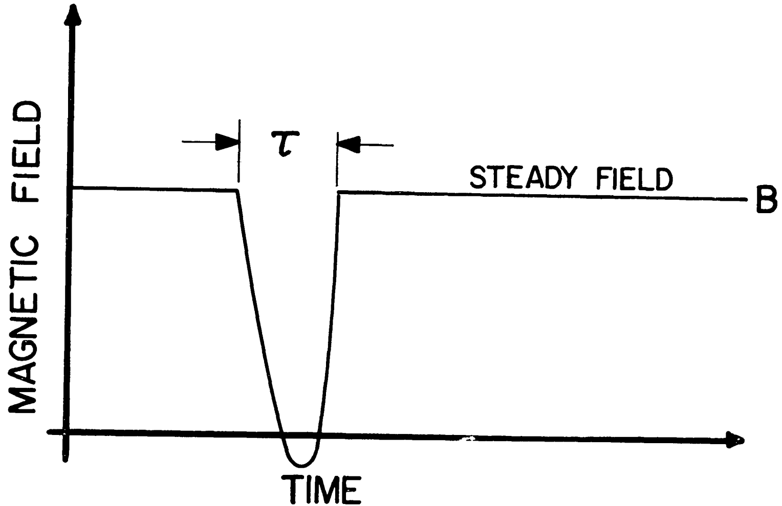
Fig. 18. Time history of the magnetic field in the sustained field \theta pinch. An impulse of magnetic field is superimposed on a steady field B, driving the magnetic field to zero. The plasma is formed on the backswing of magnetic field and sustained by the steady field B.
