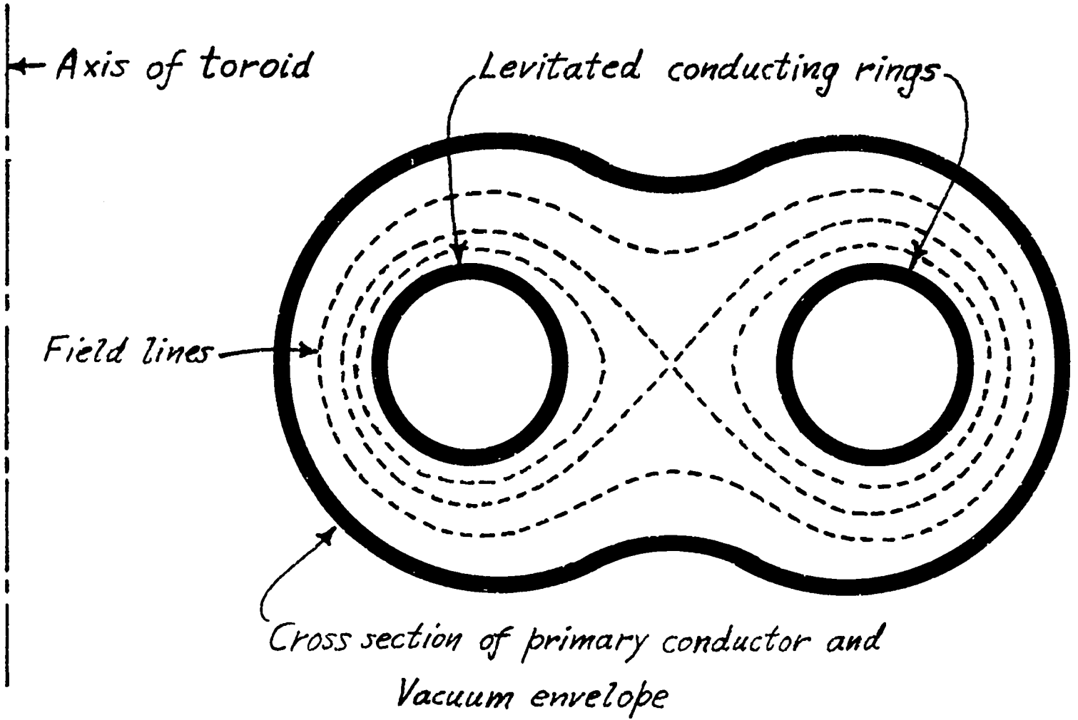
Fig. 2. Toroidal quadrupole configuration.
