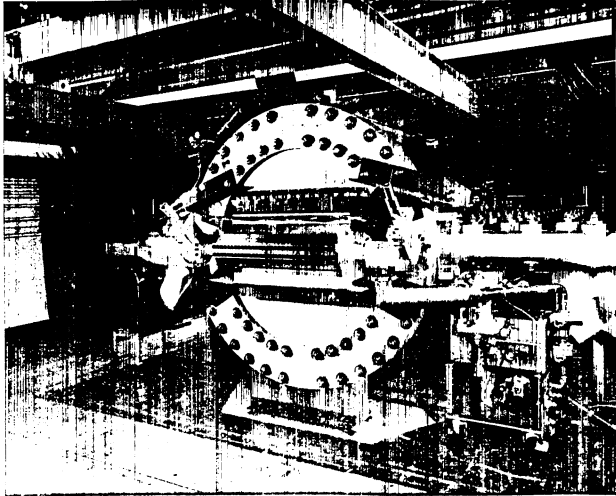
Fig. 12. Front-end of Scylla IV. The one-meter aluminum compression coil bolts to the current collector plates which consist of 3-in.-thick aluminum alloy, held together by 170 steel bolts (seen in the right rear). The large circular piece is a clamp to balance the 1600 atmospheres of magnetic pressure between the collector plates at the coil feed point.
