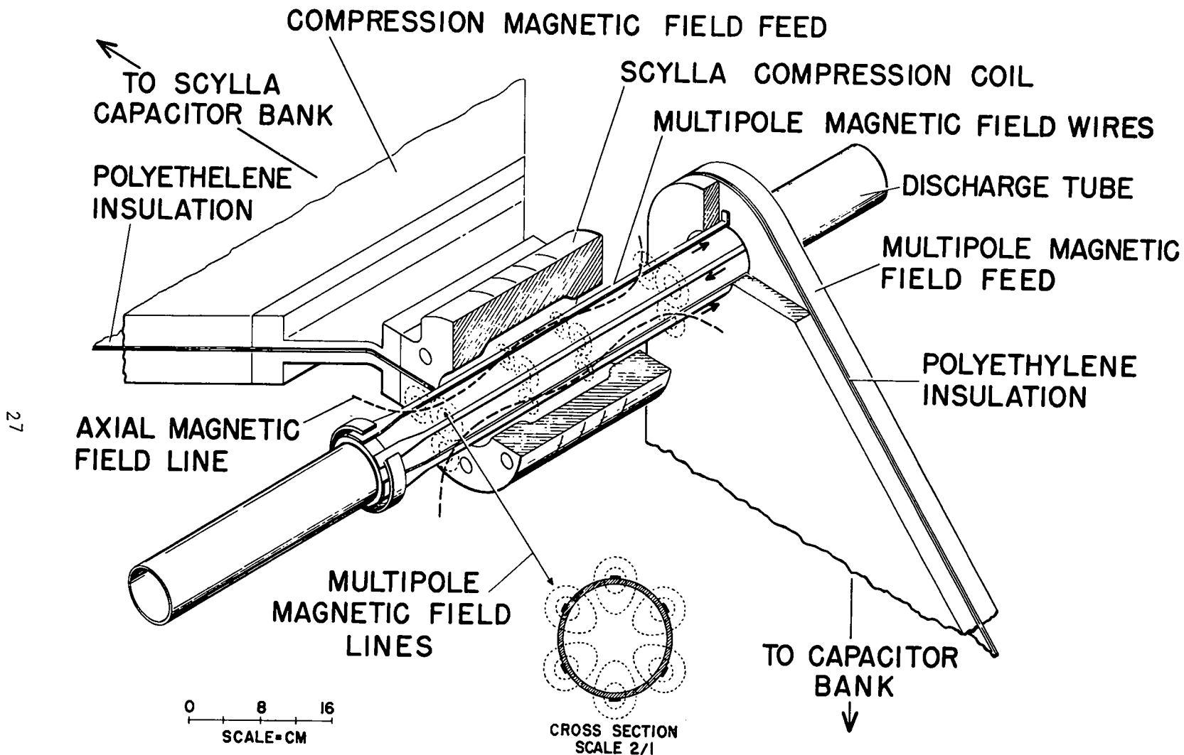
Fig. 9. Diagram of apparatus for applying a hexapolar field to the Scylla III plasma. The six wires parallel to the pinch axis apply magnetic lines, in radial planes, which are convex to the plasma.
