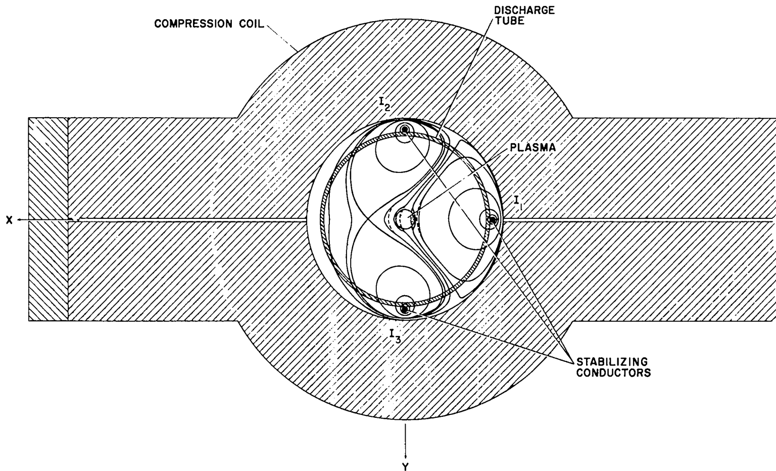
Fig. 19. Cross-sectional view of \theta -pinch compression coil with three conductors to furnish an asymmetric quadrupole field whose lines are shown. The magnetic lines are indicated by a \beta = 1 plasma and qualitatively by the dashed lines in the absence of plasma.
