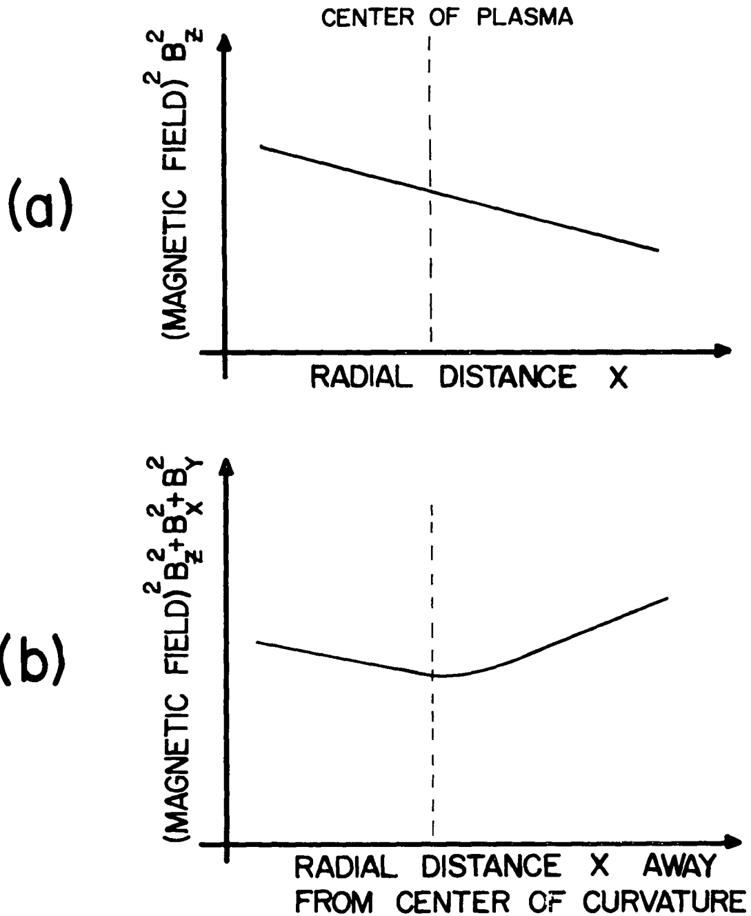
Fig. 20. (a) Magnetic pressure vs radius for curved magnetic lines whose tangent is in the z direction. (b) Magnetic pressure with added x and y components as furnished by the asymmetric quadrupole of Fig. 19.
