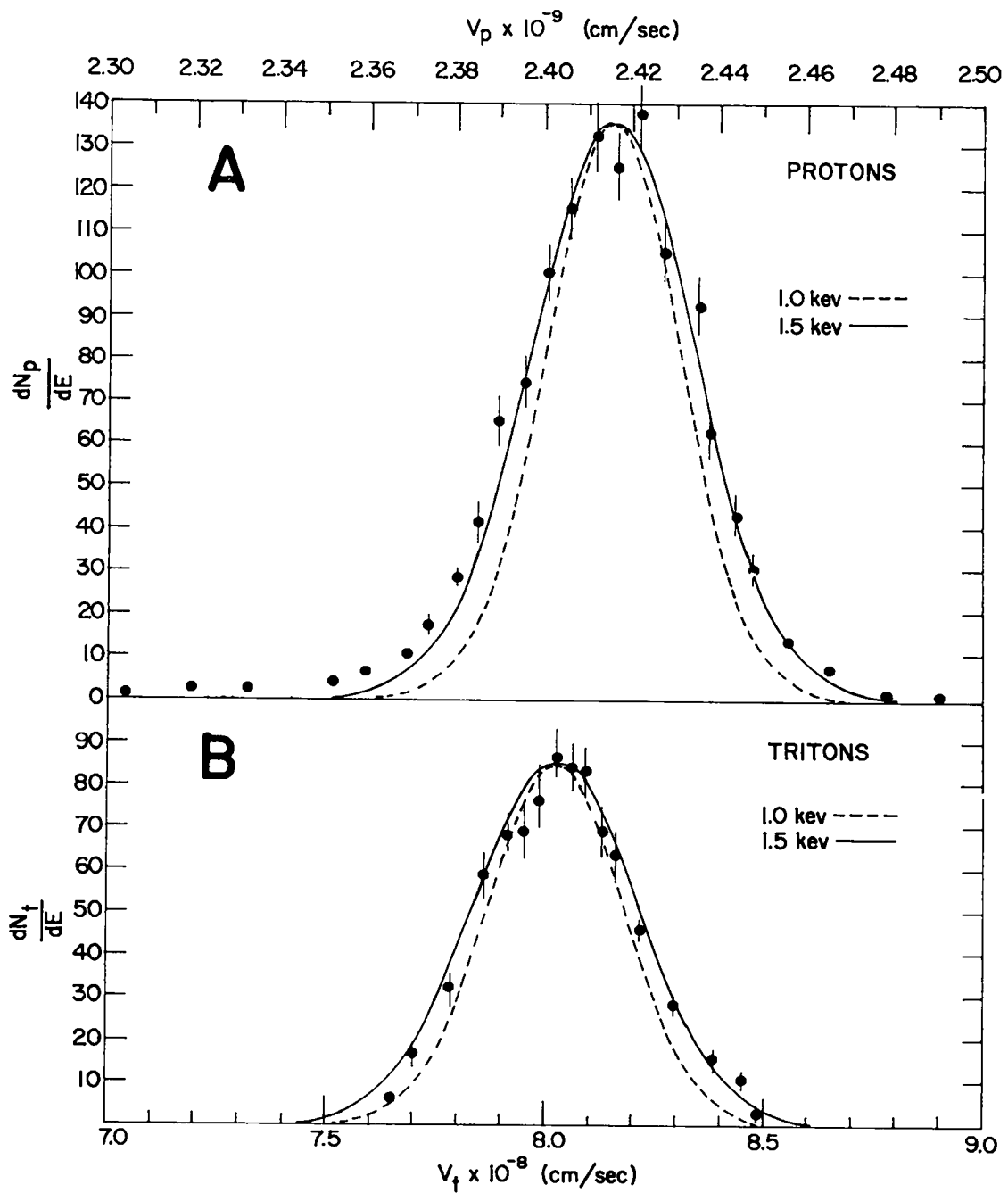
Fig. 6. Spectra of d-d protons and tritons emitted axially from the Scylla I plasma as measured in the arrangement of Fig. 5. Theoretical curves computed for Maxwellian ion velocity distributions of temperatures 1.0 and 1.5 keV are compared with the measured data points.
