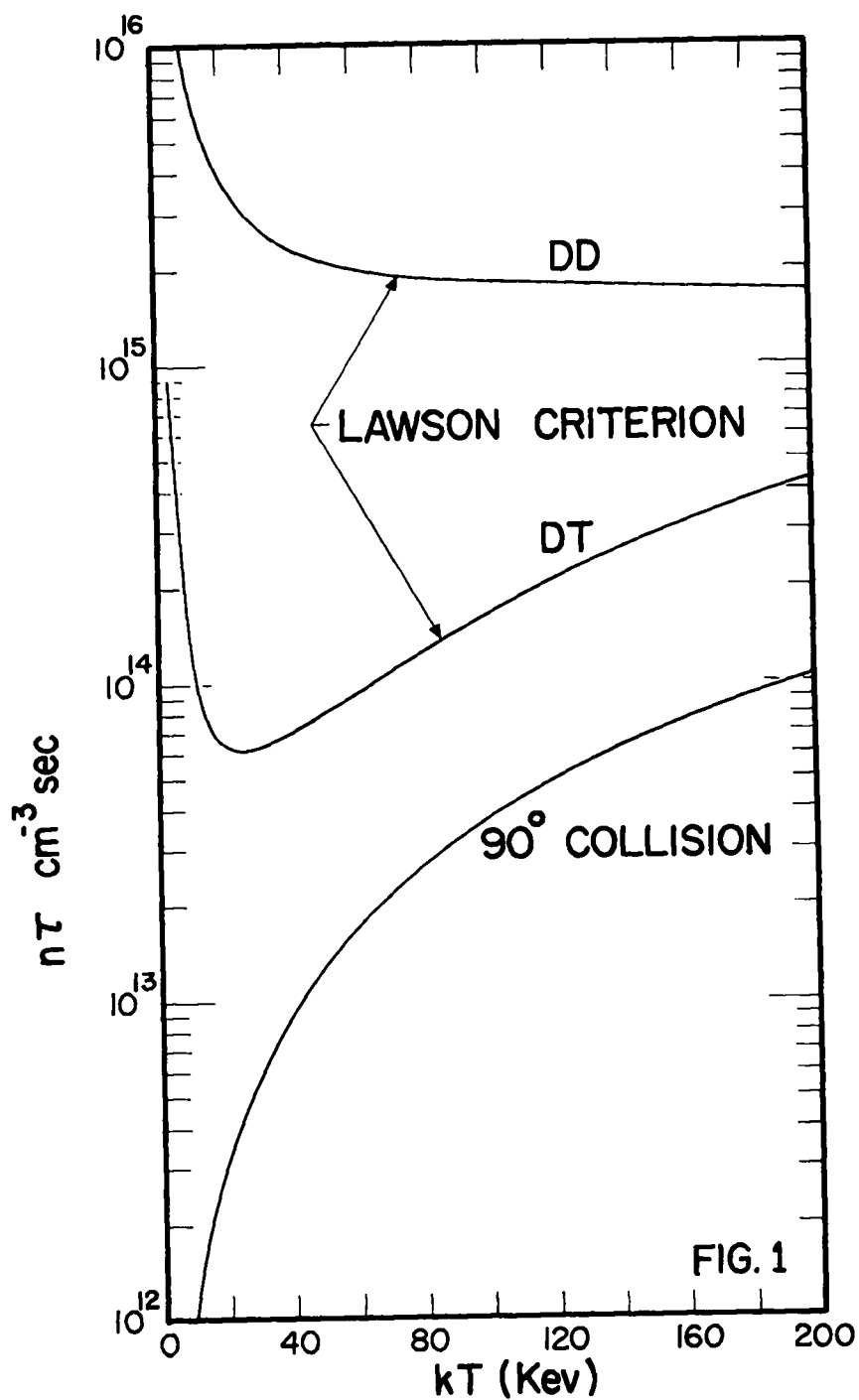
Fig. 1. The Lawson criterion for net energy production in a thermonuclear plasma and the n\tau for 90^\circ ion deflections in the plasma.
