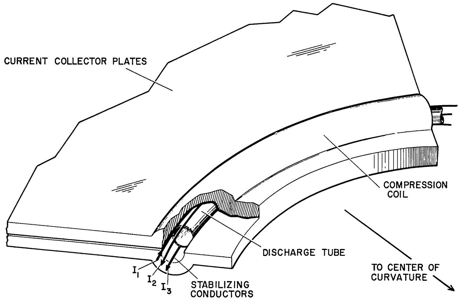
Fig. 21. Schematic view of curved sector coil for a \theta pinch using stabilizing conductors, corresponding to the cross-sectional drawing of Fig. 19.
