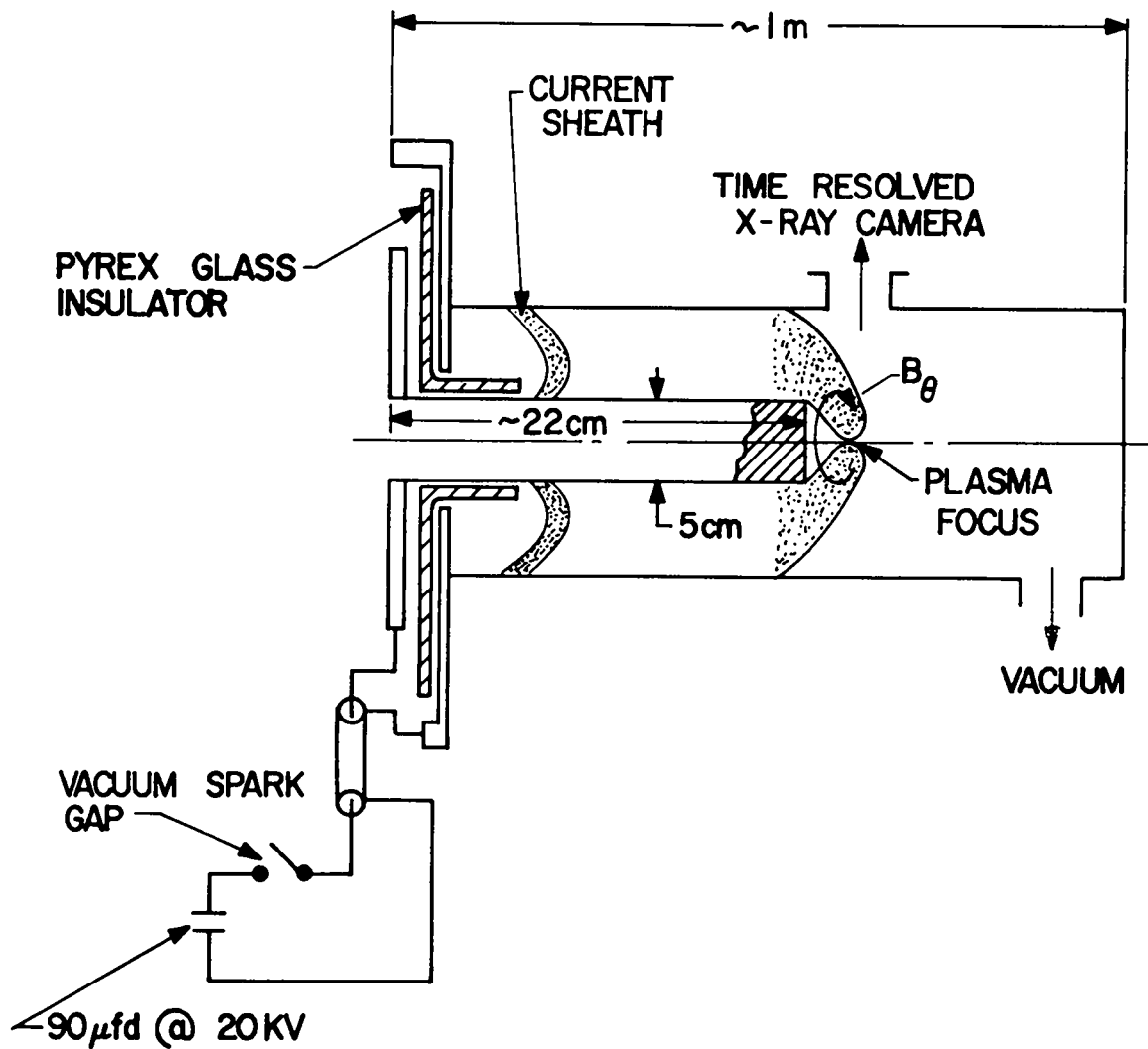
Fig. 1. Schematic of the discharge apparatus showing approximately the shape of the current sheath during the formative stages of the plasma focus.
