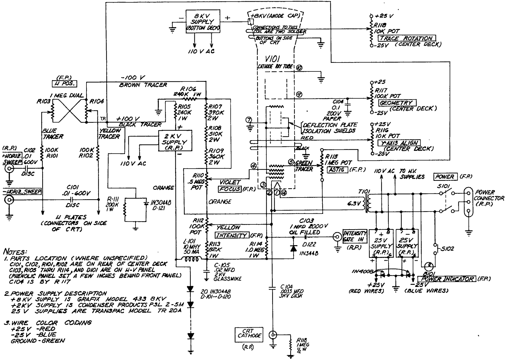
Fig. 21. Oscilloscope module designed for streak recording, less signal preamplifiers.
