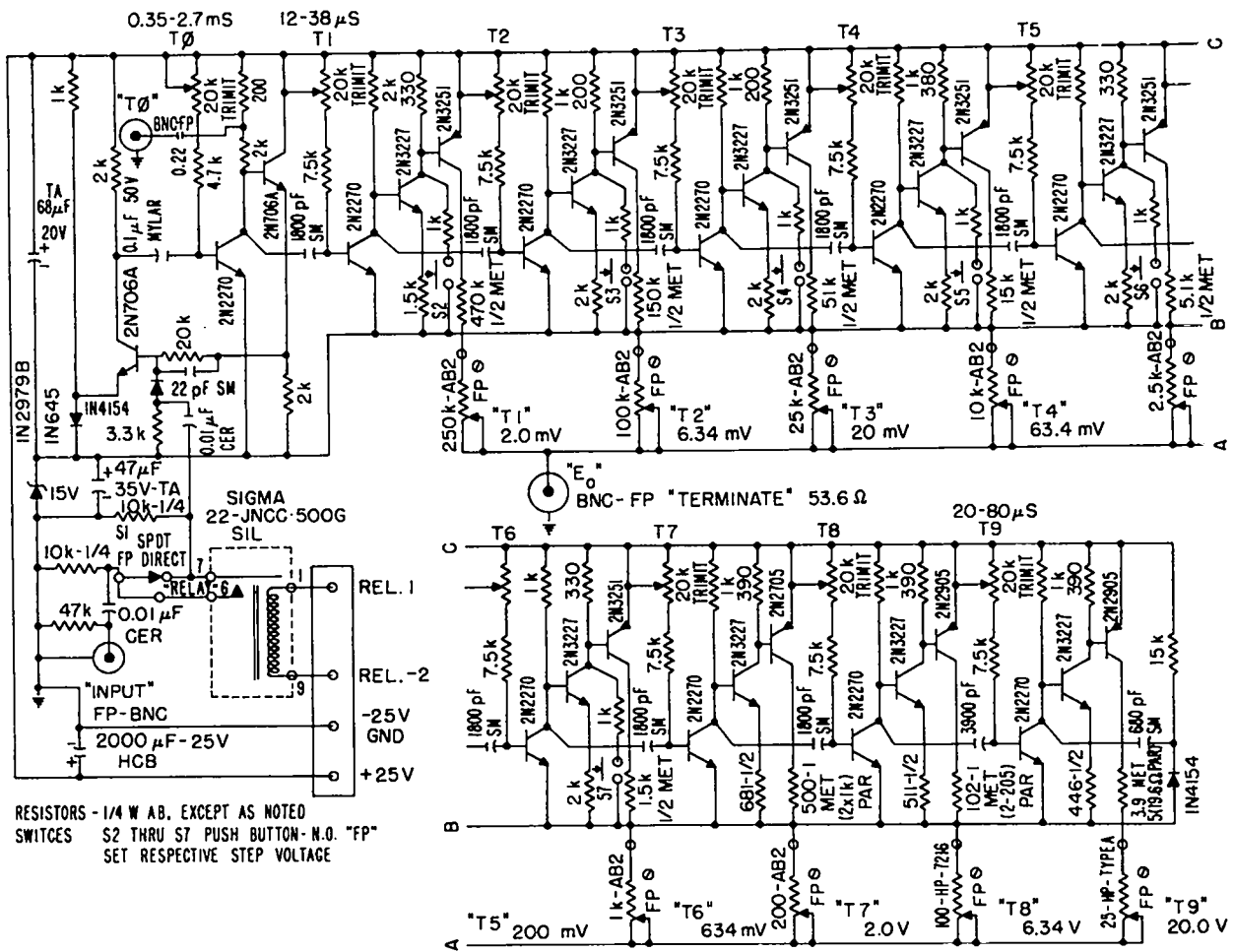
Fig. 15. LASL Model 3A stair-step calibrator.
