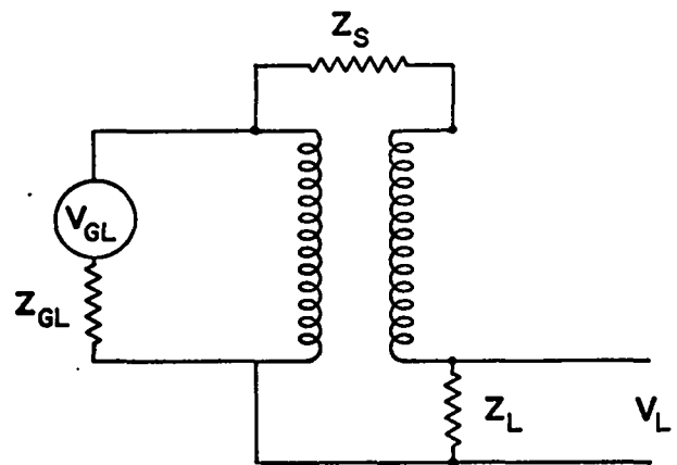
Fig. 19. Reconstruction of a coaxial cable as a 1:1 transformer.
