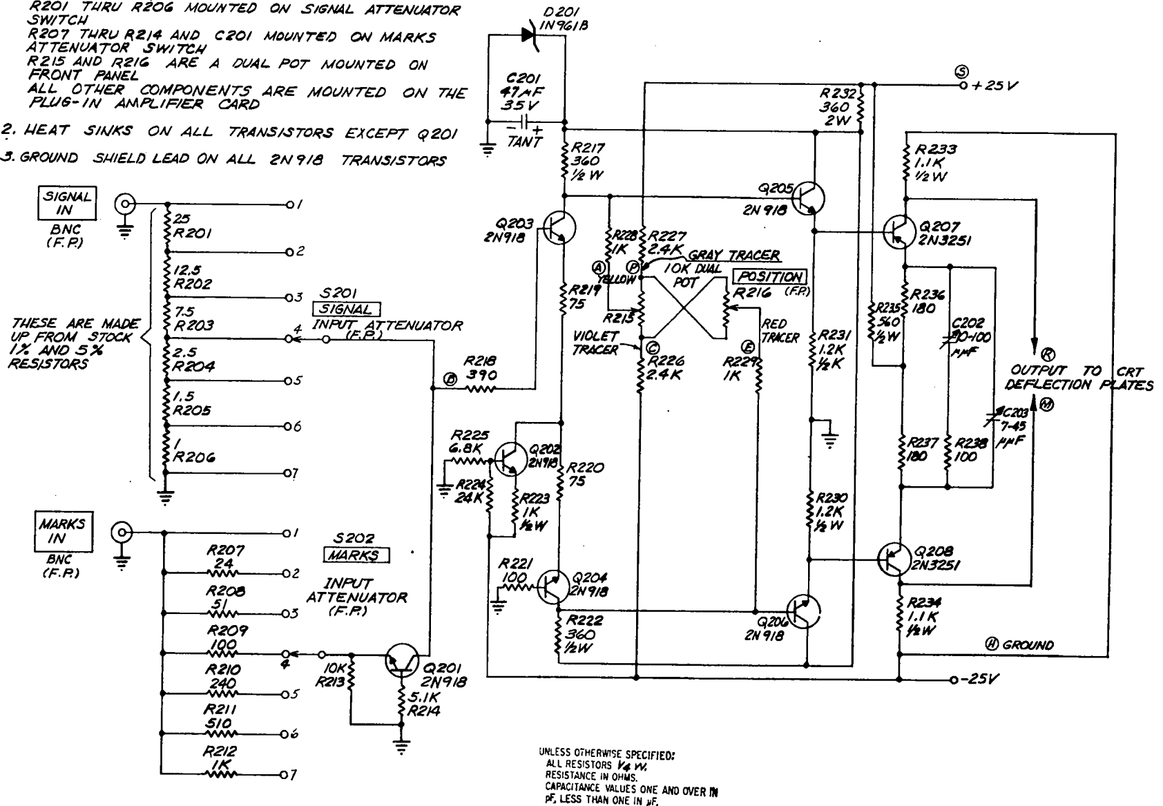
Fig. 22. Oscilloscope module designed for streak recording, signal preamplifiers only.
