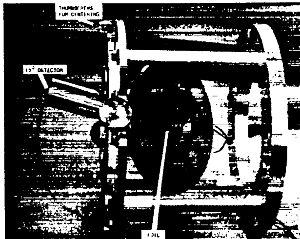
Fig. 7. Module for mounting one foil and its detectors.
