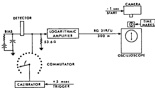
Fig. 10. Schematic showing one detector, log preamplifier, cable, calibrator, and recorder.
