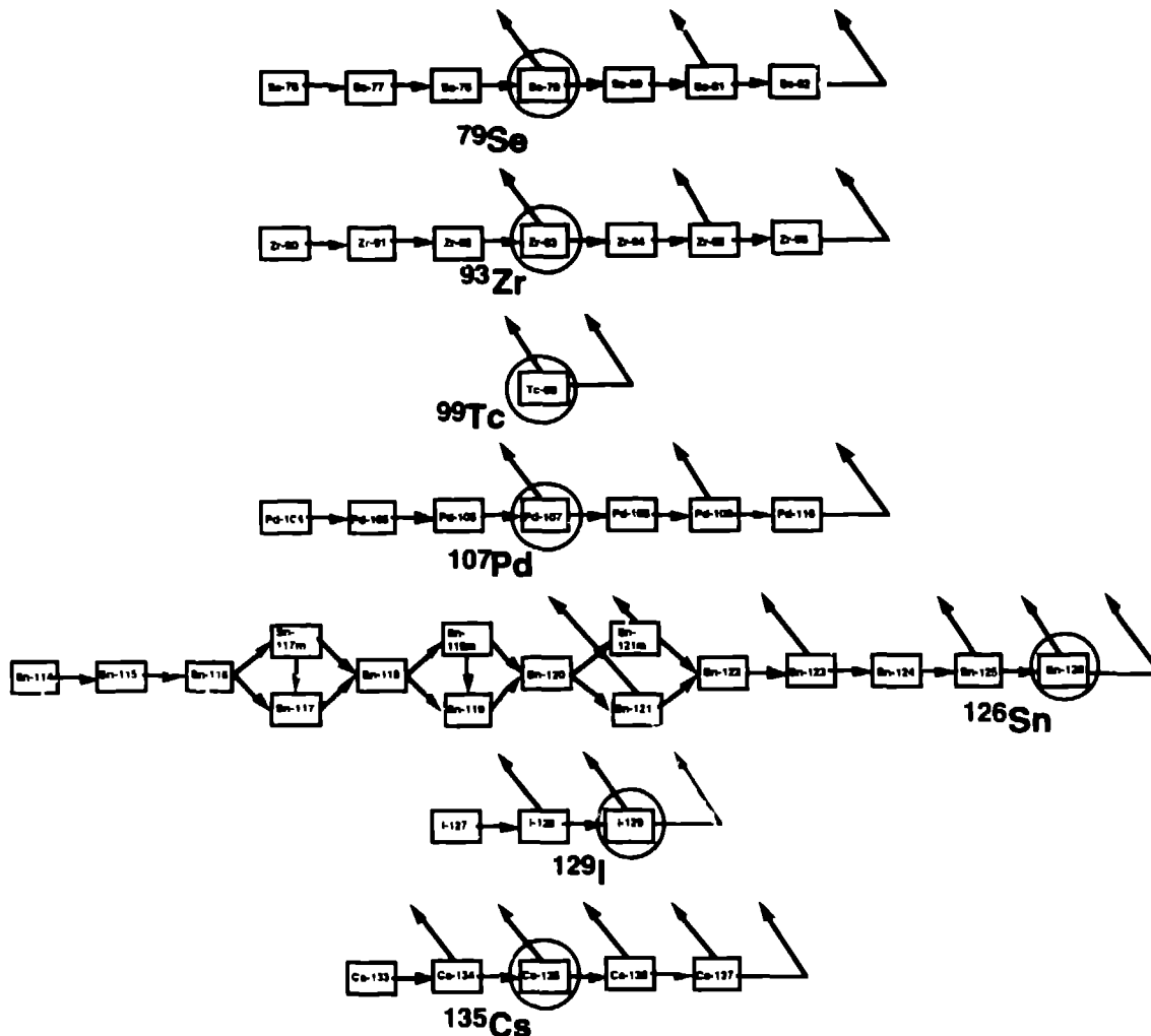
Figure 2. Long-Lived Fission Product Chains
