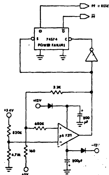
Fig. 7. Power failure detector. The 5.4V supply is battery operated and will never disappear. The negative going output from comparator occurs at a voltage of about 4.65V and sets power failure flip-flop that disables all the circuitry. When power returns, PF flip-flop will keep the circuits at reset until the voltage reaches about 4.9V.
