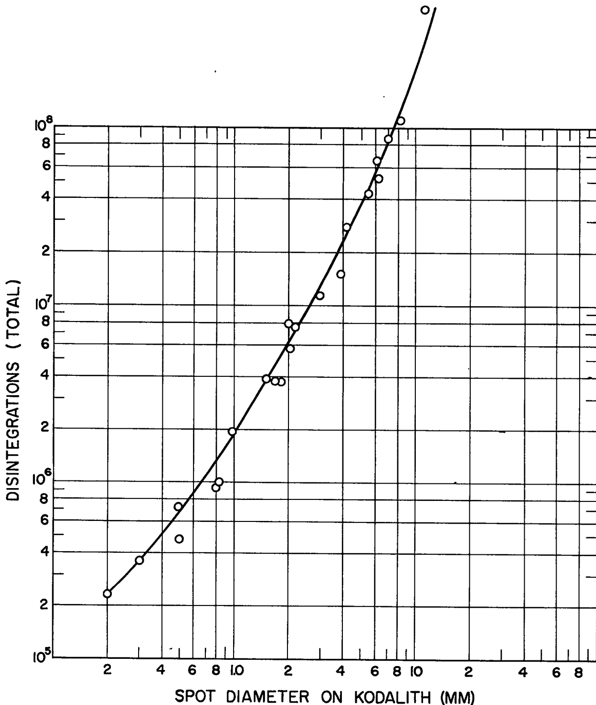
Fig. 9. Spot size on Kodalith film as a function of beta activity. (Ansco High Speed x-ray film).
