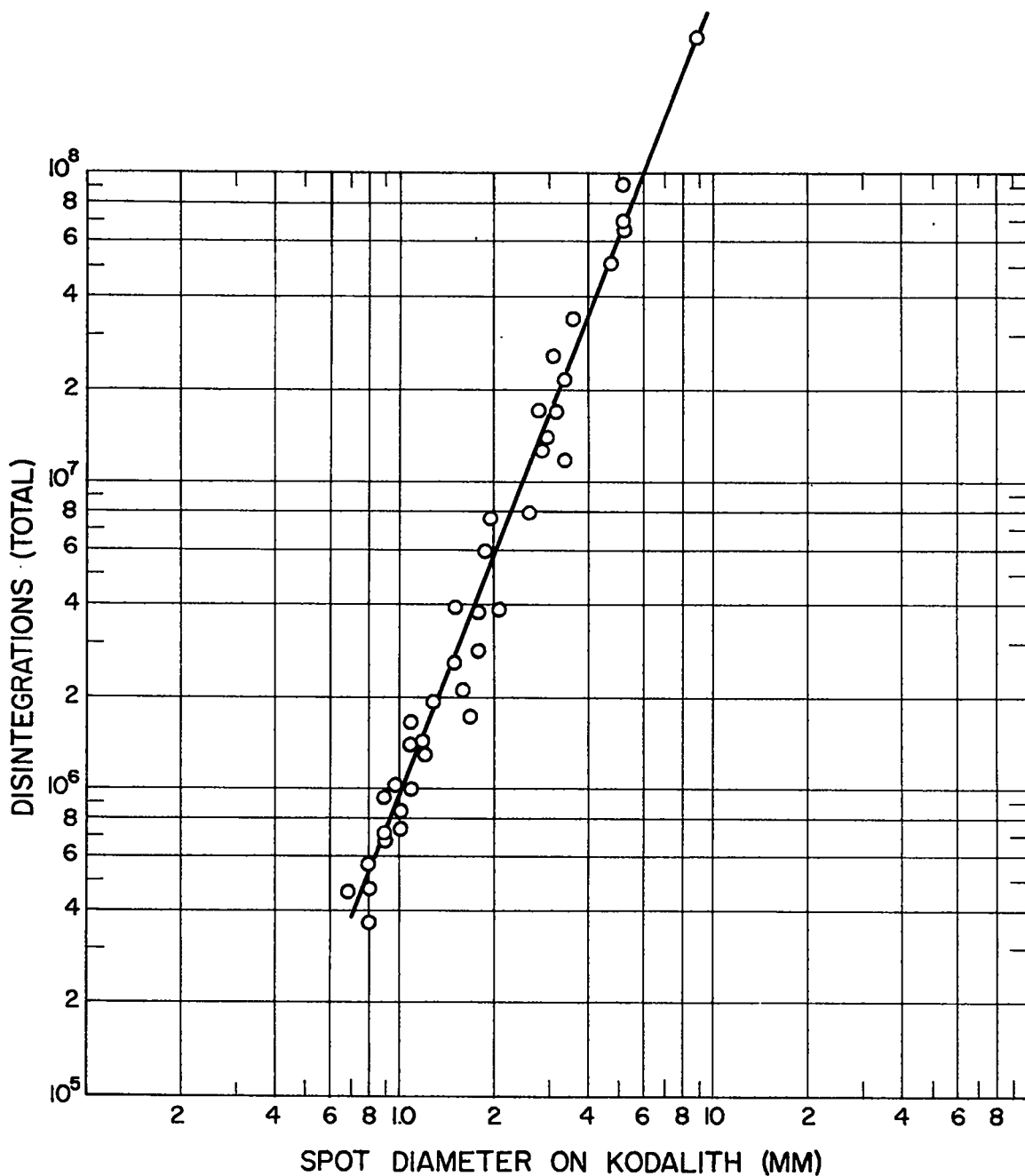
Fig. 11. Spot size on Kodalith film as a function of beta activity (Type-K x-ray film).
