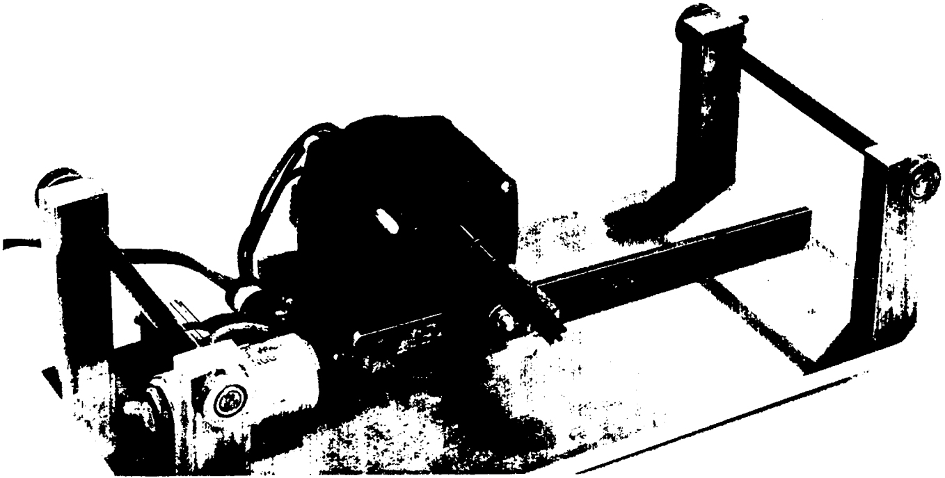
Fig. 3. Motor-driven carriage
