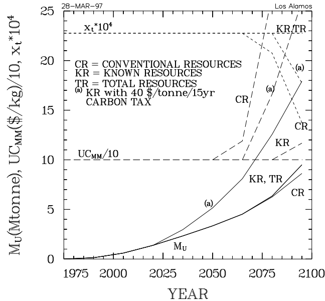
Figure 37. Uranium resource utilization, cost, and cost-optimum tailings concentrations 24,25 for the basis scenario under three assumptions of resource availability.
