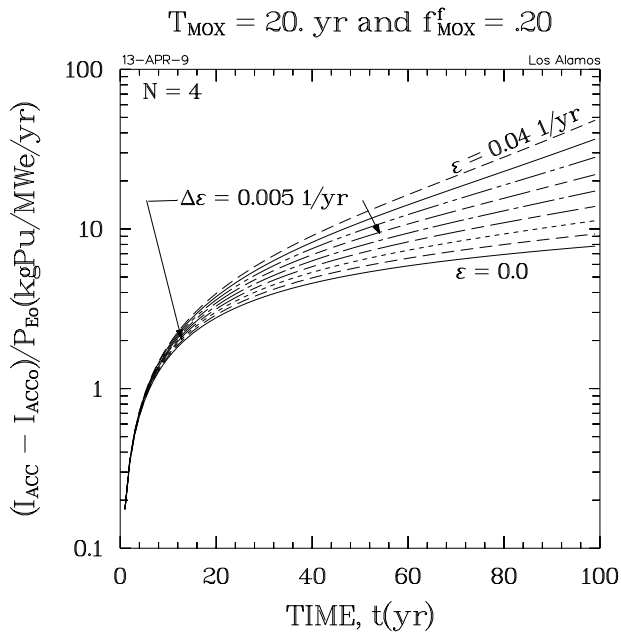
Figure A-3A. Time dependence of recyclable (to LWRs, ACC) plutonium inventories for a range of nuclear energy growth rates, \epsilon , and asymptotic MOX core fractions, f_{MOX}^f , for the parameters listed in Table A-I: f_{MOX}^f = 0.20
