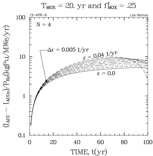
Figure A-3B. Time dependence of recyclable (to LWRs, ACC) plutonium inventories for a range of nuclear energy growth rates, \epsilon , and asymptotic MOX core fractions, f_{MOX}^f , for the parameters listed in Table A-I: f_{MOX}^f = 0.25
