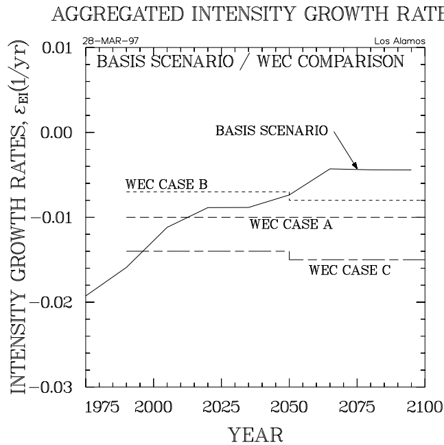
Figure 19. Comparison of rate of primary energy intensity decrease for the basis scenario with three WEC cases: 5,6 Case A = High Growth; Case B = Base Case; Case C = Ecologically Driven.
