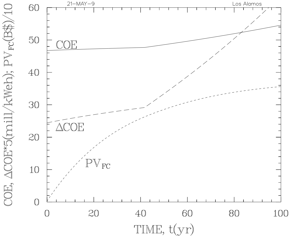
Figure 10. Time evolution of cost of electricity, COE(mill/kWeh), incremental COE related to the fuel cycle, \Delta\text{COE} (mill/kWeh), and present value of all fuel cycle charges evaluated over the time of the computation for a cost of money \text{COM} = 0.05 1/yr, for the OT/LWR case and uranium resources = KR (Fig. 5).
