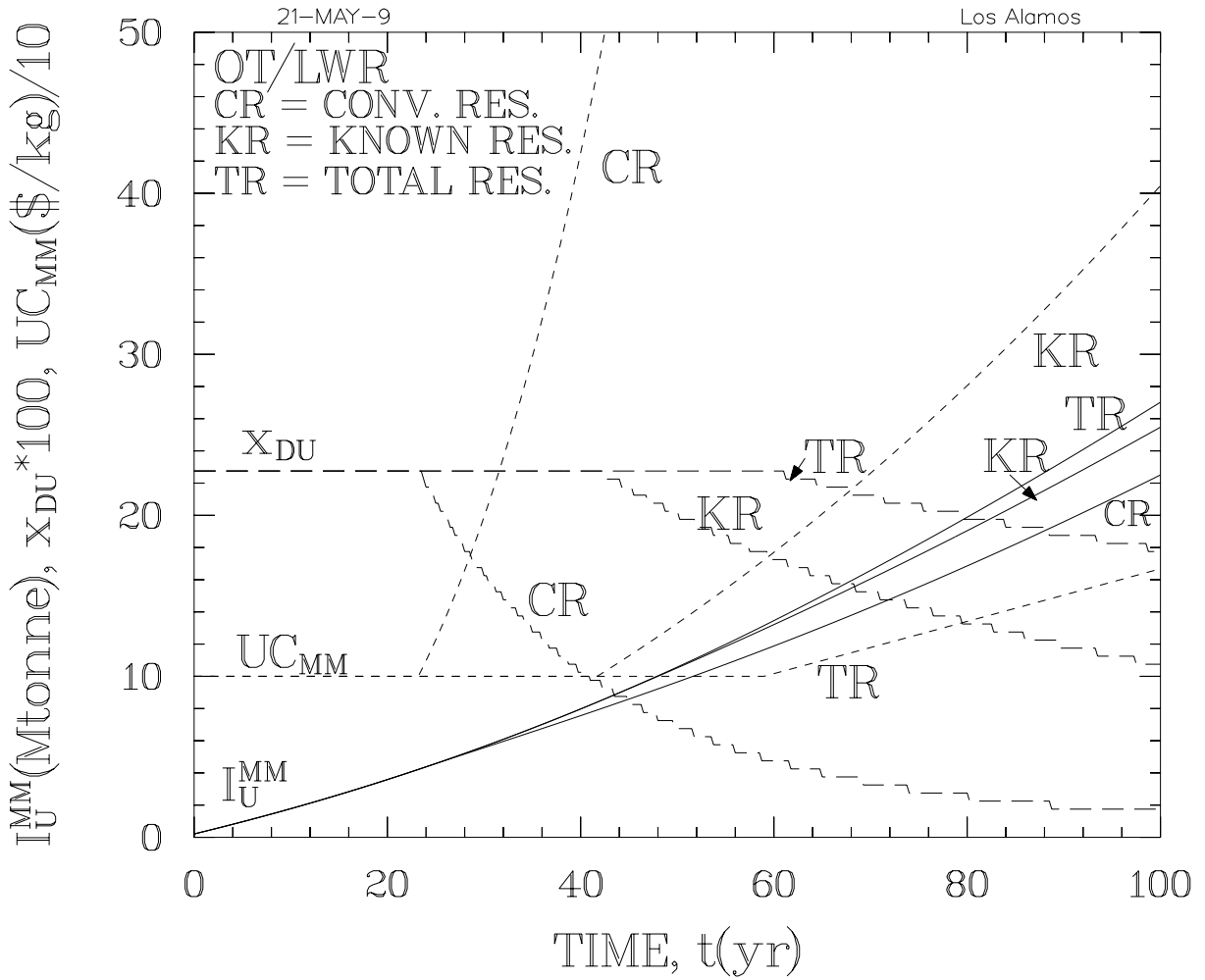
Figure 12. Cost impact of the range of uranium resource “realities” suggested on Fig. 5 for the OT/LWR case. Reflections of these uranium costs on COE and \Delta COE are given in comparison with the MOX/LWR case (Fig. 17).
