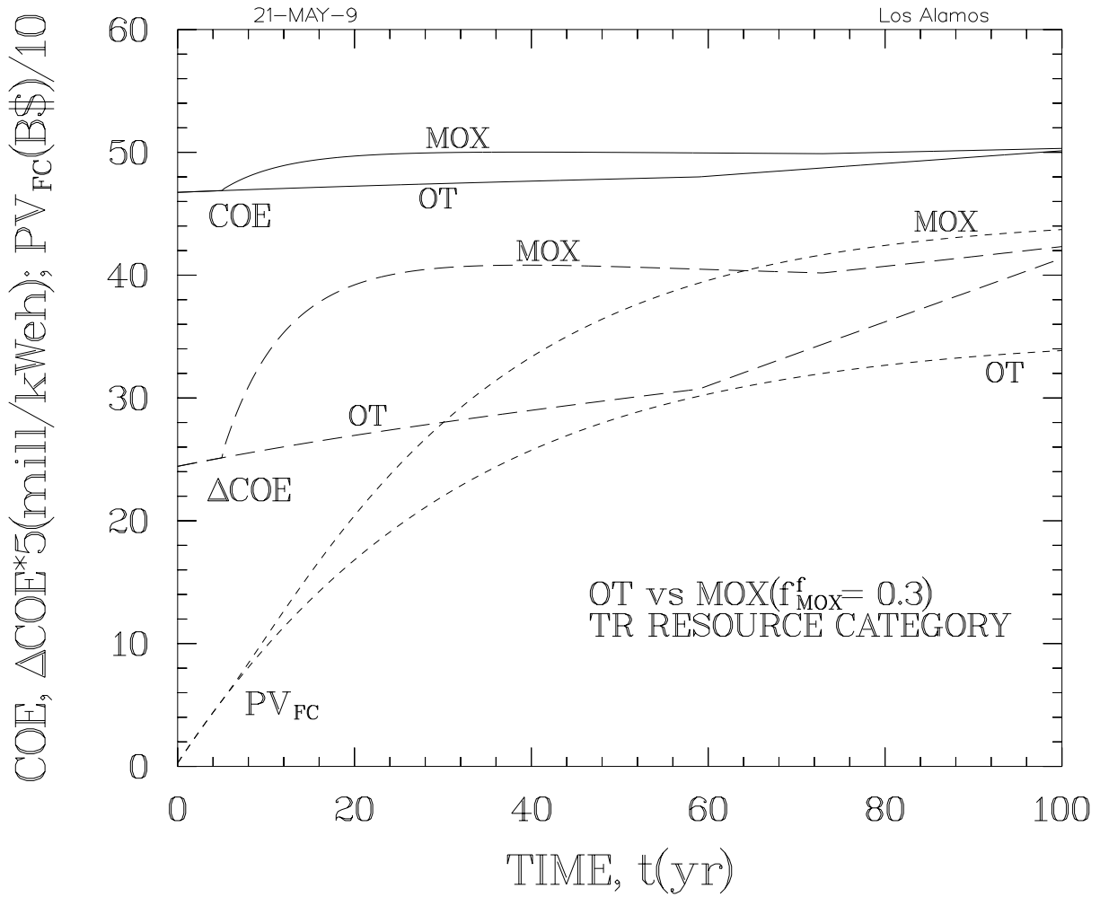
Figure 17C. Time evolution of cost of electricity, COE(mill/kWeh), incremental COE related to the fuel cycle, \Delta COE(mill/kWeh), and present value of all fuel cycle charges evaluated over the time of the computation for a cost of money COM = 0.05 1/yr, for the f_{MOX}^f = 0.3 MOX/LWR case and the TR category of uranium resources (Fig. 5).
