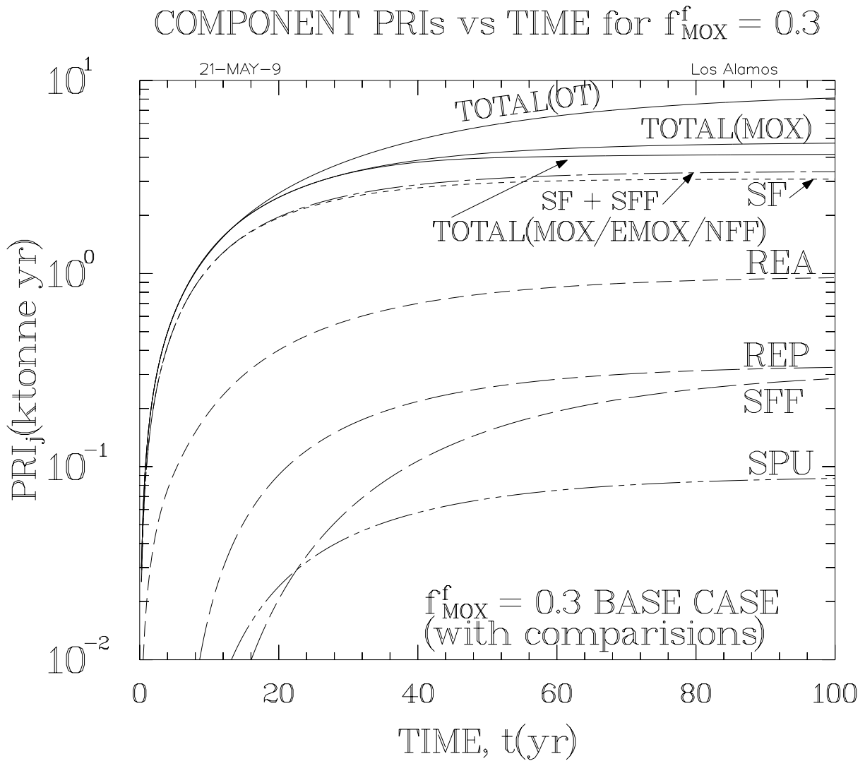
Figure 18. Time evolution of total and component proliferation risk indices, \text{PRI}(\text{ktonne yr}) , for the f_{\text{MOX}}^f = 0.3 MOX/LWR case that discounts risk at a rate r = 0.05 \text{ 1/yr} using the weights listed in Tables I and II. A comparison of the total PRI for the OT/LWR case reported on Fig. 11, as well as for a MOX/EMOX/NFF scenario reported in Sec. III.B.4, is given.
