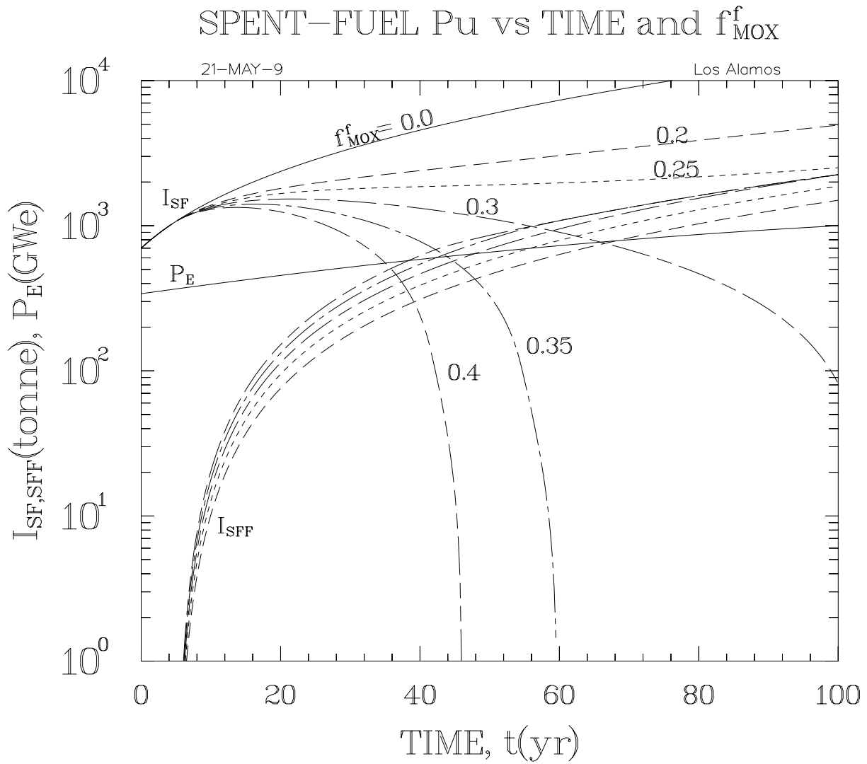
Figure 23A. Time dependence of key plutonium inventories for a range of asymptotic values of MOX core volume fraction for the cases depicted on Fig. 21; the OT/LWR case is designated by f_{MOX}^f = 0.0 ; SF = LWR-recyclable and SFF = LWR-unusable plutonium in spent fuel.
