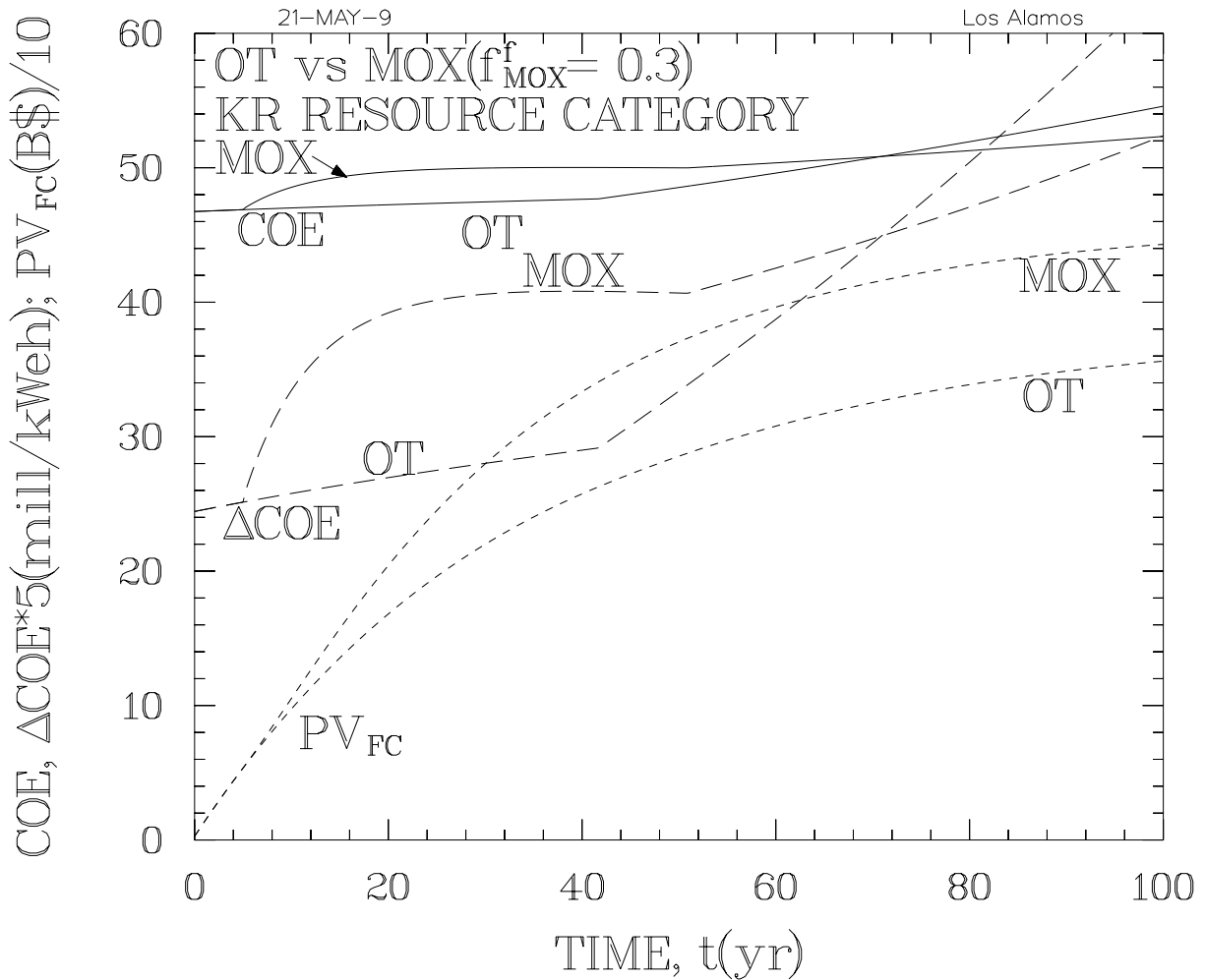
Figure 17B. Time evolution of cost of electricity, COE(mill/kWeh), incremental COE related to the fuel cycle, \Delta\text{COE} (mill/kWeh), and present value of all fuel cycle charges evaluated over the time of the computation for a cost of money \text{COM} = 0.05 1/yr, for the f_{\text{MOX}}^f = 0.3 MOX/LWR case and the KR category of uranium resources (Fig. 5).
