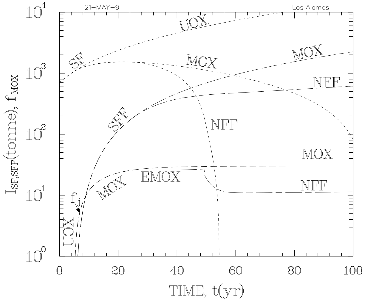
Figure 24A. Time dependence of key plutonium inventories for three fuel-cycle variations depicted on Fig. 3: a) OT/LWR (designated here as UOX); b) f_{MOX}^f = 0.3 MOX/LWR (base case); and c) UOX/EMOX/NFF (as depicted by the full scenario given in Fig. 3); SF = LWR recyclable and SFF = LWR-unusable plutonium in spent fuel.
