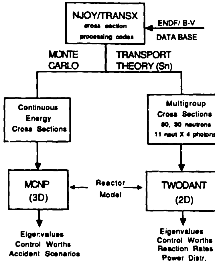
Fig. 8 Representative Calculational Methods
