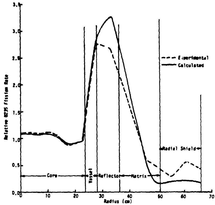
Fig. 11 Radial ^{235}\text{U} fission rate comparison
