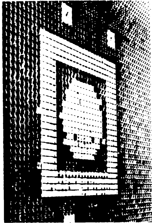
Fig. 2 - ZPPR-16A assembly loaded into matrix
