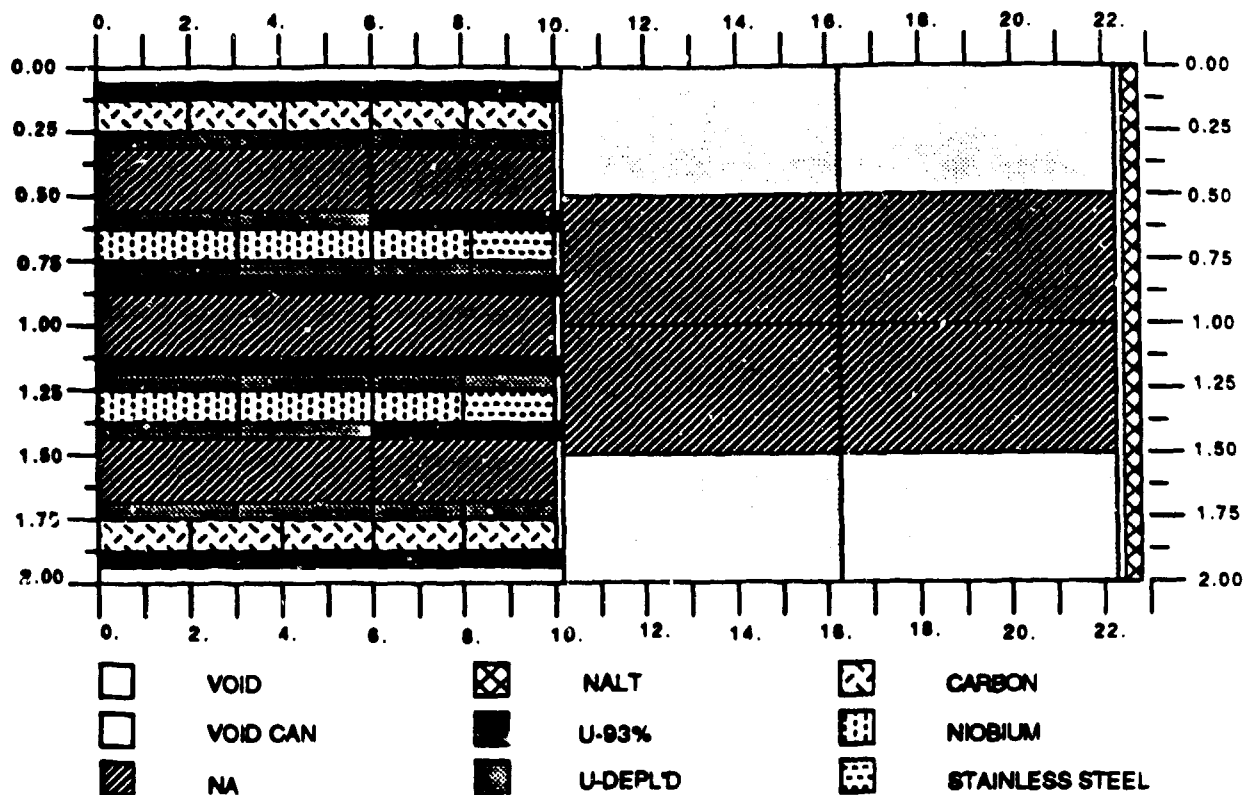
Fig. 4. Schematic of ZPPR-16B core drawer
