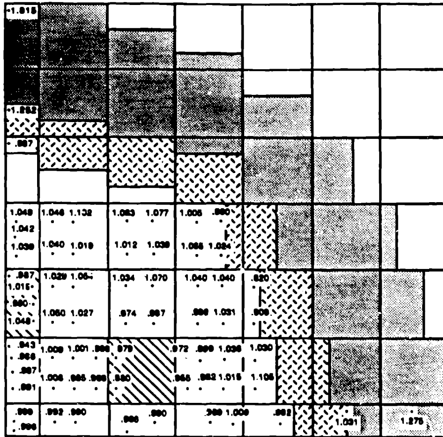
Fig. 10 Comparison of measured and calculated ^{235}\text{U} fission rates (16 mesh per drawer).
