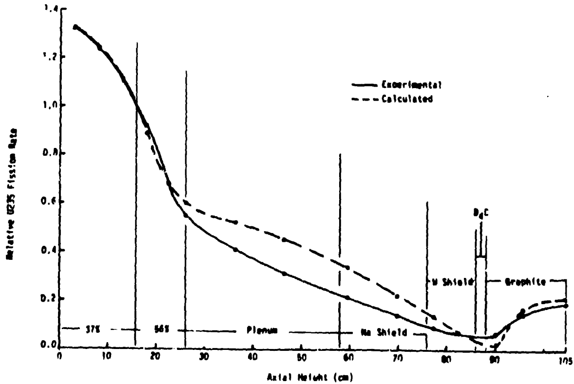
Fig. 12 Axial fission rate comparison for ^{235}\text{U} in central fuel drawer
