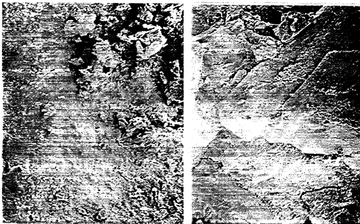
Figure 6. (Left) Weathered PBX 9404 (Specimen #1W, 1,000 \times ). (Right) PBX 9404 fresh cut from weathered piece (Specimen #1F, 1,000 \times ).
