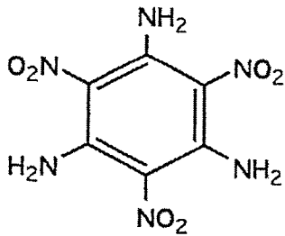
TATB FW = 258.1
