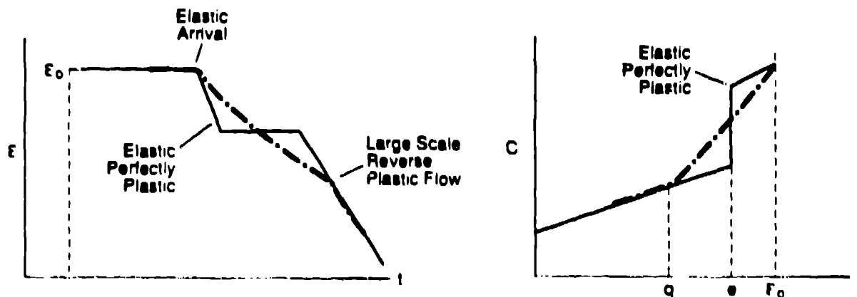
Fig. 1.- Anelastic release-wave profile.
