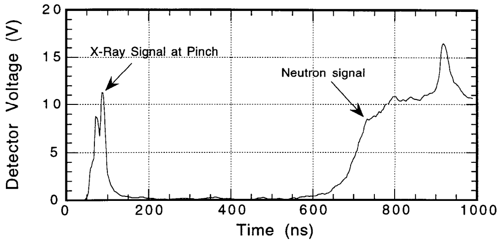
Figure 8 The signal from the scintillator/Photomultiplier tube diagnostic on Saturn Shot 1020 showing a hard x-ray signal at pinch time, the neutron-generated signal, and the late time scatter from the walls.
