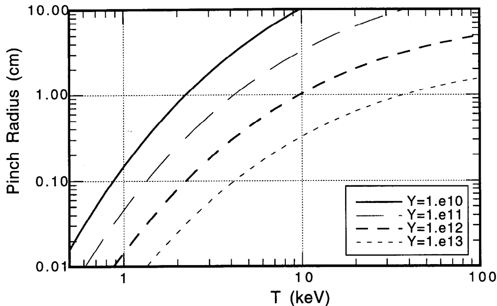
Figure 11 A plot showing the relationship between the final pinch radius, plasma temperature and the neutron yield..
