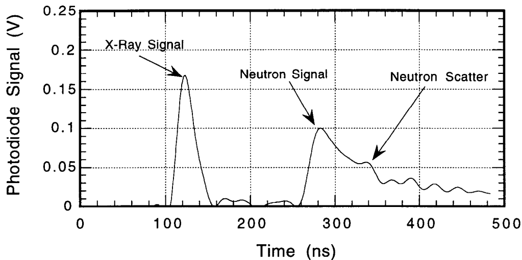
Figure 9 The signal from the photodiode on Saturn Shot 1020 showing a hard x-ray signal the neutron-generated signal and the late time scatter from the near by hardware.
