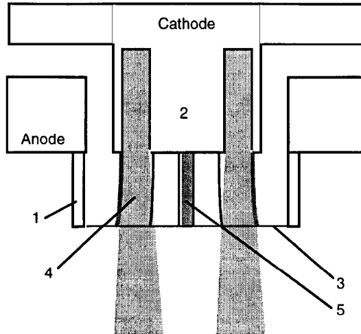
Figure 1 A schematic of the deuterium gas-puff z-pinch load configuration showing the anode and cathode electrodes, the anode current return posts (1), the supersonic gas nozzle (2), the current return wires (3), the initial position of the injected gas (4), and the final pinch (5).
