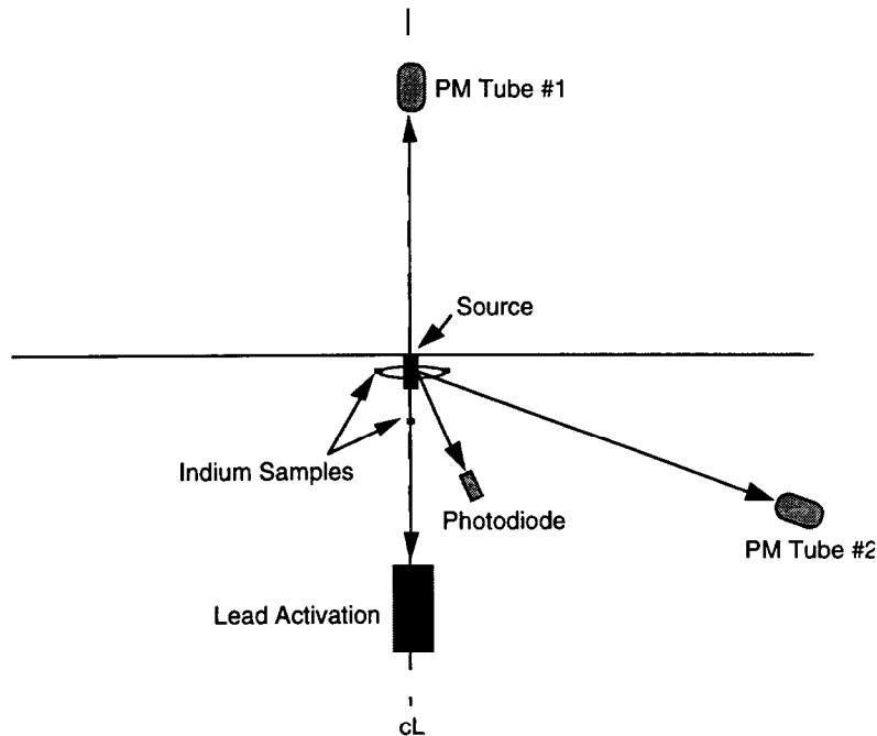
Figure 2 A schematic of the neutron diagnostics fielded on Saturn for the D-D fusion experiments showing their relative orientation. The figure indicates the relative orientation of the neutron diagnostics.
