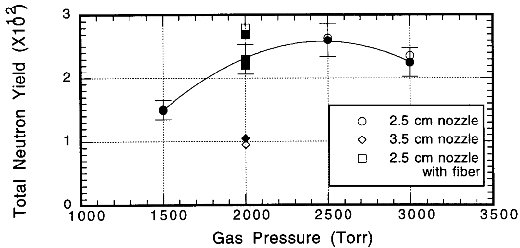
Figure 6 Data from the D-D neutron shots on Saturn for the different plasma conditions of the experiments. Solid points are scaled PM tube data while open circles are yields from the indium activation detector.
