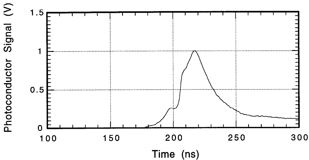
Figure 7 The signal from a gallium-arsenide PCD filtered with 254 \mu\text{m} of Kapton. The signal amplitude is related directly to the electron temperature.
