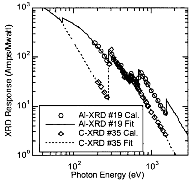
Figure 12. Typical calibration data and fits to the data for an aluminum and carbon photocathode.
