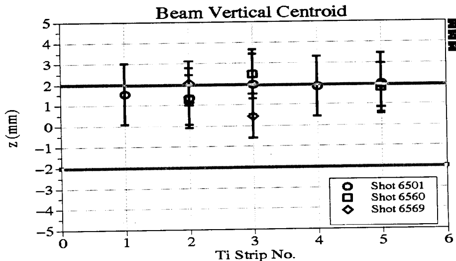
Figure 4. Vertical centroid focus position from three target shots. The target midplane is at z=0 and extends to +/- 2 mm.
