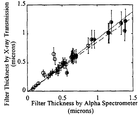
Figure 3. Comparison of selected filter thickness measurements from alpha spectrometer and x-ray transmission. Thick filters and filter designs with consistently high errors have been omitted.
