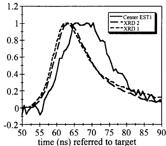
Figure 9. Time history of two XRD traces and the emission from the center of the target as obtained with the EST diagnostic. The FWHM_{center} = 17 \pm 4 ns and the FWHM_{XRD} = 13 \pm 2 ns.
