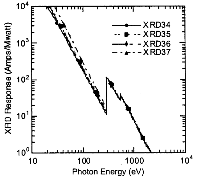
Figure 14. Responses for the carbon photocathodes.
