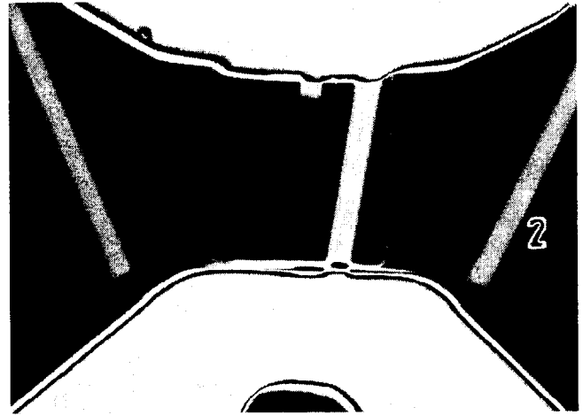
Figure 6. Technique used to image the distance from the strips to the gold foil: 35 kV, 500 \mu A, 165-second exposure time; source-to-object distance: 2-1/8"; source-to-film: 27". A hard cassette was used with Kodak AA film sandwiched between .001" of lead foil with 0.010" of lead screen behind the foil to reduce scatter.
