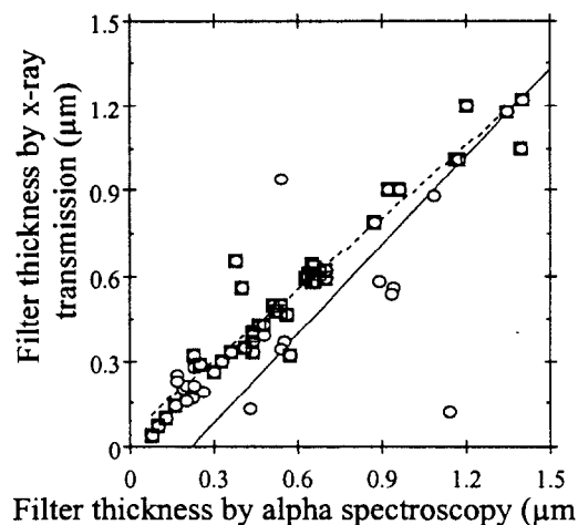
Figure 2. Comparison of filter thickness from alpha spectrometer and x-ray transmission measurements. This graphs shows only those filters up to 1.5 \mu\text{m} thickness. The solid line is a linear fit of all data points shown in Figure 1 (circles). The dashed line is a fit to the "selected," or consistent filters (squares).
