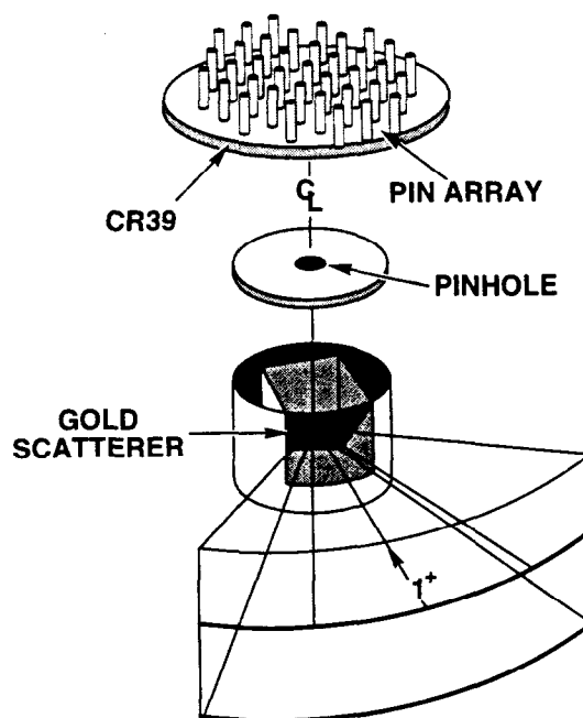
Figure 7. Artist's conception of the ion movie camera.
