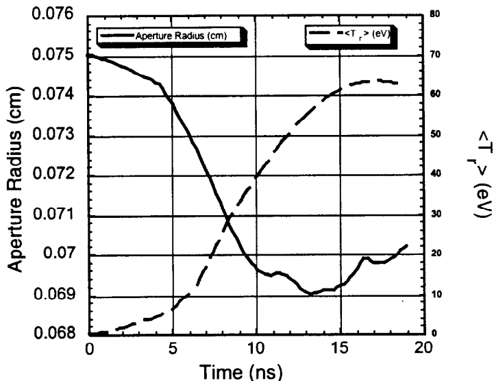
Figure 6. The aperture radius reaches a minimum (at 13.3 ns) before peak hohlraum wall temperature (at 17.2 ns).
