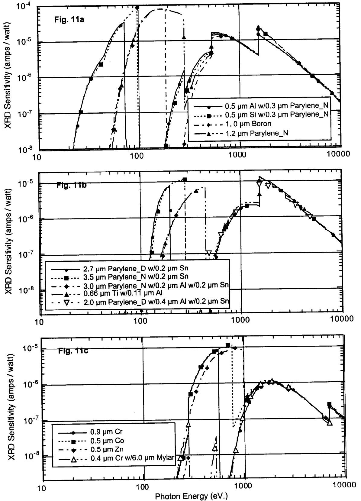
Figure 11a-c. Nominal XRD sensitivities used.
