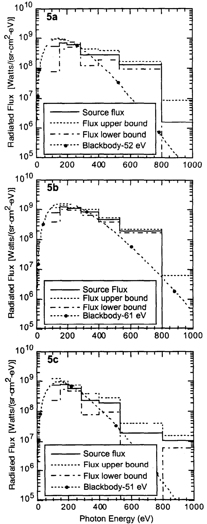
Figure 5a. The unfolded spectrum from shot 6517 at 10.5 ns, (5b) 14.5 ns, and (5c) 22.5 ns into the power pulse.
