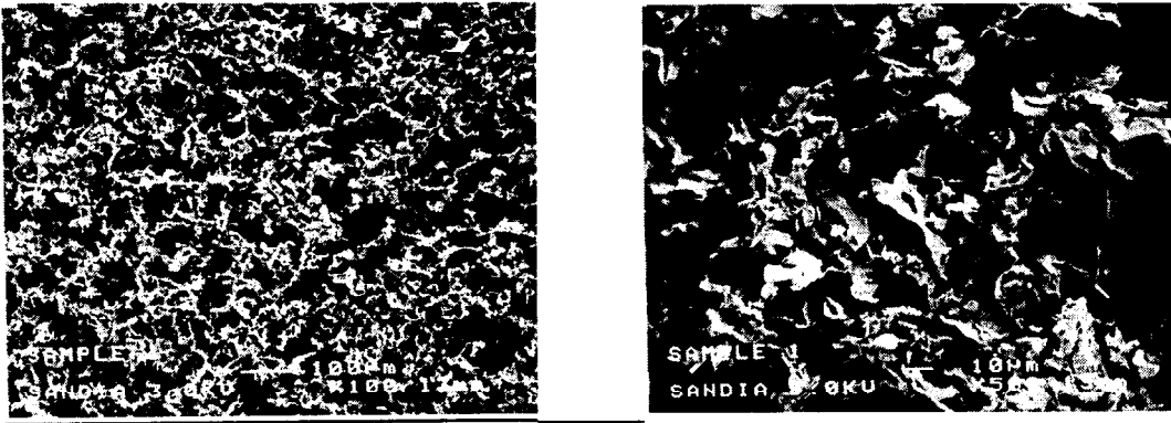
Figure 5. Scanning electron photomicrographs of nominal 5\text{mg}/\text{cm}^3 TPX foam.
