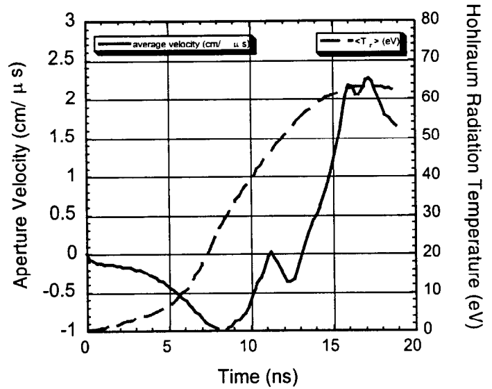
Figure 7. The aperture initially closes with a maximum velocity of -1.0 \text{ cm}/\mu\text{s} and then begins to re-open as the hohlraum temperature rises.
