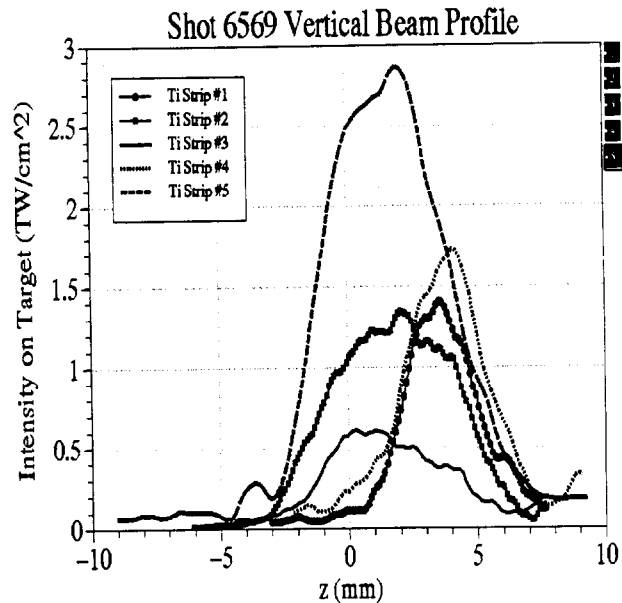
Figure 3. Vertical beam profiles from shot #6569. Strips #1 and #4 are shortened and thus only view the beam above the target. The target midplane is at z=0.
