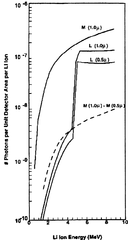
Figure 4. L- and M-shell yields for Li ions on Au cones of thickness 0.5 m and 1.0 m. Because the cone is optically thick for the M-shell, there is only a small difference in doubling the foil thickness; thus I show the difference in M-shell yield with foil thickness.
