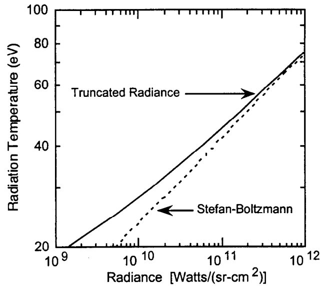
Figure 4. Characteristic temperature as a function of the integral of the differential energy spectrum for emitted flux as given by the Stefan-Boltzmann equation (dotted line) and the integral between 98.1 and 1200 eV (solid line).
