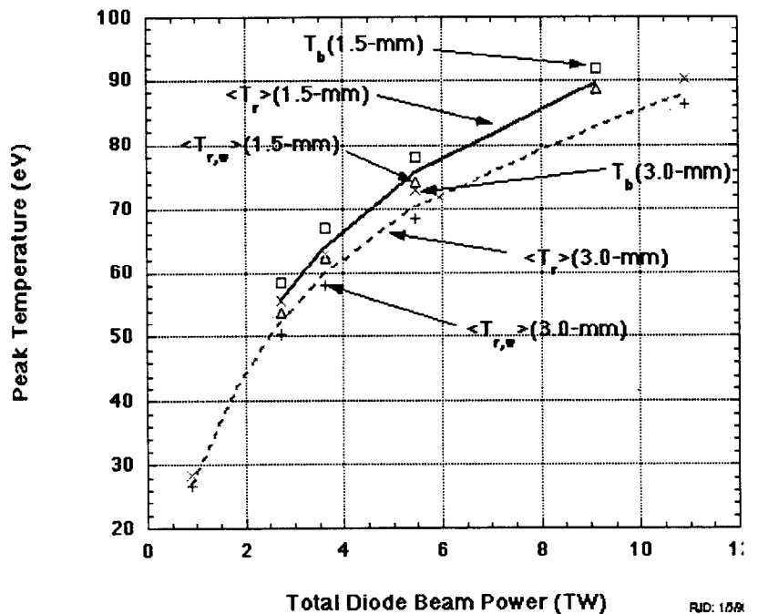
Figure 2. Hohltraum temperature scaling with total ion beam power.
