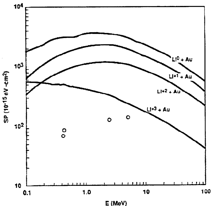
Figure 2. Comparison of calculated SP for Li on gold with the measurements of Teplova et al. 4 (open circles).
