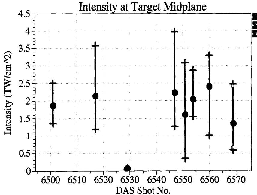
Figure 6. The range of absolute intensity for each shot is shown along the target midplane. Circles show the mean intensity; the crosses show the maximum and minimum intensities measured.
