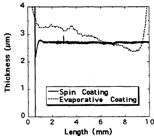
Figure 1. Comparison of film thicknesses of evaporatively coated and spin coated films of Pilot U.
