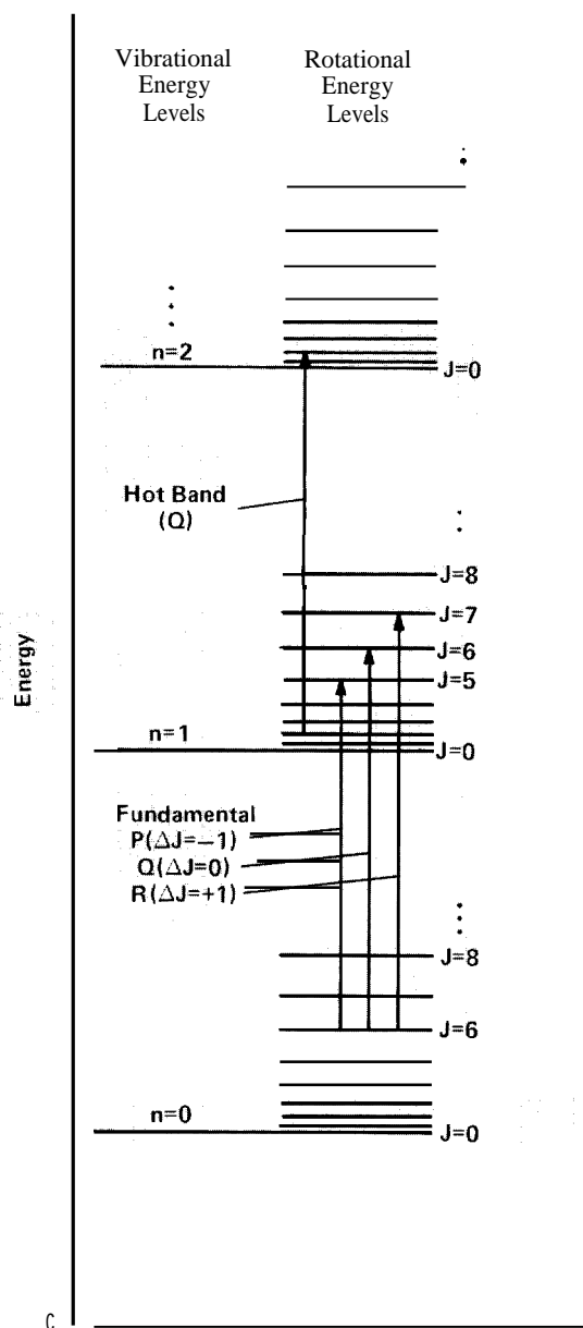
Fig. 5. Rotational-vibrational energy transitions. For a harmonic normal-mode vibration, the energy levels are equally spaced; these are represented here by the quantum number n with only the three lowest levels shown. The ground vibrational energy level ( n = 0 ) is not at zero energy because the Heisenberg uncertainty principle requires an oscillator never to be completely at rest. The rotational energy levels are represented by the total angular momentum quantum number J and have spacings that increase quadratically with J . Thus the frequency of a given energy transition depends on both the J of the starting level and the simultaneous change in rotational energy. Examples of allowed transitions out of the vibrational ground state ( n = 0 ) are shown. The conventional designation is P(J) , Q(J) , or R(J) , depending on the value of \Delta J , plus the value of J in the lower state; thus, the three transitions shown are P(6) , Q(6) , and R(6) . A single hot-band transition from n = 1 to n = 2 , Q(2) , is also shown. The relative spacings of the rotational and vibrational energy levels will depend on the bond strengths and the molecular moments of inertia; typically, the rotational energy levels are much more closely spaced than depicted here.
