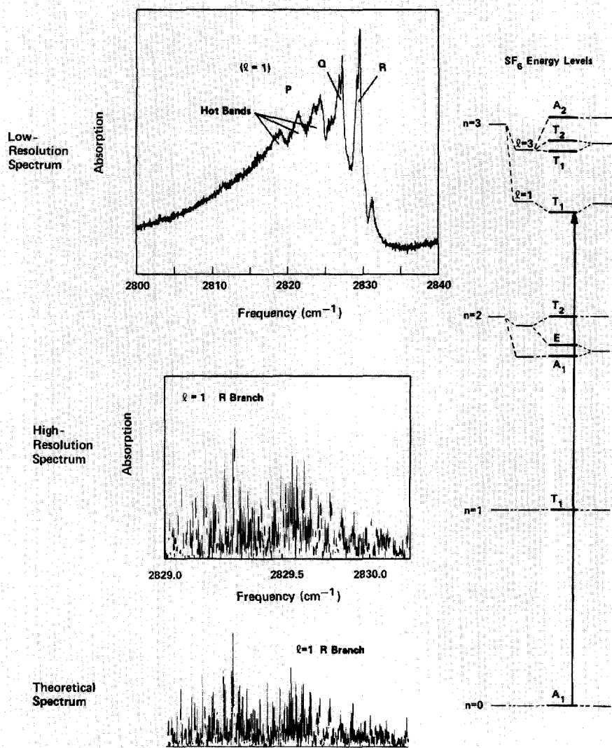
Fig. 11. The overtone 3\nu_3 of SF_6 . The upper spectrum was obtained with a Fourier-transform infrared interferometer at a resolution of 0.04\text{ cm}^{-1} . The middle spectrum is a Doppler-limited scan recorded by A. S. Pine at the MIT Lincoln Laboratory using a difference frequency spectrometer. It shows the rotational fine structure of the R branch of the \ell = 1 transition; the vibrational energy transition corresponding to this spectrum is shown on the energy level diagram at the right. The bottom panel illustrates the match that is possible with a theoretical simulation of the spectrum.
