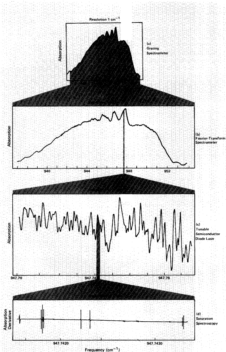
Fig. 2. Infrared spectra of the \nu_3 absorption of SF 6 at four resolutions. Spectrum (a) was recorded with a Fourier-transform infrared (FTIR) interferometer, but resolution was degraded to 1 cm -1 to match the spectrum produced by a typical commercial grating spectrometer. (b) An FTIR spectrum at a resolution of 0.06 cm -1 . (c) A Doppler-limited spectrum obtained by E. D. Hinkley at the MIT Lincoln Laboratory in 1970 using a tunable semiconductor diode laser. The effective resolution is the Doppler linewidth of 0.001 cm -1 . (d) Sub-Doppler saturation spectrum recorded by L. Henry at the University of Paris in 1976 with a resolution of better than 10 -6 cm -1 . All of the features in (d) occur inside the small range of frequency possible for the lasting of a single line of a CO 2 gas laser. The trace shows the first derivative of the absorption. Each absorption feature shown in (c) and (d) can be assigned to specific rotational-vibrational transitions of the SF 6 molecule.
