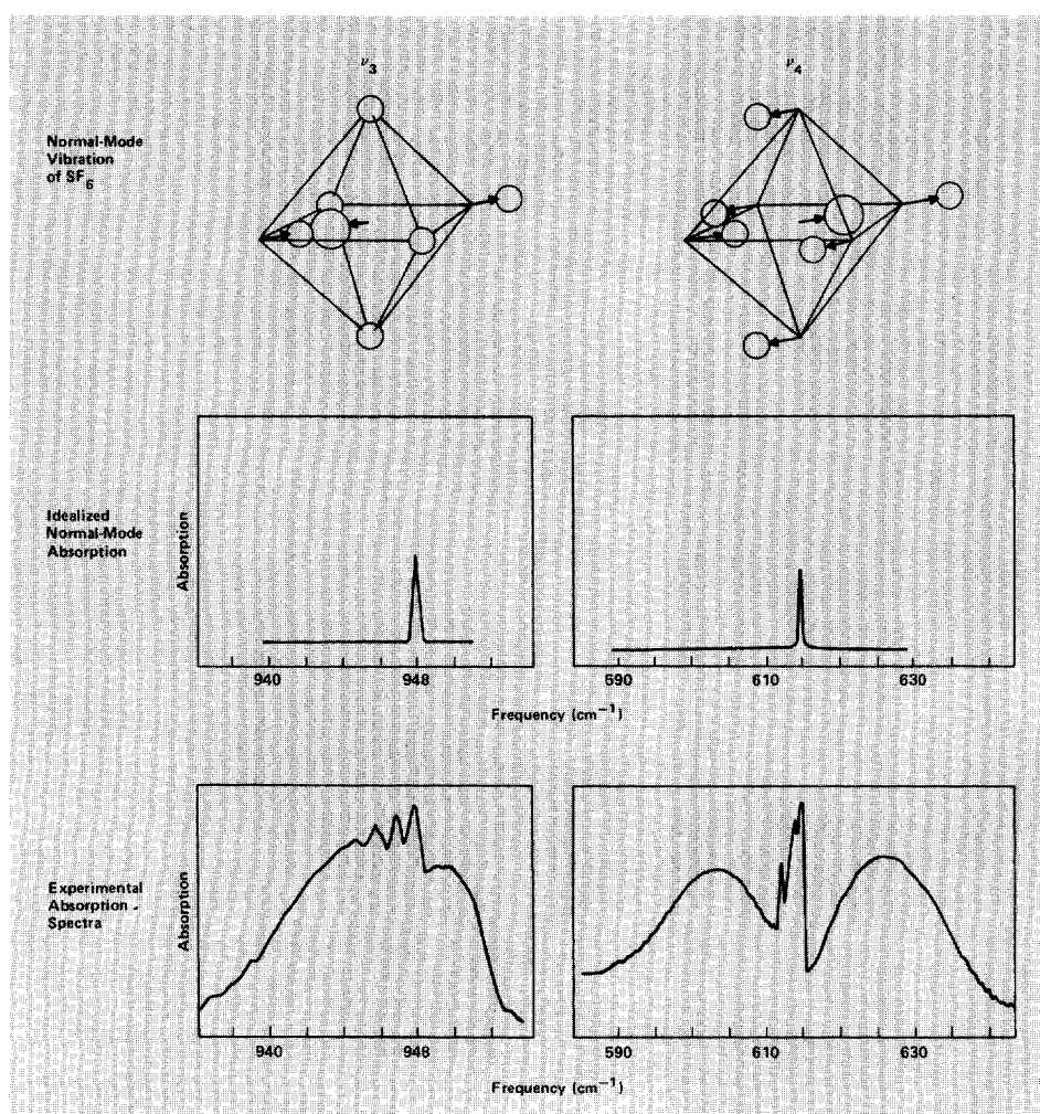
Fig. 1. The two infrared-active vibrations of SF_6 and associated spectra. The \nu_3 normal mode is principally an S-F bond stretching motion, whereas the \nu_4 mode is an F-S-F bending motion. If these vibrations were harmonic and no molecular rotation occurred, then the spectra would look like the graphs labeled Idealized Normal-Mode Absorption . Much of the width and structure seen in the Experimental Absorption Spectra are due to small rotational energy changes that accompany the large change in vibrational energy. (All spectra in this article have absorption increasing in the up direction.)
