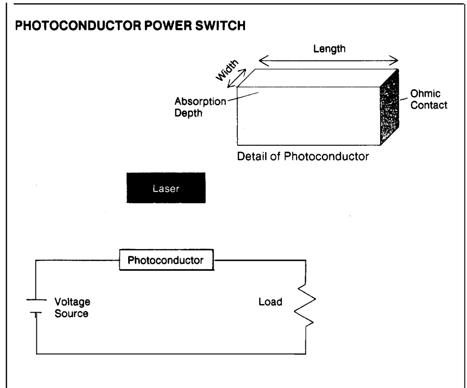
Fig. 2. A small volume of photoconductive material of relatively high intrinsic resistivity, a high-voltage source, and a pulsed laser are the basic components of a photoconductor power switch. When the photoconductive material is illuminated by a pulse of photons from the laser, its conductance rapidly increases and a short-rise-time current pulse flows through the load. In the absence of a laser pulse, the photoconductive material acts in effect as an open switch. The ohmic contacts to the
