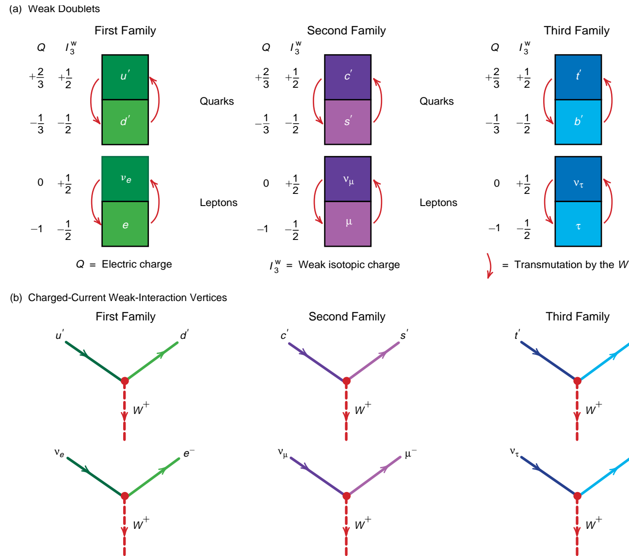
Figure 5. The “Weak” States—Particles Defined by the Local Symmetries of the Weak Force
