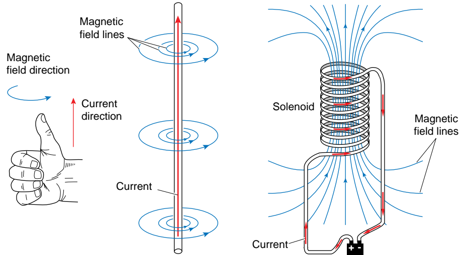
Figure 1. Magnetic Fields and Electrical Currents
