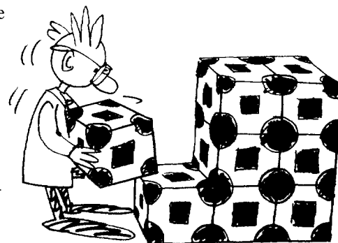
unit cell
