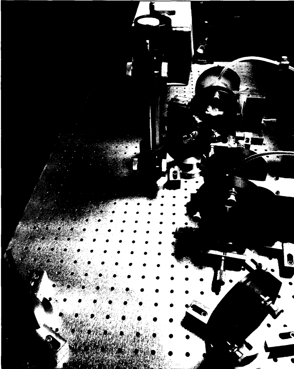
Photograph of the CPM laser built by the Laboratory's Electronic Research and Exploratory Development Group. The lasing medium (yellow) and the saturable absorber (purple) circulate through the tubes at the right, the pump laser is visible at the top, and the output coupling mirror is in the far background.
